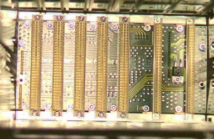
Backplane Board (Foil Side)
