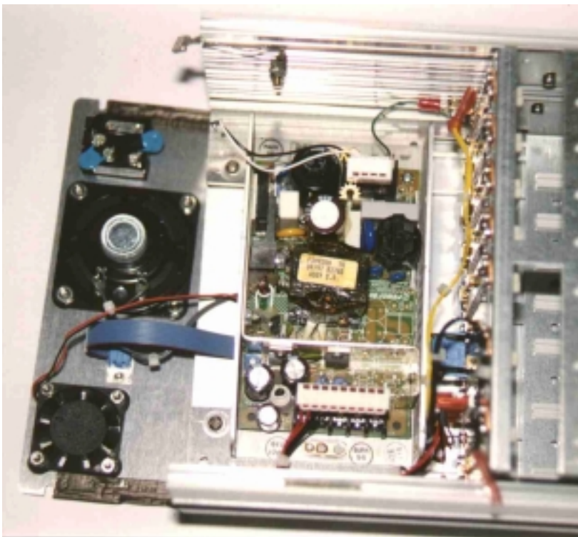
Power Supply Module Installed in Housing
