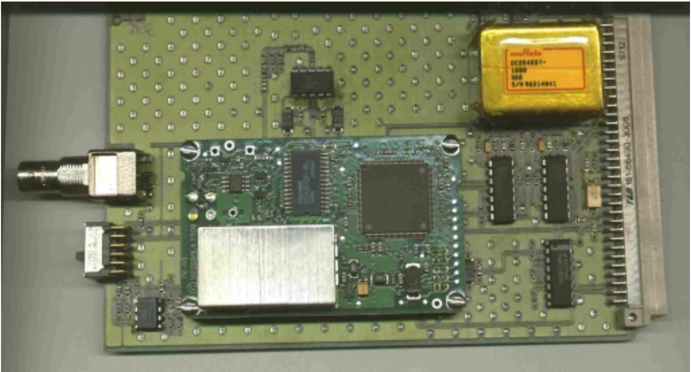
GPS-OSC Board Assembled
