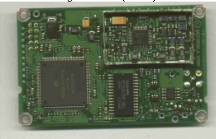
GPS-OSC Daughter Board (Side 2)
