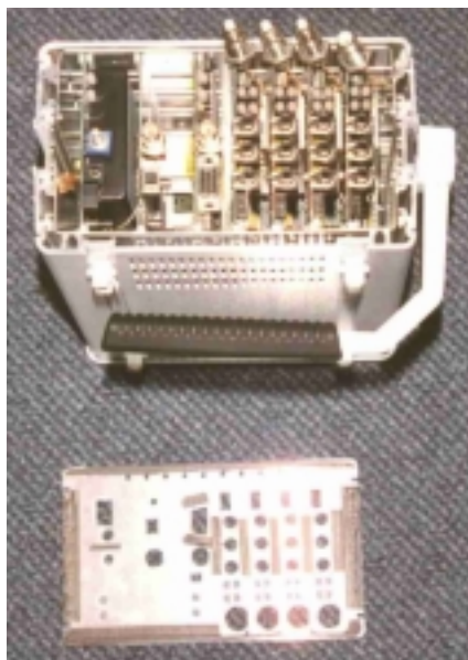
Top Cover Open
