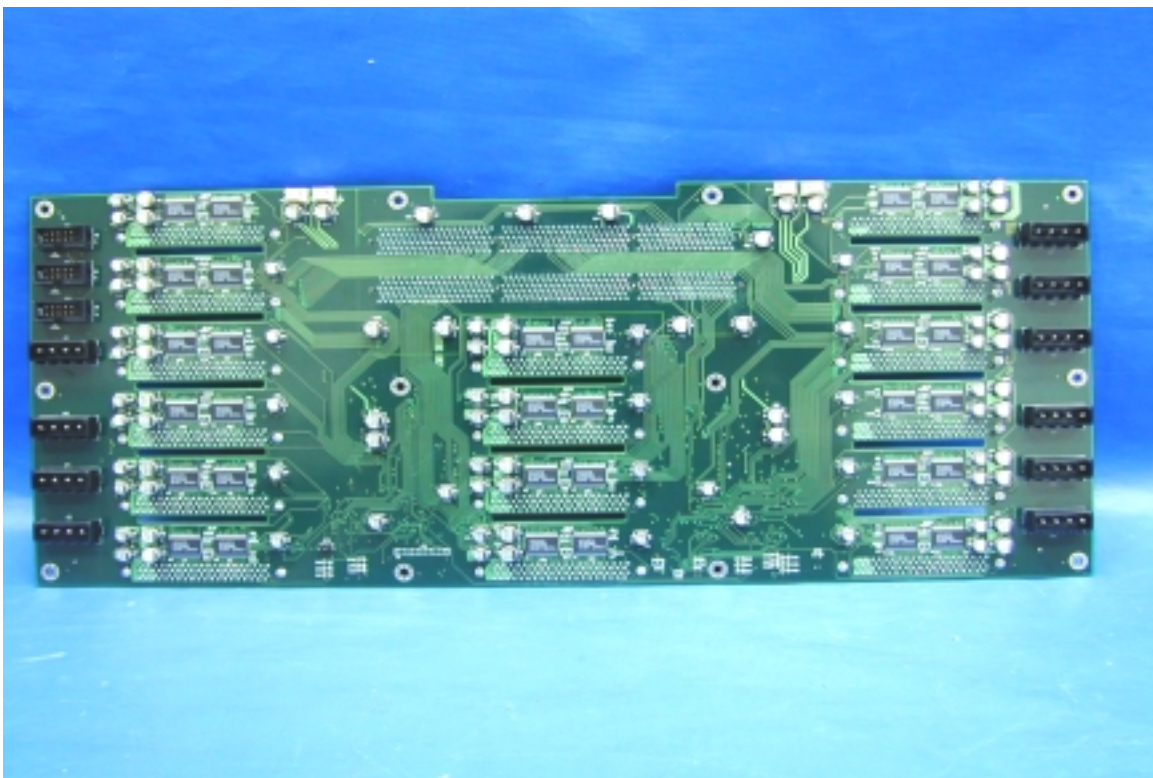
PHOTO. 20. EUT SOLDERING SIDE VIEW
