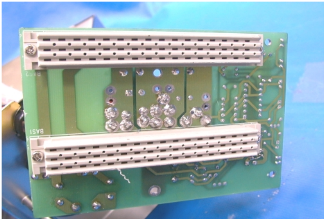
PHOTO. 18. POWER SUPPLY SOLDERING SIDE VIEW
