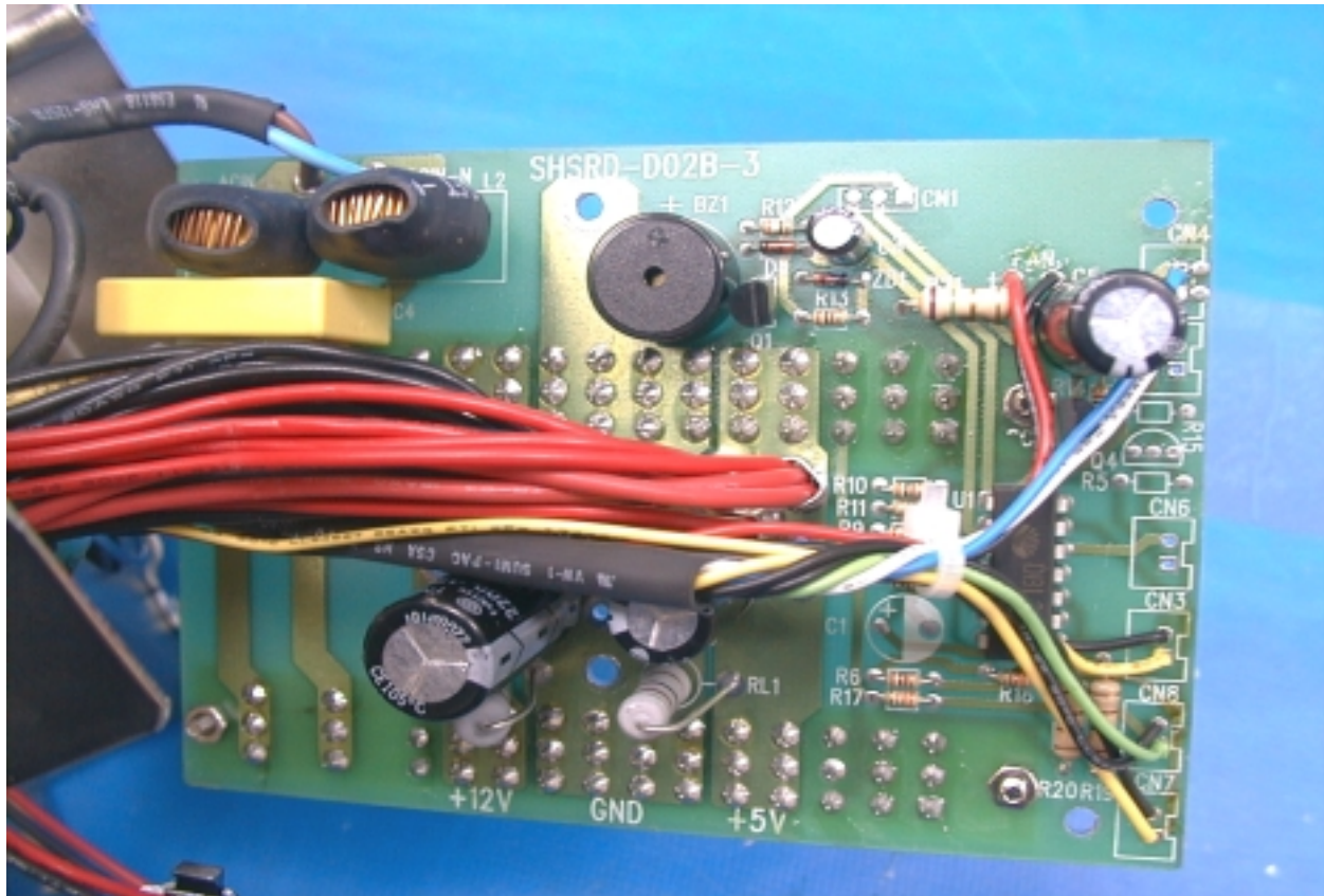
PHOTO. 17. POWER SUPPLY COMPONENT SIDE VIEW
