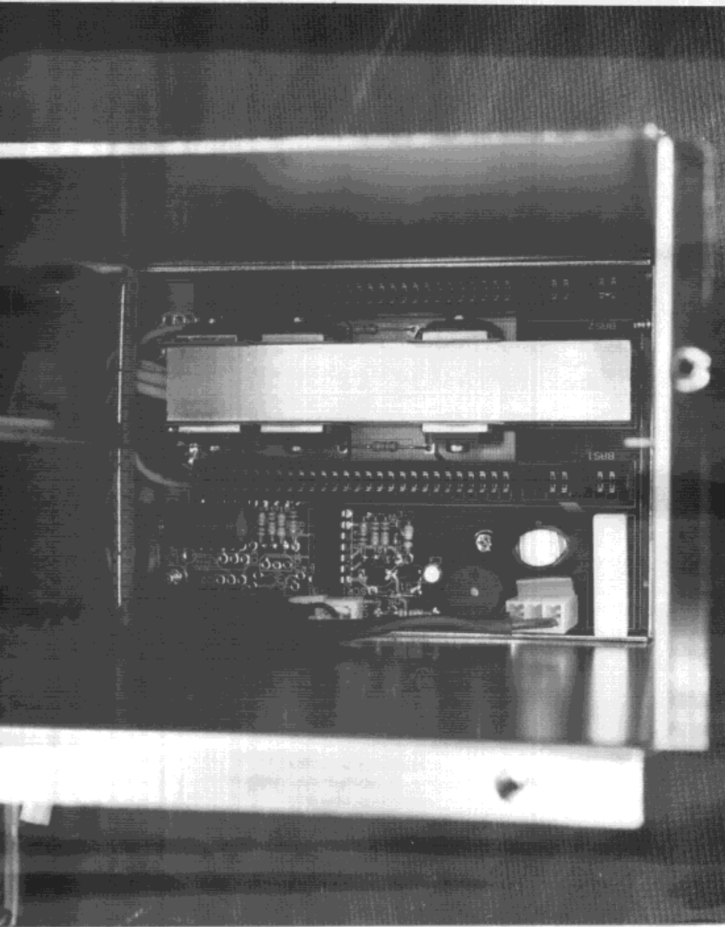
PHOTO 10. POWER SUPPLY INSIDE VIEW
