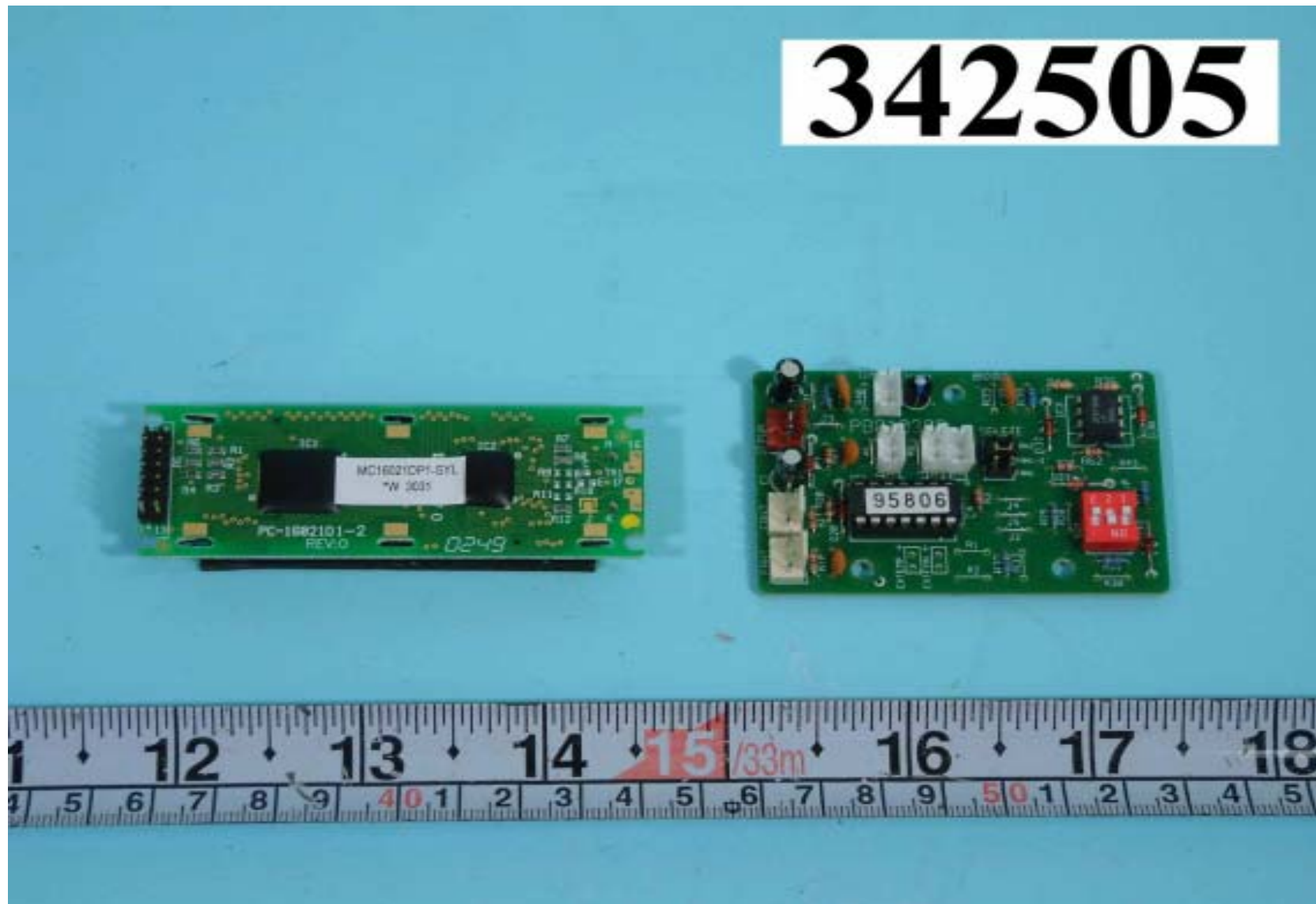
Rear side of LCD module and environment control card
