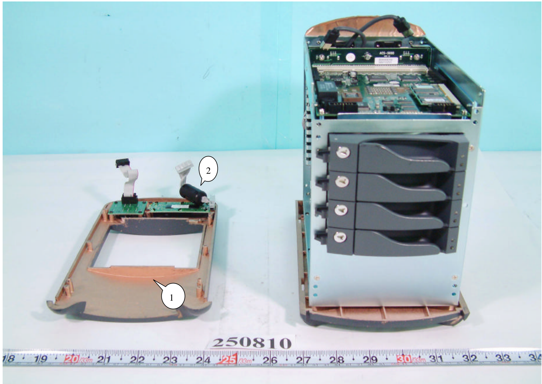
Mechanical Construction
