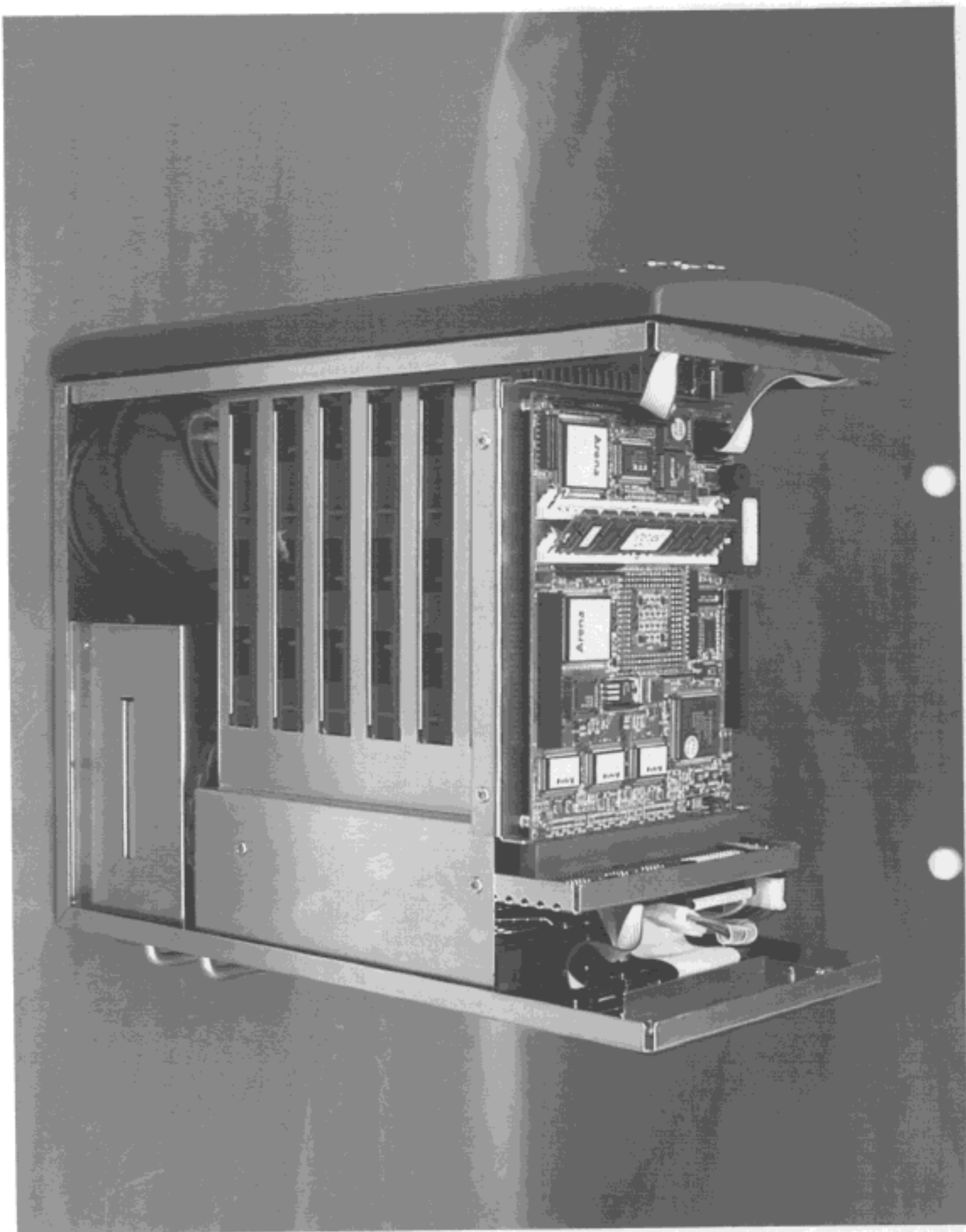
PHOTO 4. EUT INSIDE VIEW
