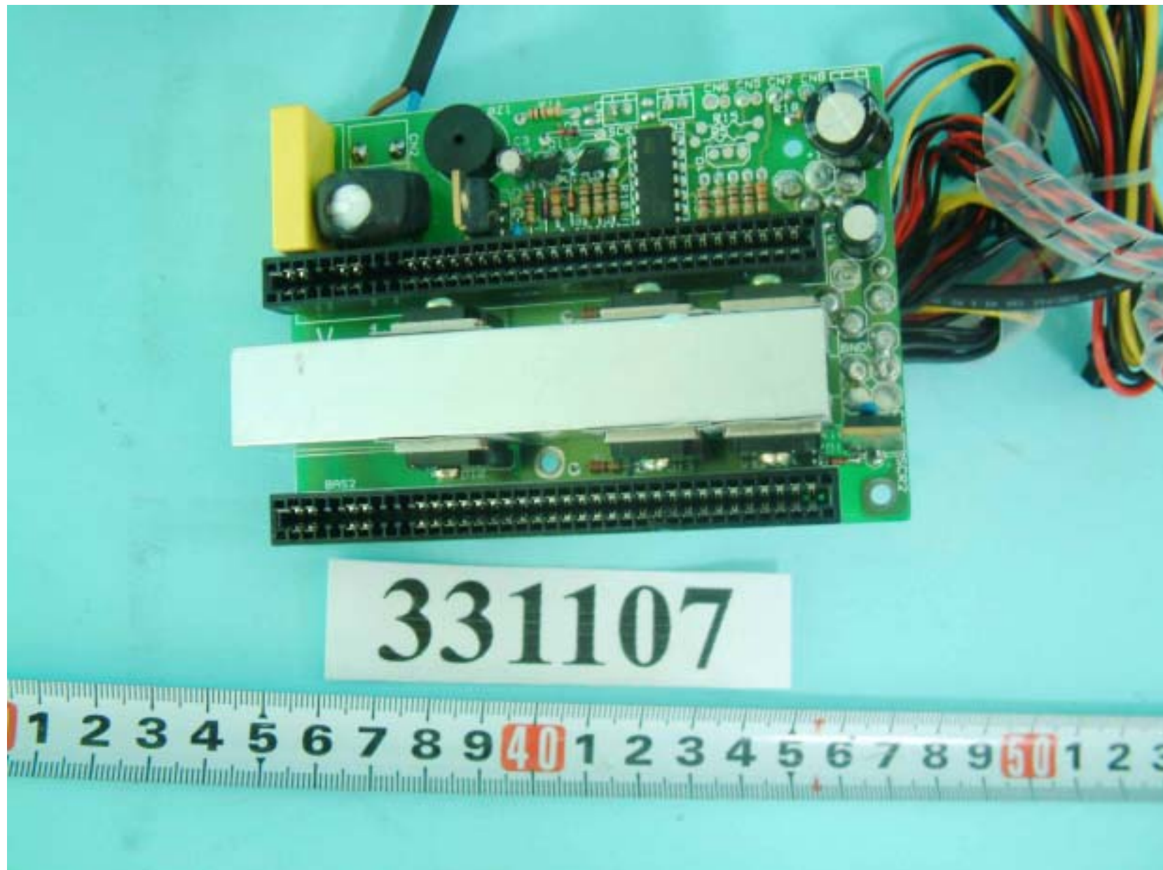
Front side of back plane of power
