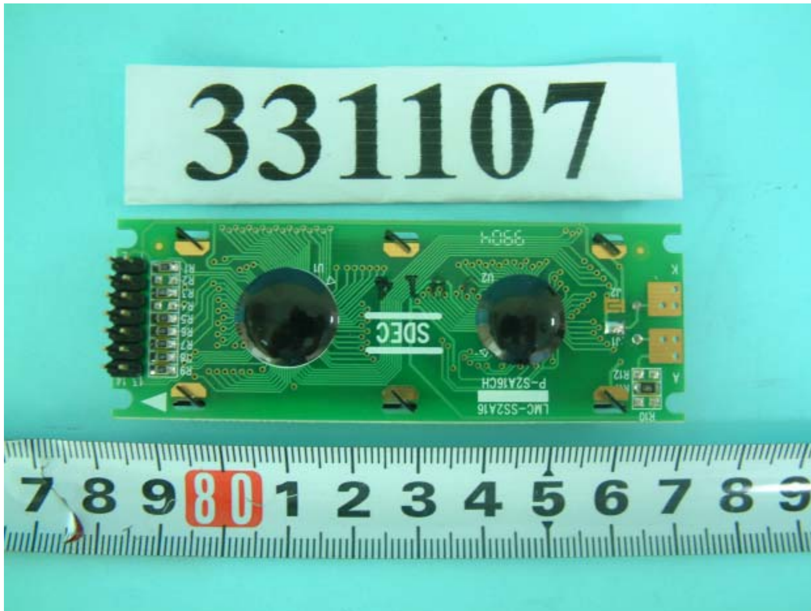
Rear side of LCD module
