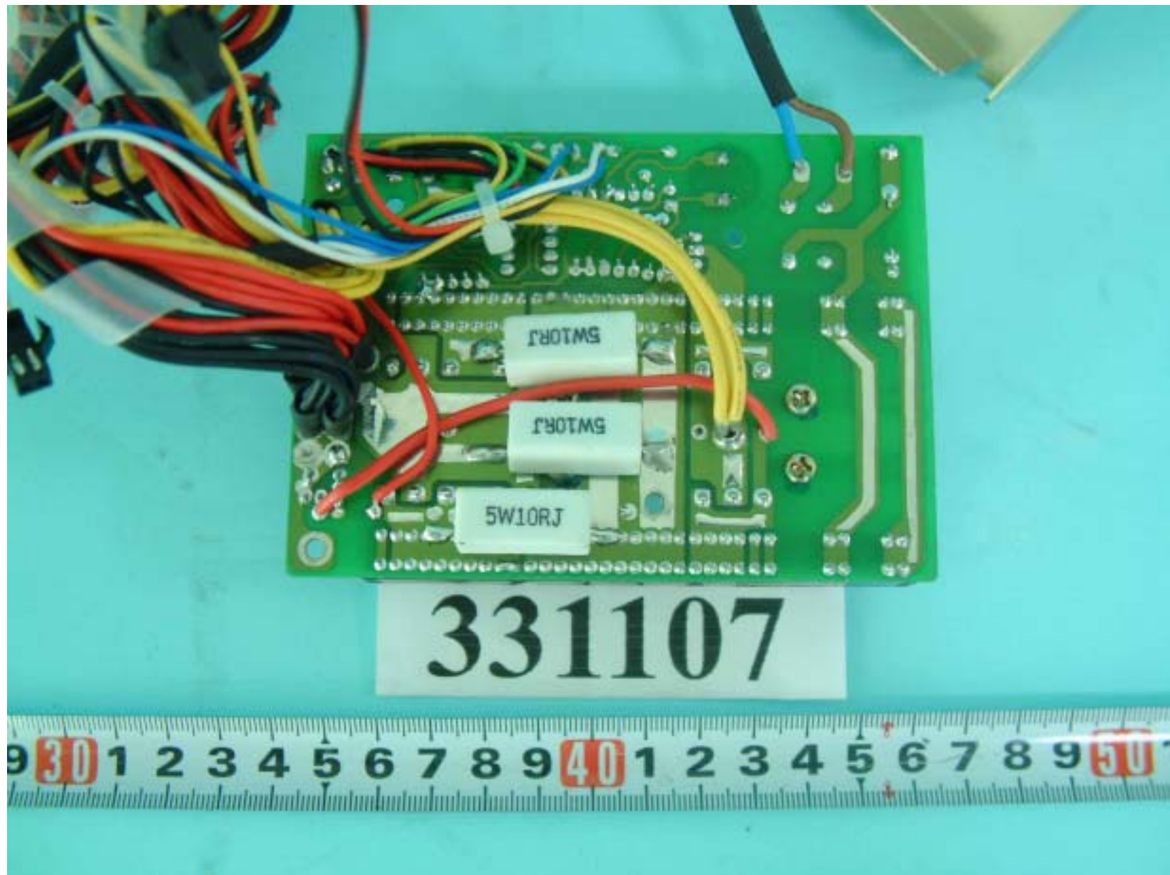
Rear side of back plane of power
