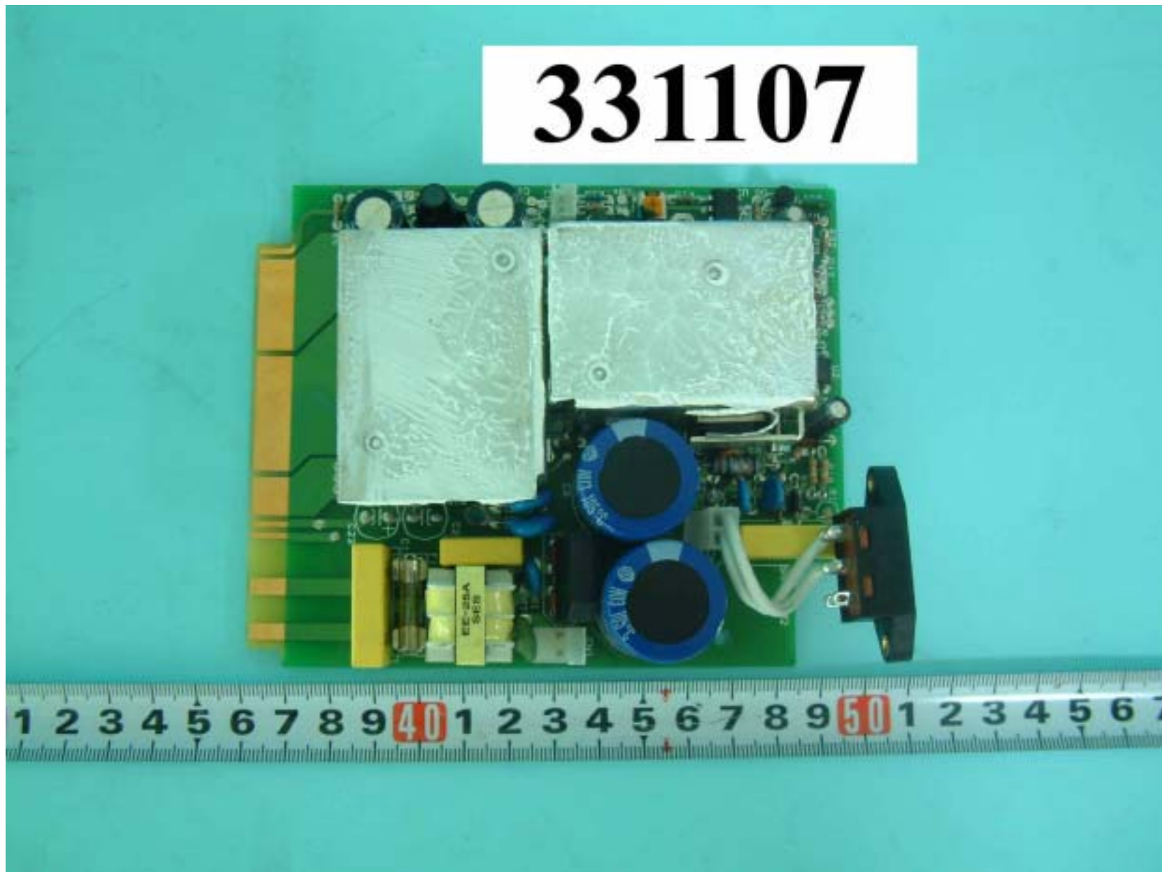
Front side of main board of module power
