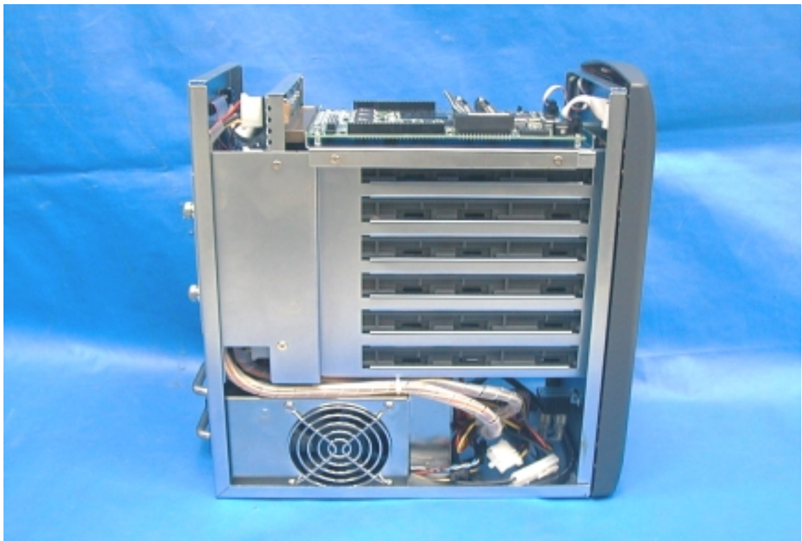
PHOTO. 4. EUT INSIDE VIEW
