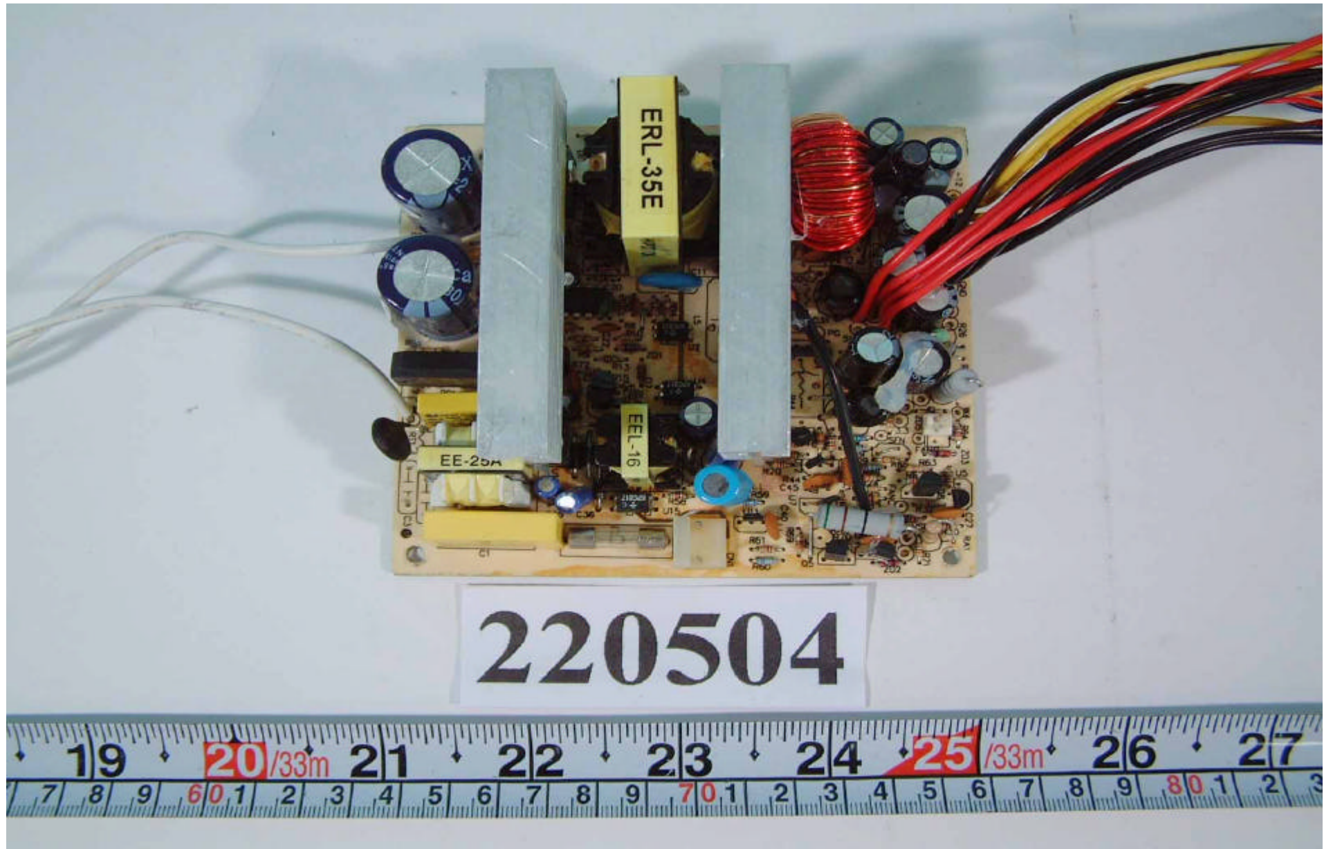
Front SIDE of Main board
