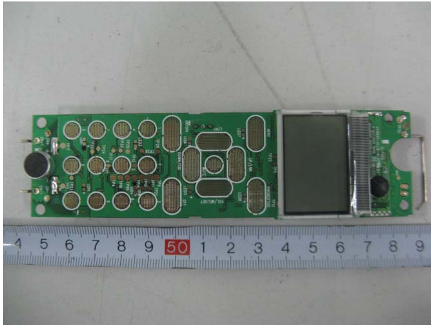
EUT – Main Board with Shielded Cover Bottom View (Handset)
