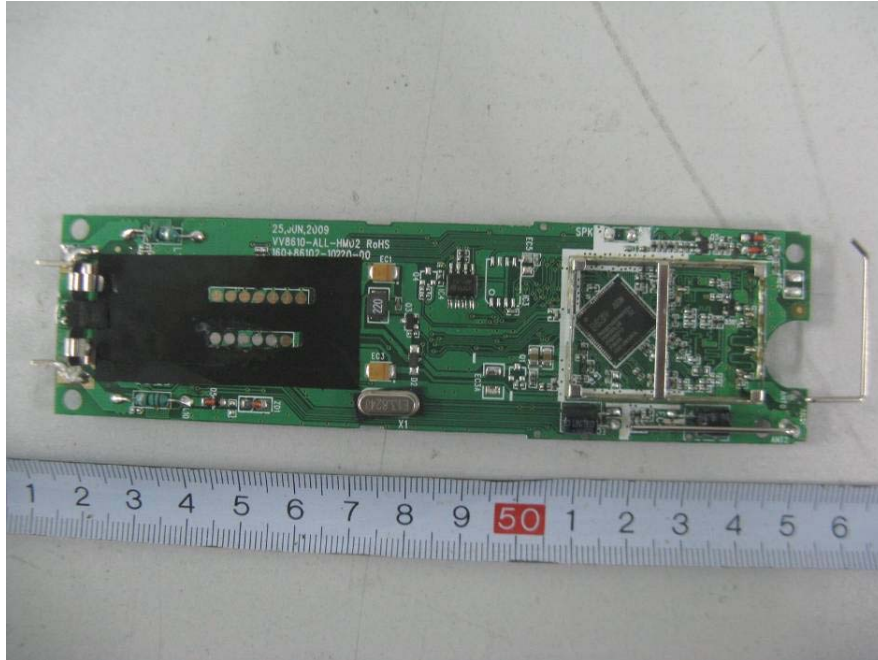
EUT – Cover off View (Charger)
