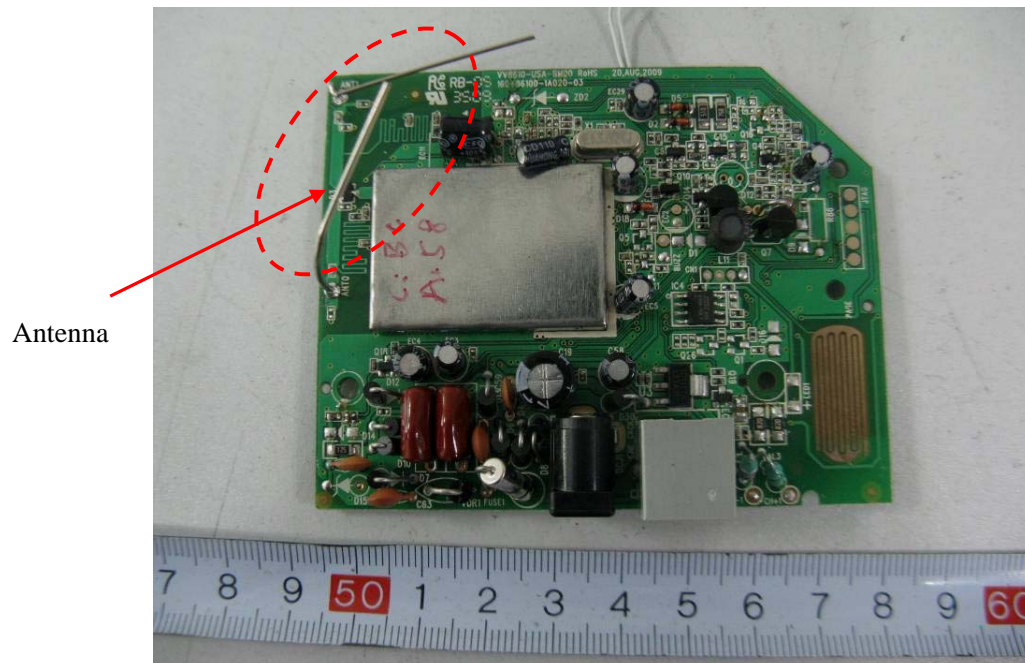
EUT – Main Board with Shielded Cover Top View
