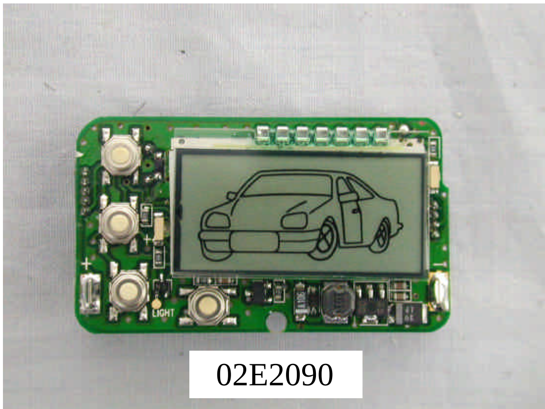
Photo 3 Unit partially Disassembled
