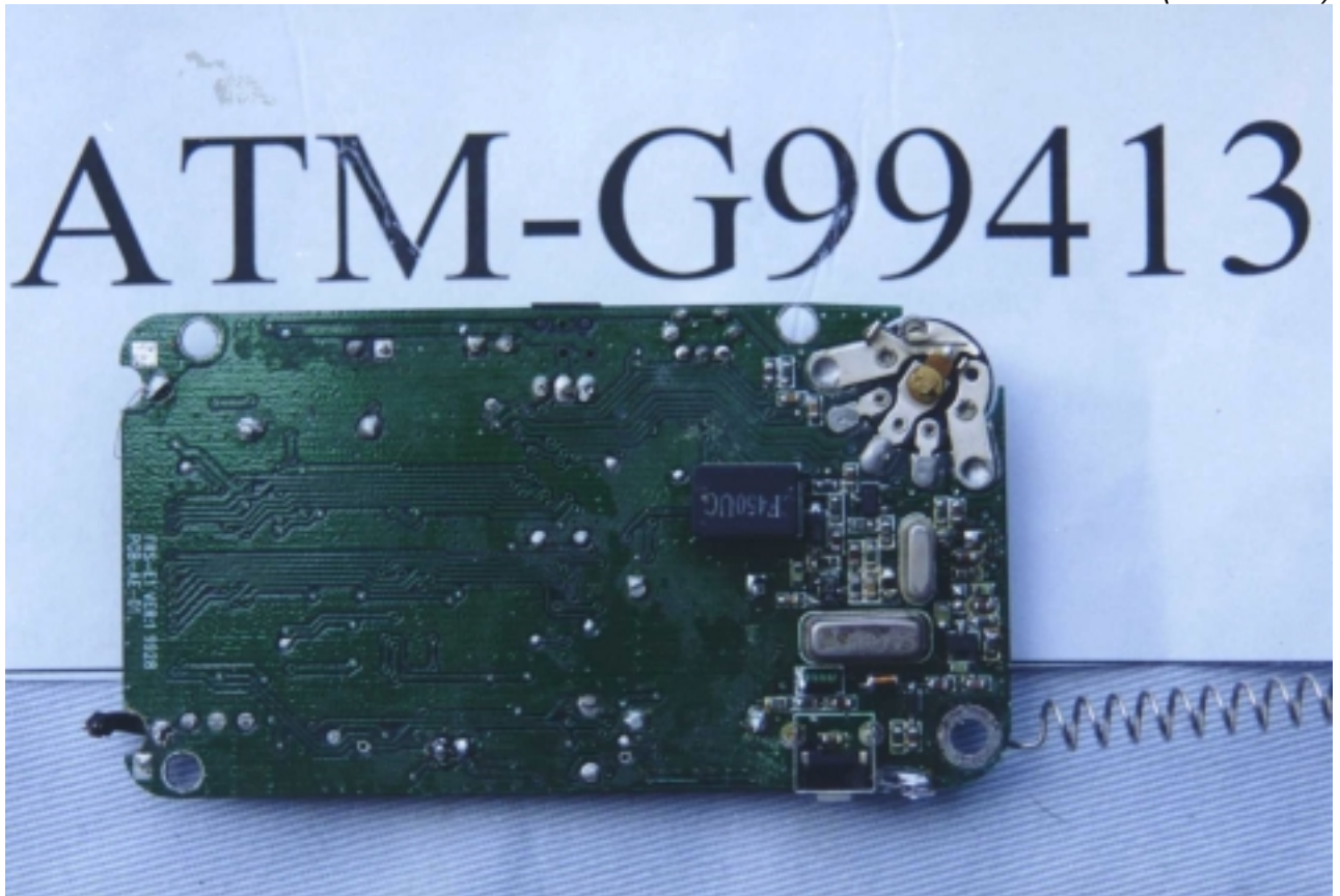
Photo 7 Main Board (Back Side)
