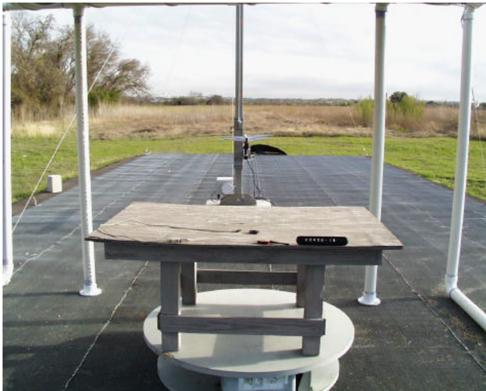
Radiated Emissions – Back View
