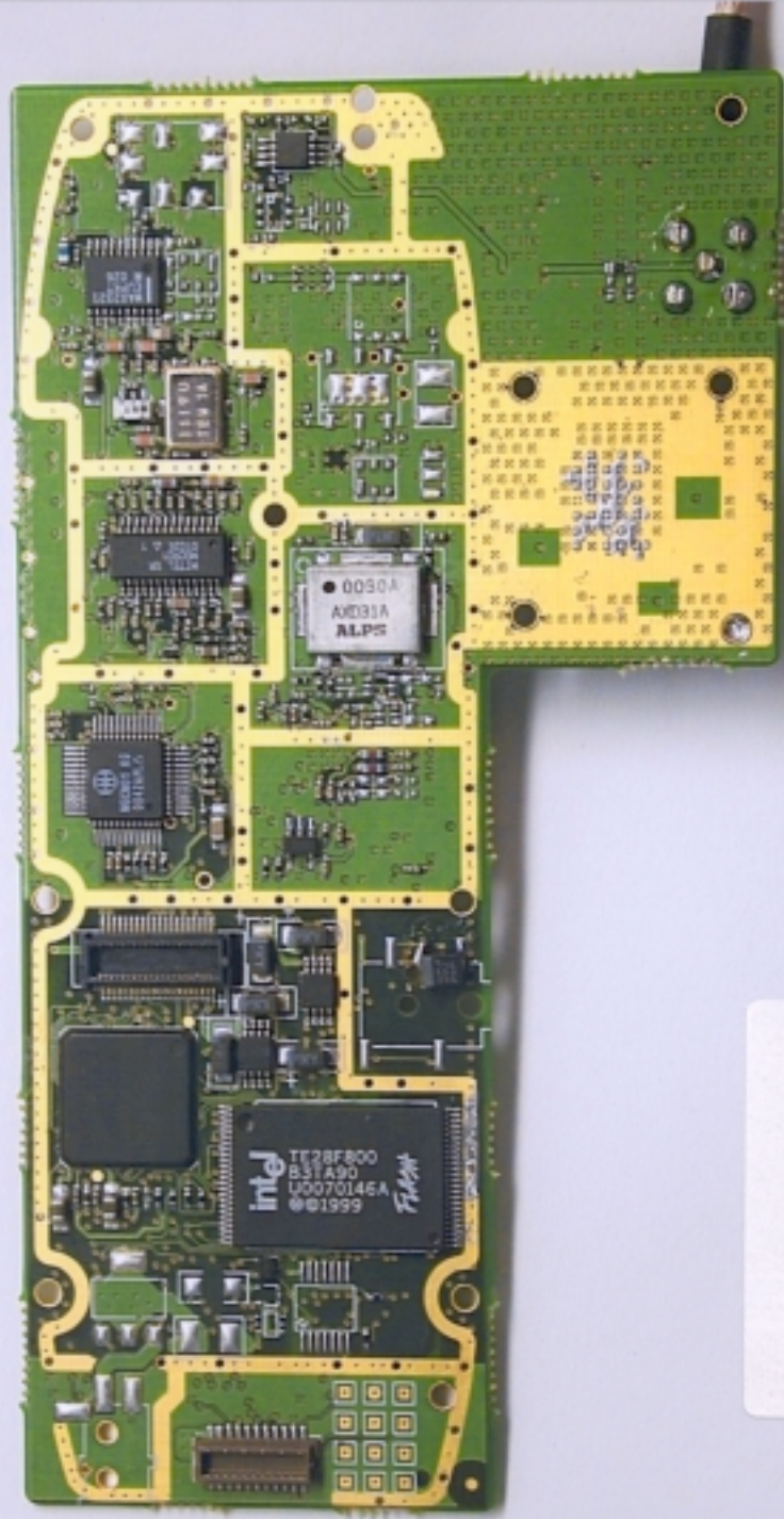
FWT-8100 TDM 3W PCB Assembly Bottom FCC ID NJFW8100
