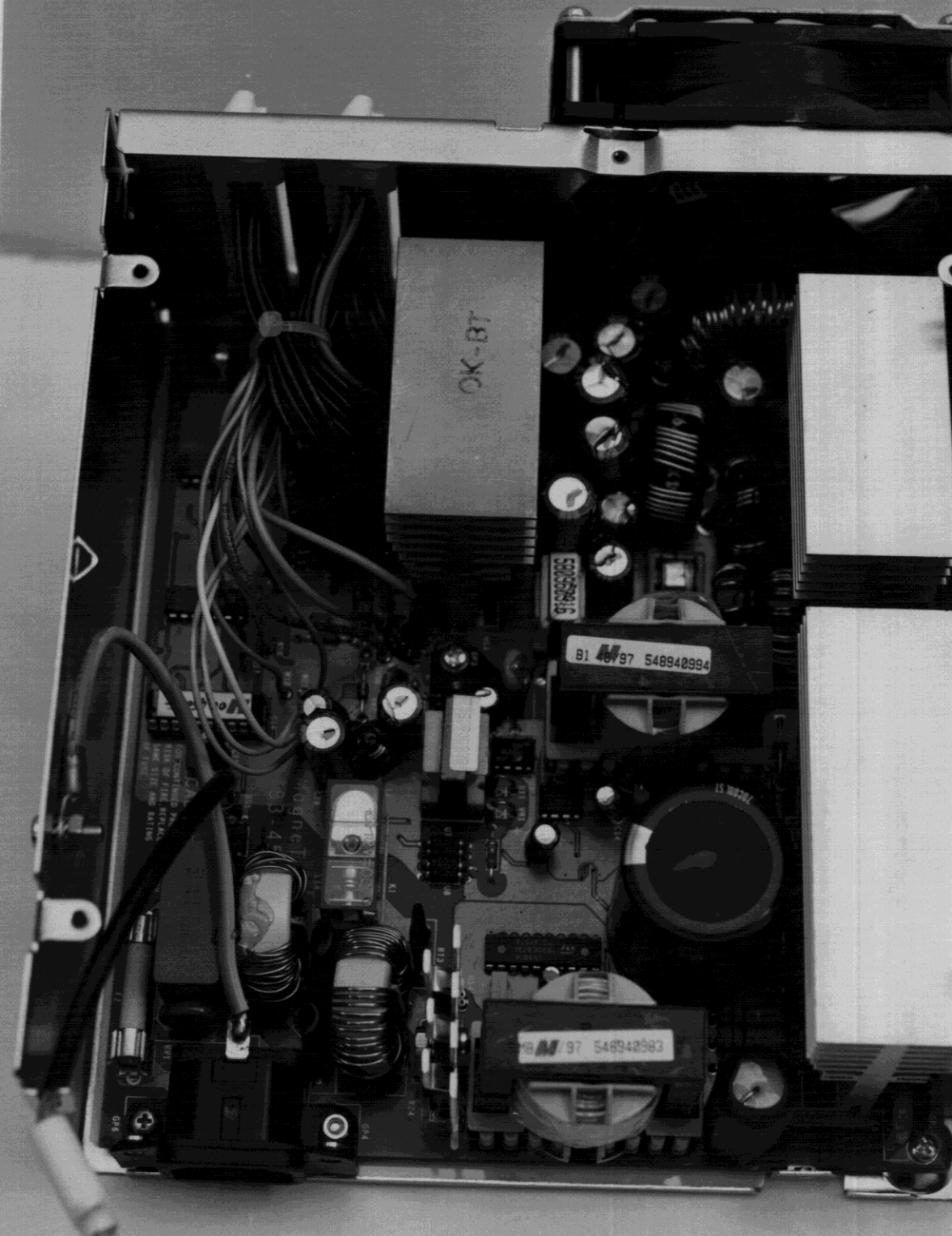
Fig. 8.12 Power Supply Unit MAGNETEK model 3783-45-2. Components S
