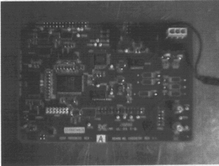
FIGURE 17: DSP PCB top side
