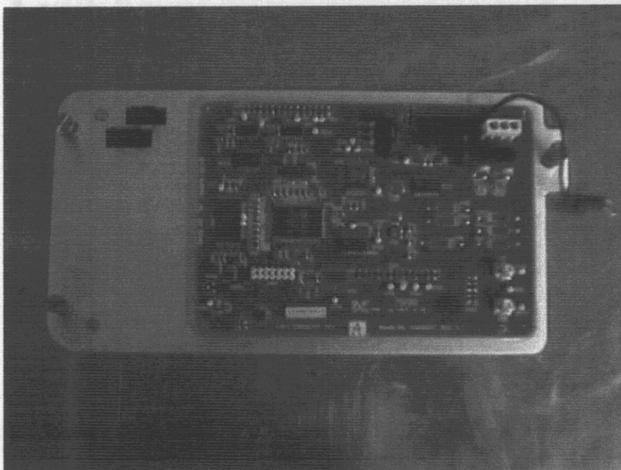
FIGURE 29: DSP/Analog PCB/Mounting board top
