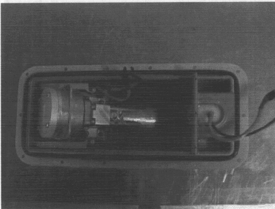
FIGURE 24: Microwave sensor/ultrasonic unit bottom inside
