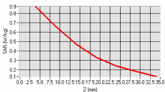
SAR, Z Axis Scan (X = -15, Y = -6)
