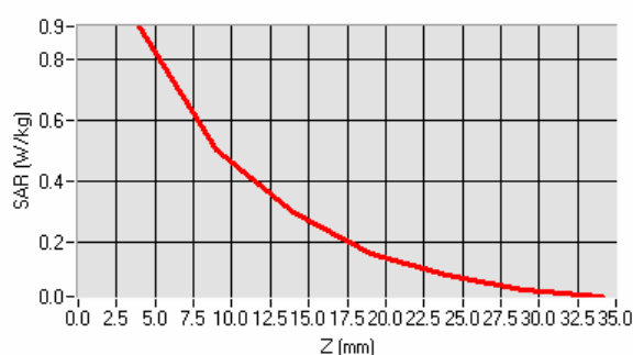
SAR, Z Axis Scan (X = -16, Y = 1)
