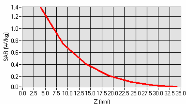
SAR, Z Axis Scan (X = 1, Y = 37)
