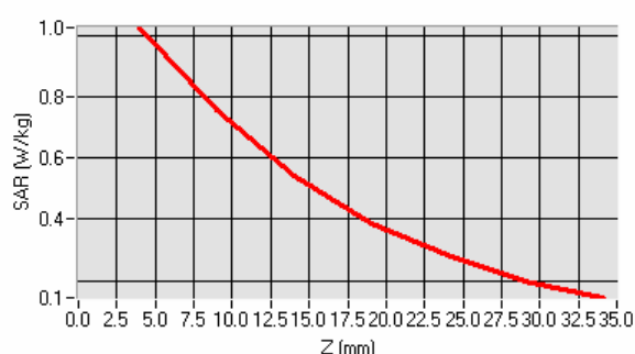
SAR, Z Axis Scan (X = -14, Y = -5)
