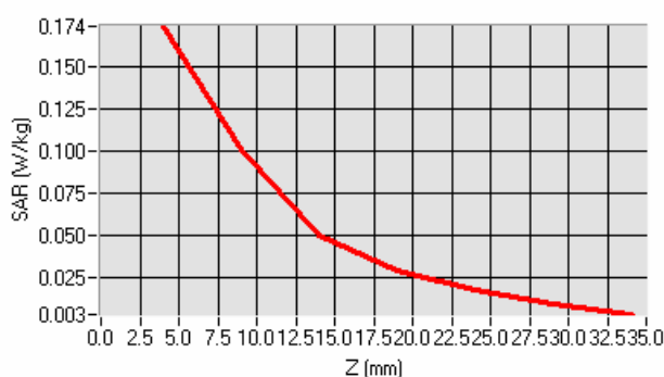
SAR, Z Axis Scan (X = -5, Y = -17)
