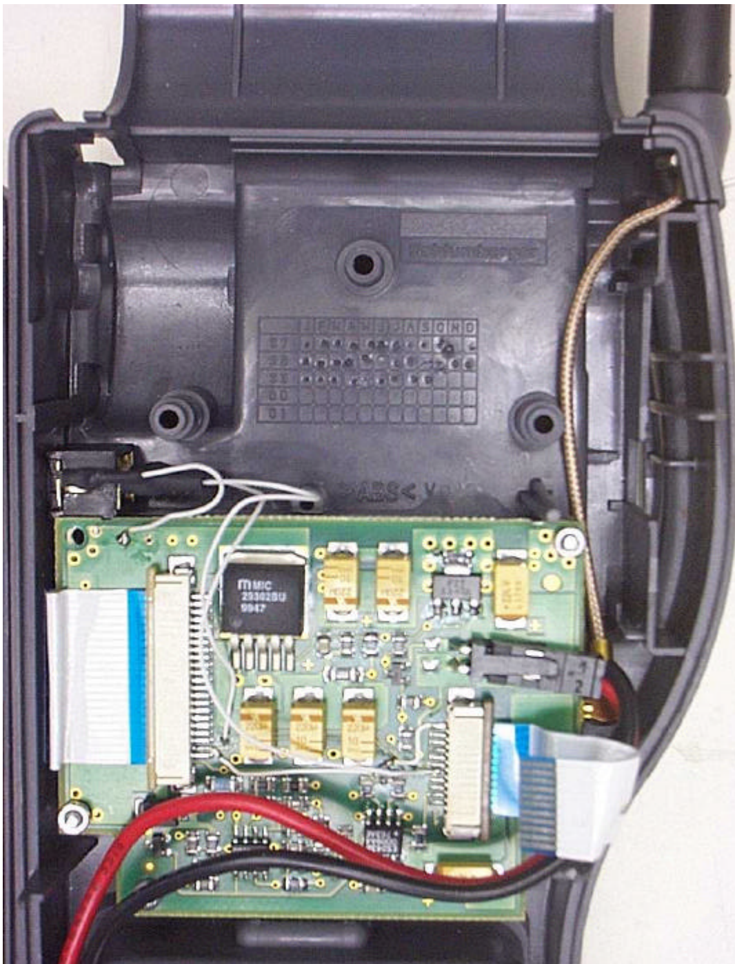
Board covering wireless modem
