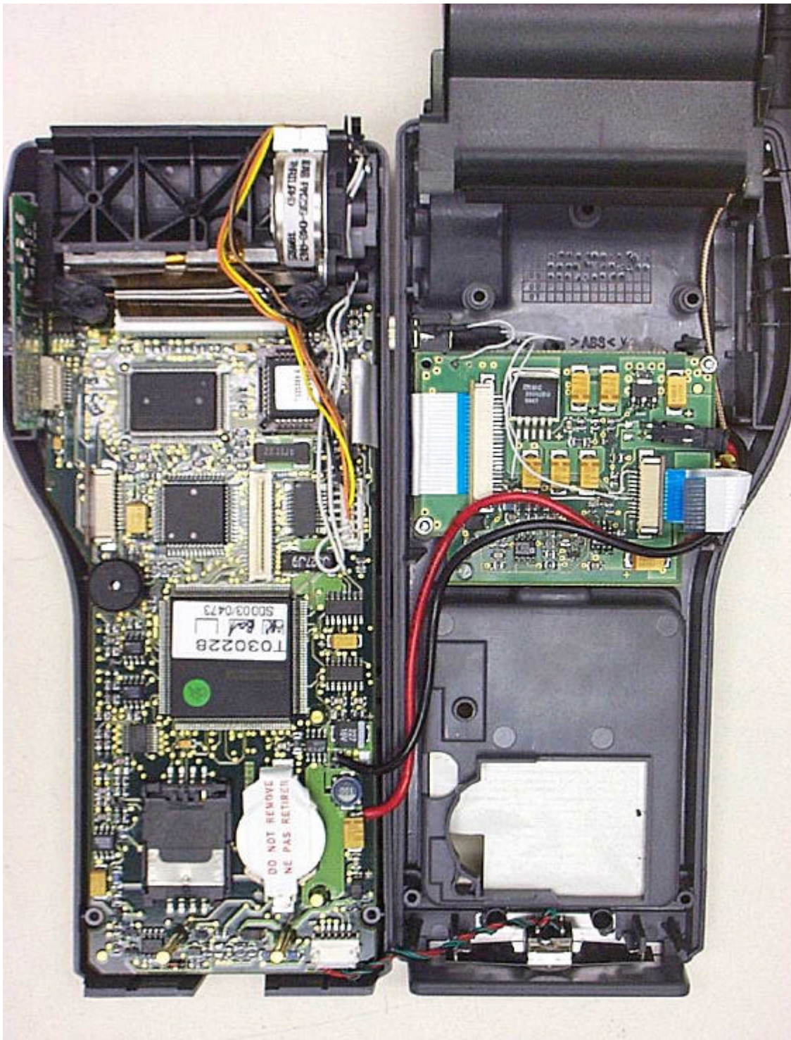
Interior of Schlumberger Magic 9000
