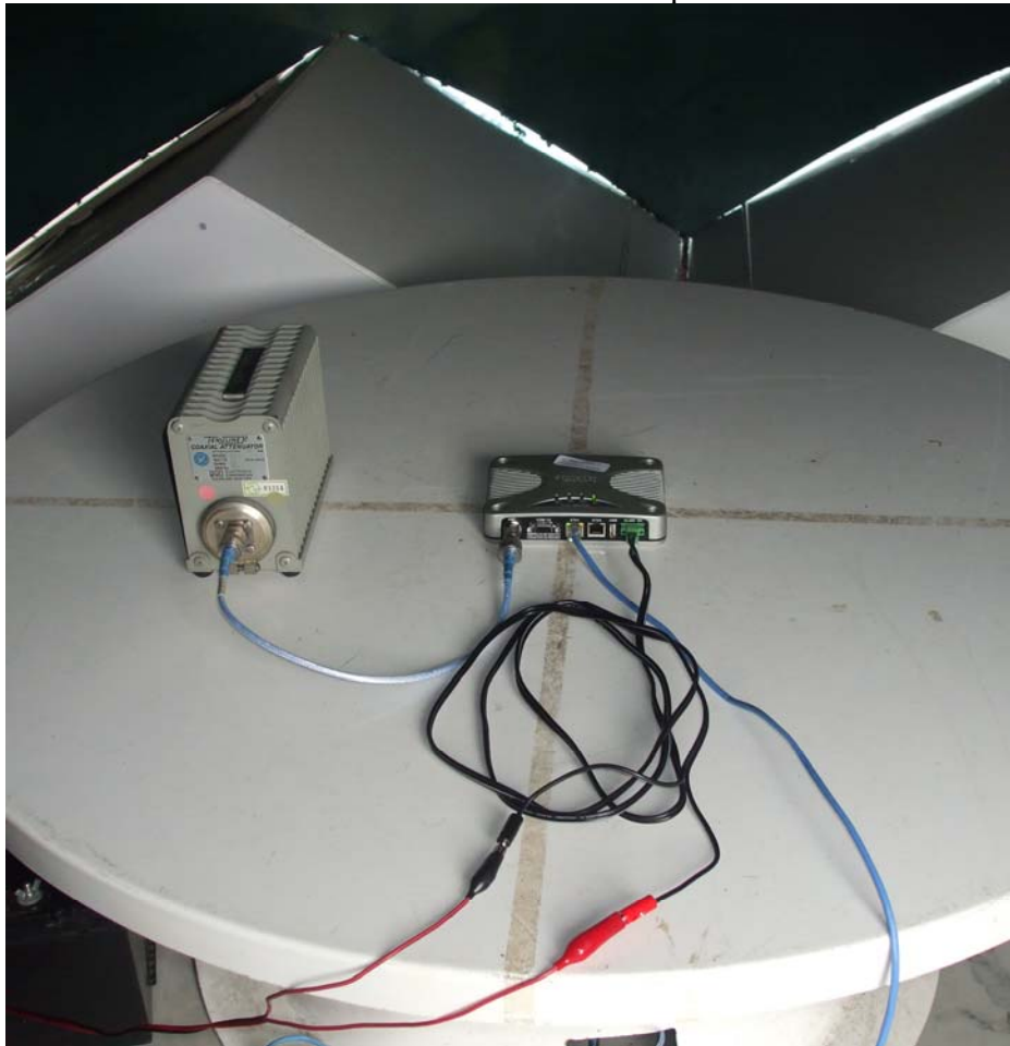
Radiated emissions setup
