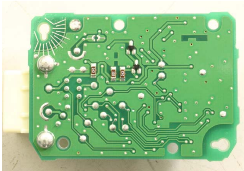
Solder Side
