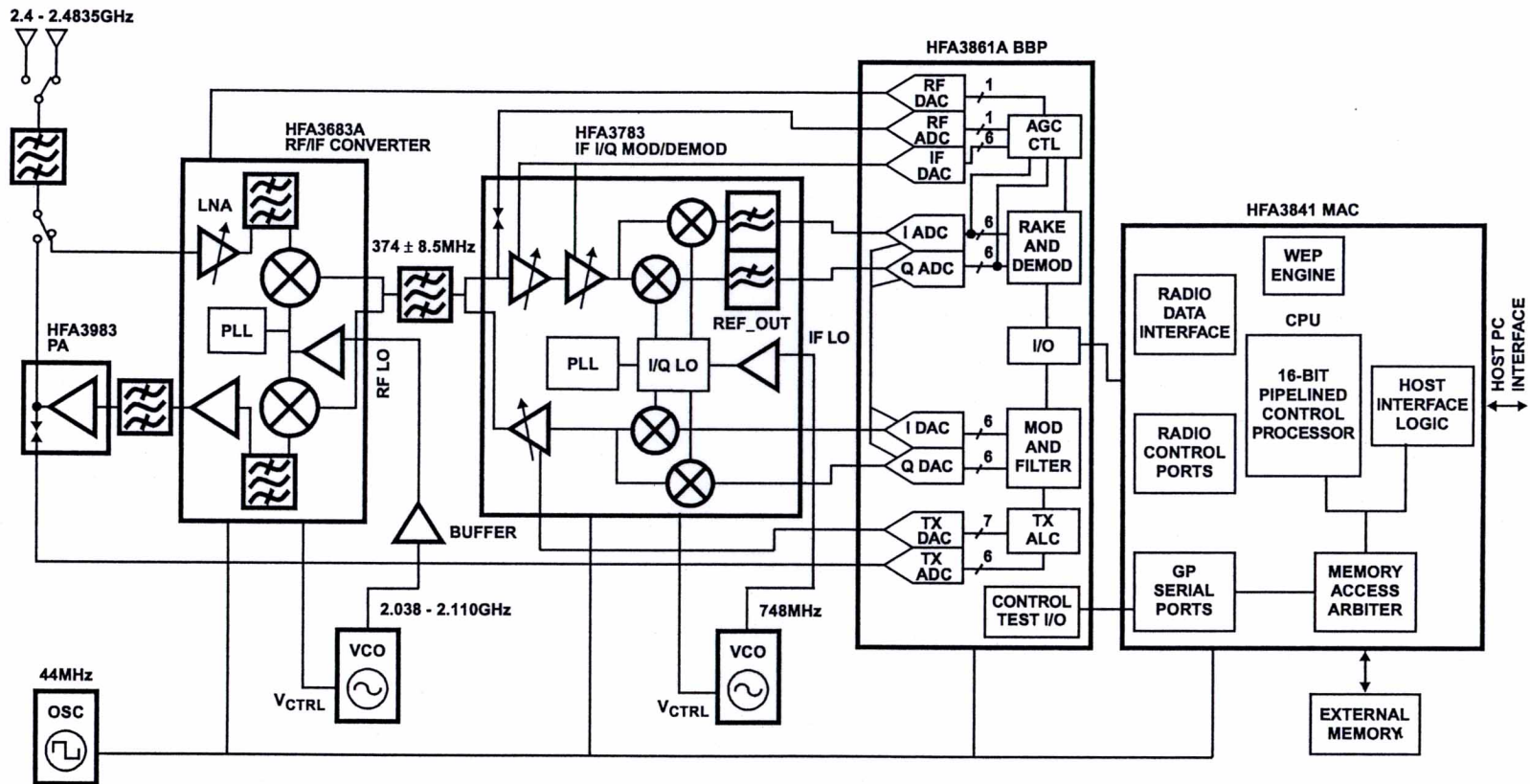
SL-2011CD WIRELESS LAN CARD BLOCK DIAGRAM
