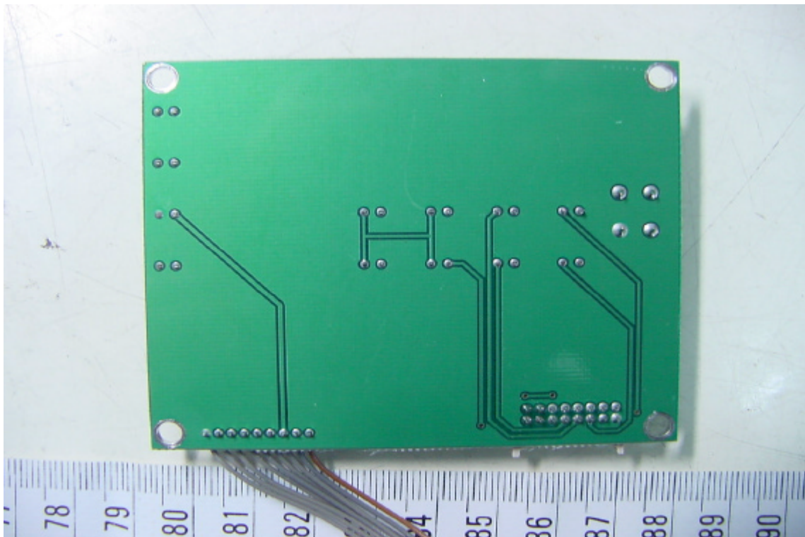
Solder View of Main PCB (DC Converter)
