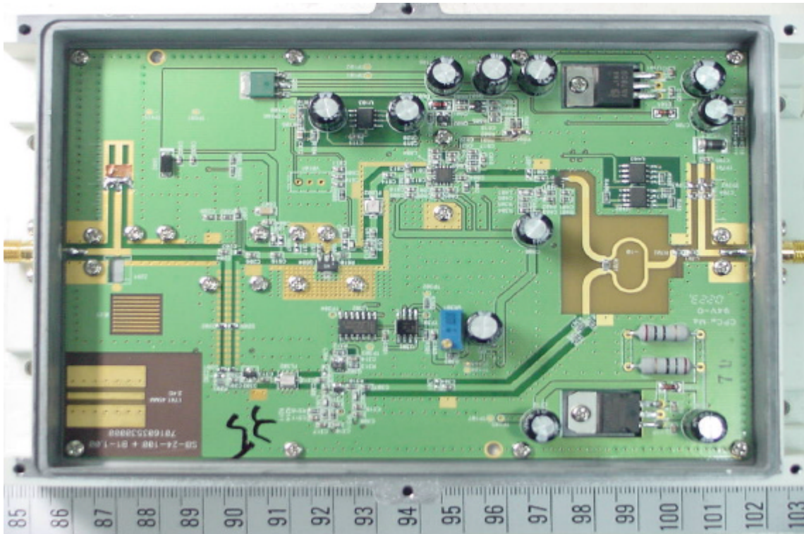
Rear View of RF Power Amplifier
