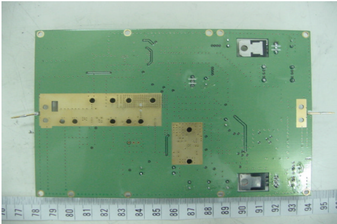
Solder View of Main PCB (RF Power Amplifier)
