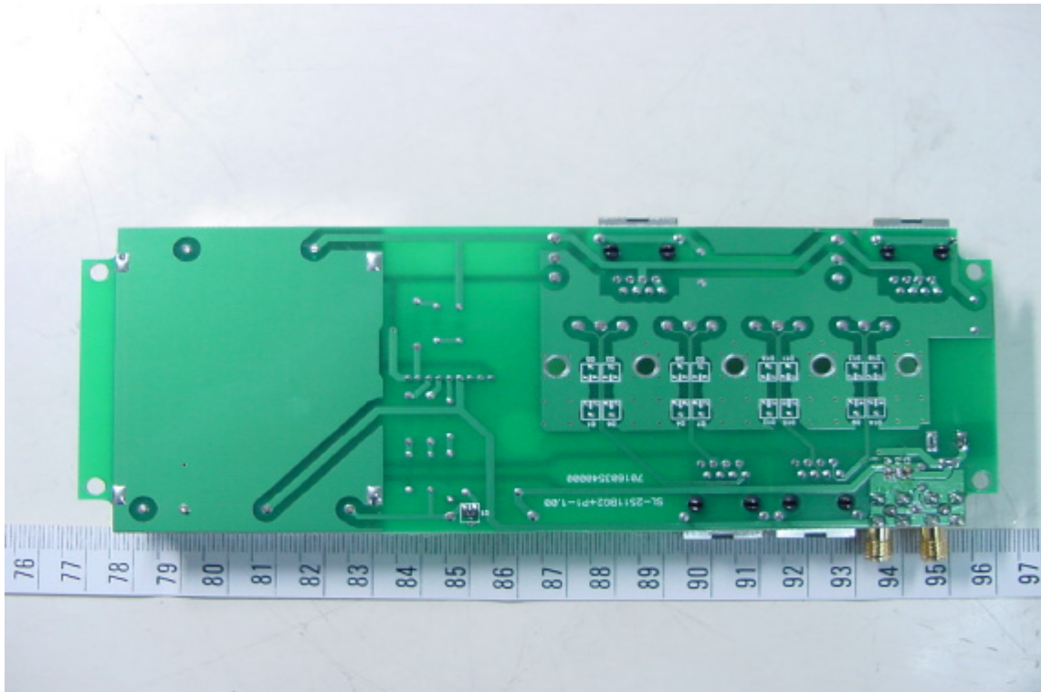
Solder View of PCB (Bridge Indicator)
