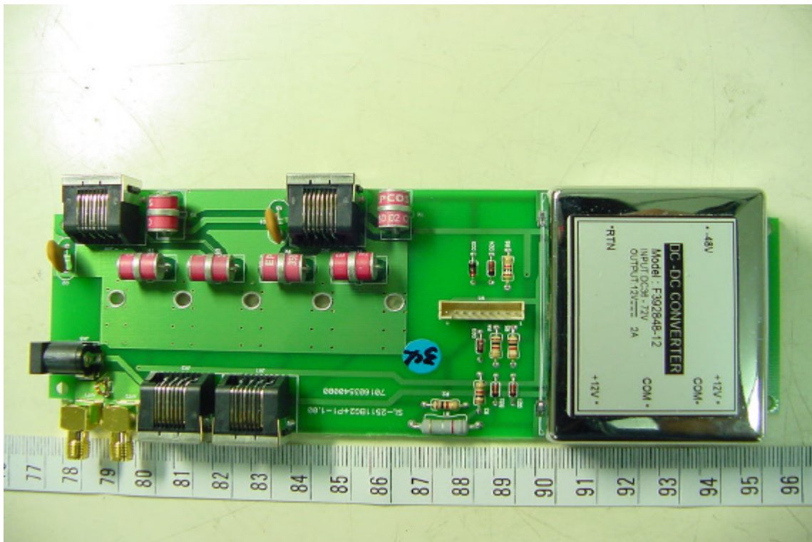
Component View of Main PCB (Bridge Indicator)
