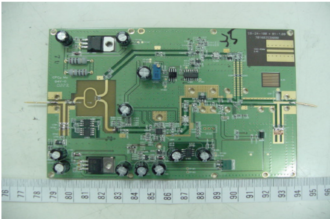
Component View of Main PCB (RF Power Amplifier)
