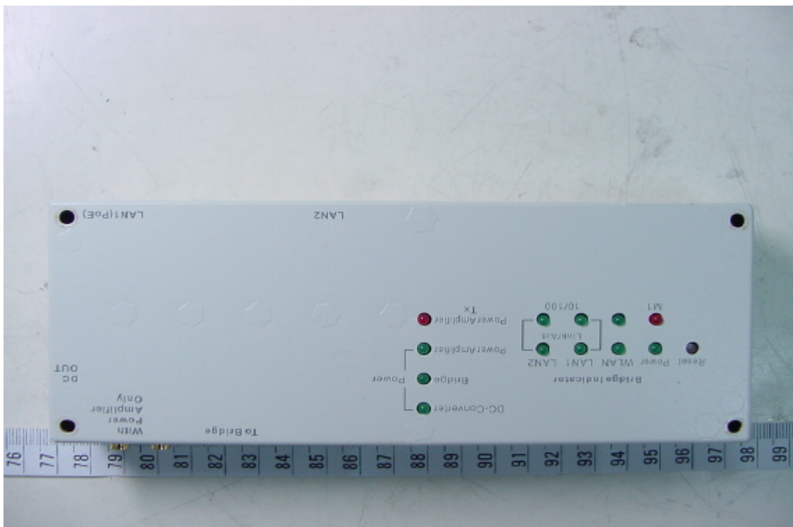
Front View of Bridge Indicator
