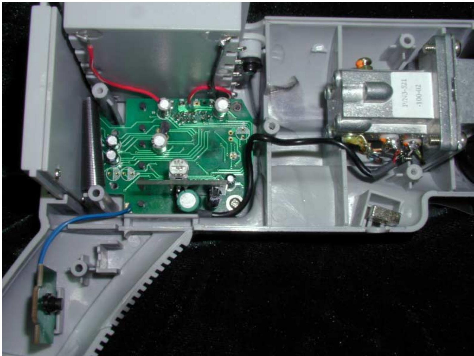
TOP VIEW
