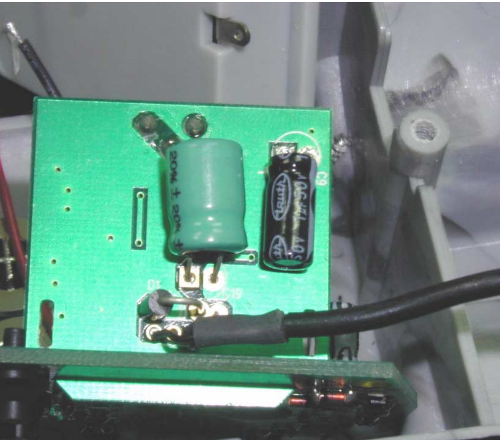
PREAMP BOTTOM
