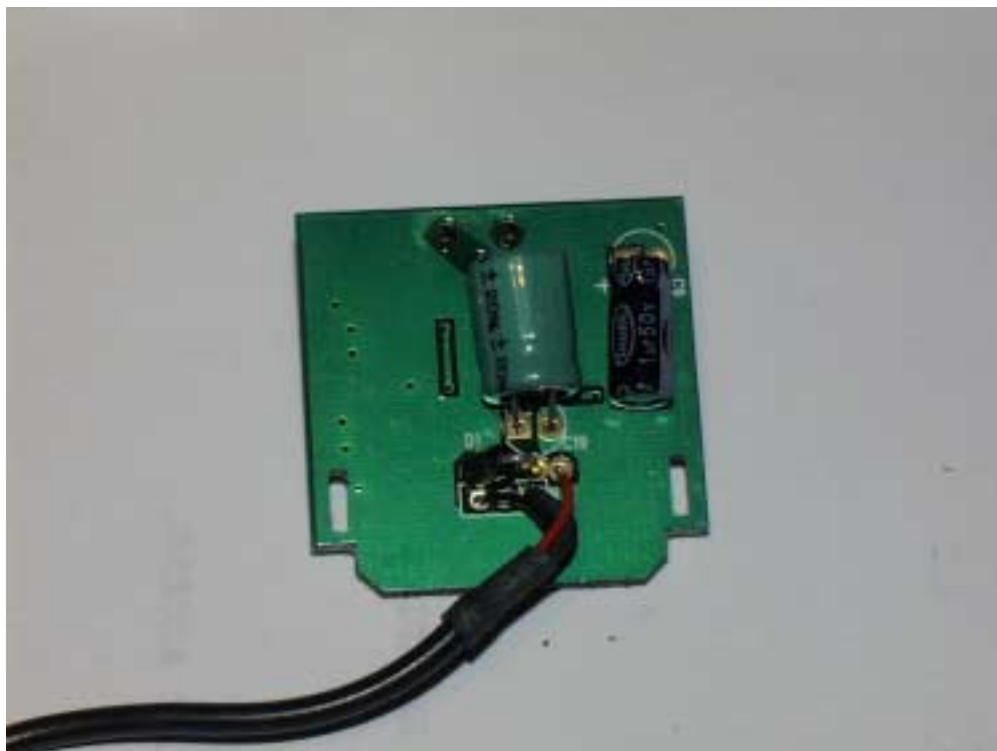
PREAMPLIFIER PCB BACK
