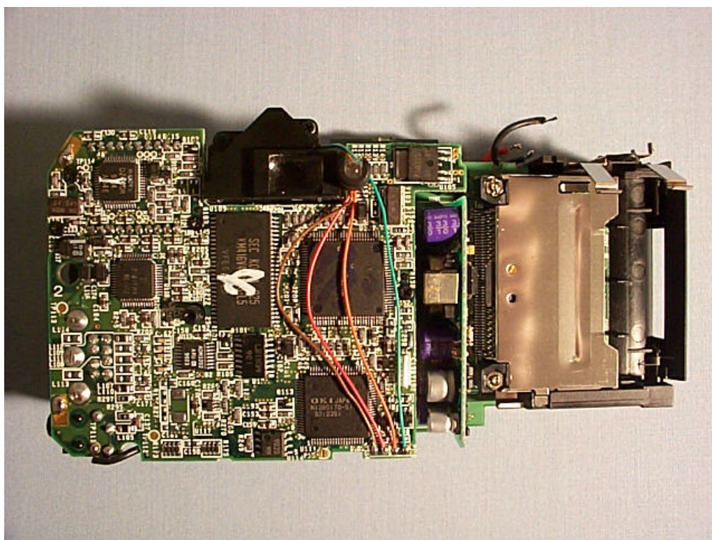
(14)EUT Photo
