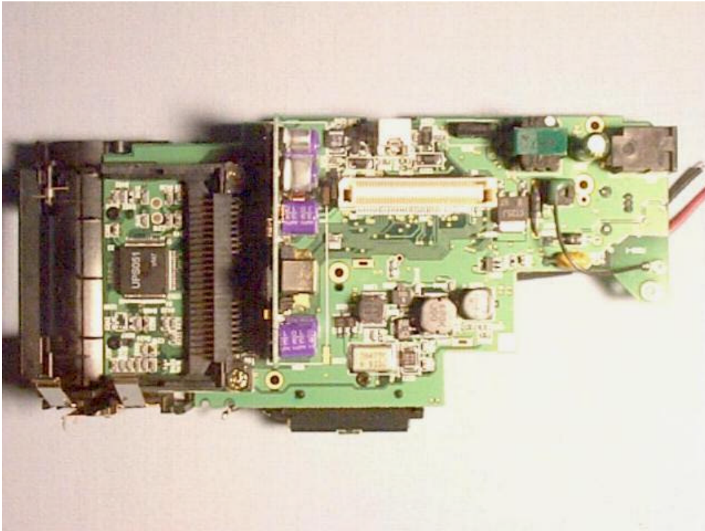
(19)EUT Photo
