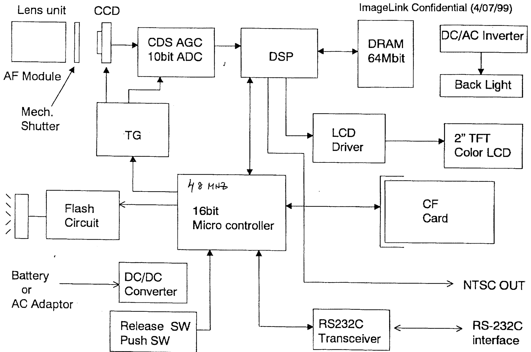
Block Diagram of DC-1500
