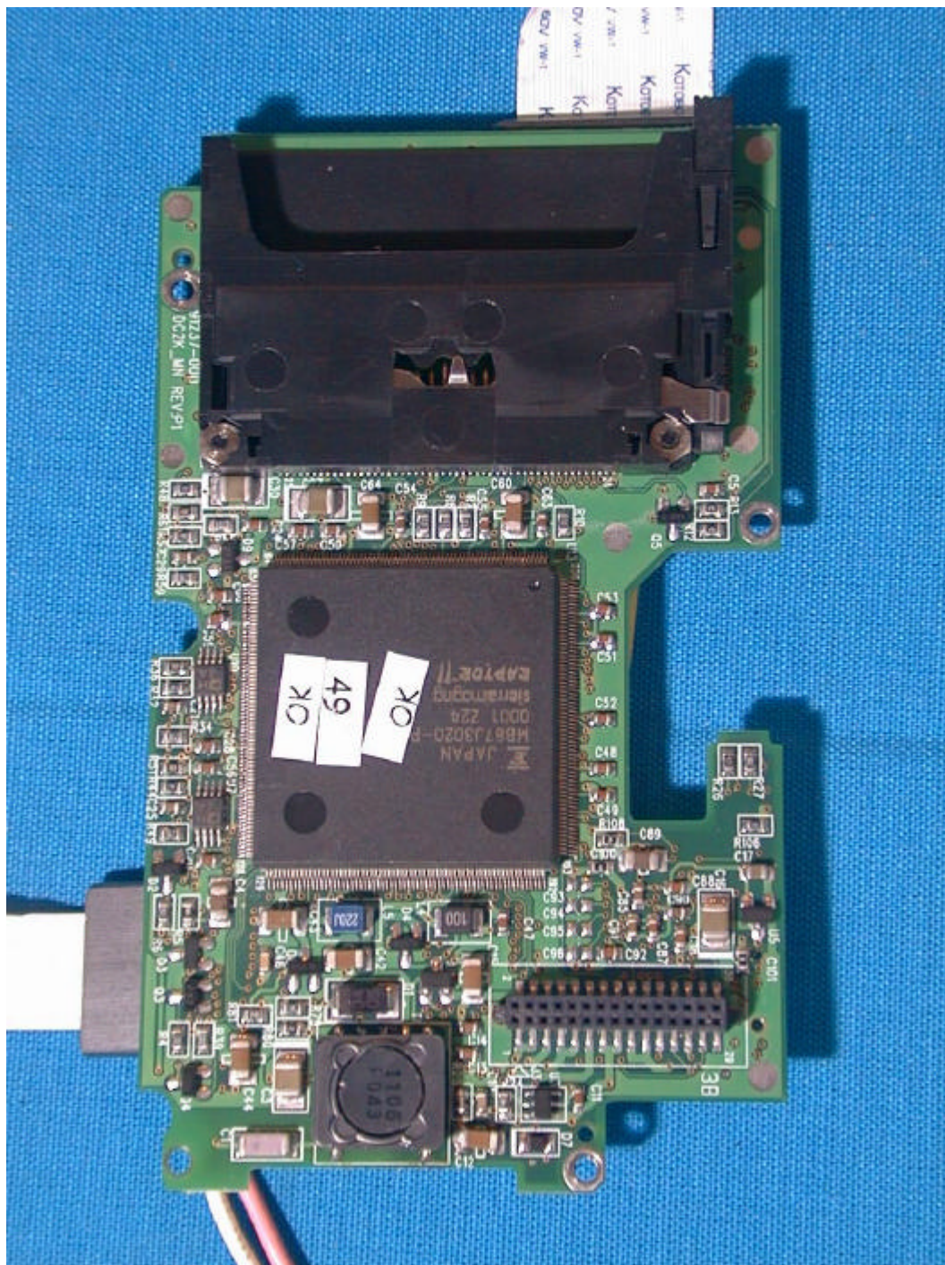
(27) EUT Photo
