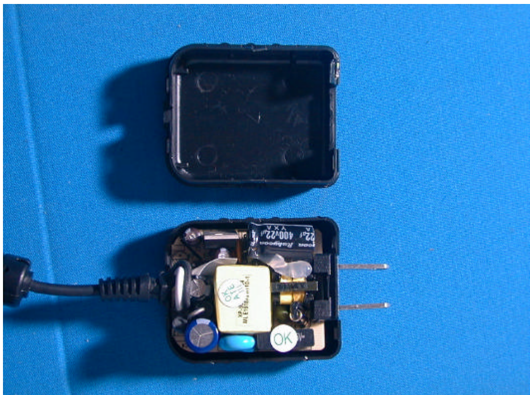
(30) Adapter Photo
