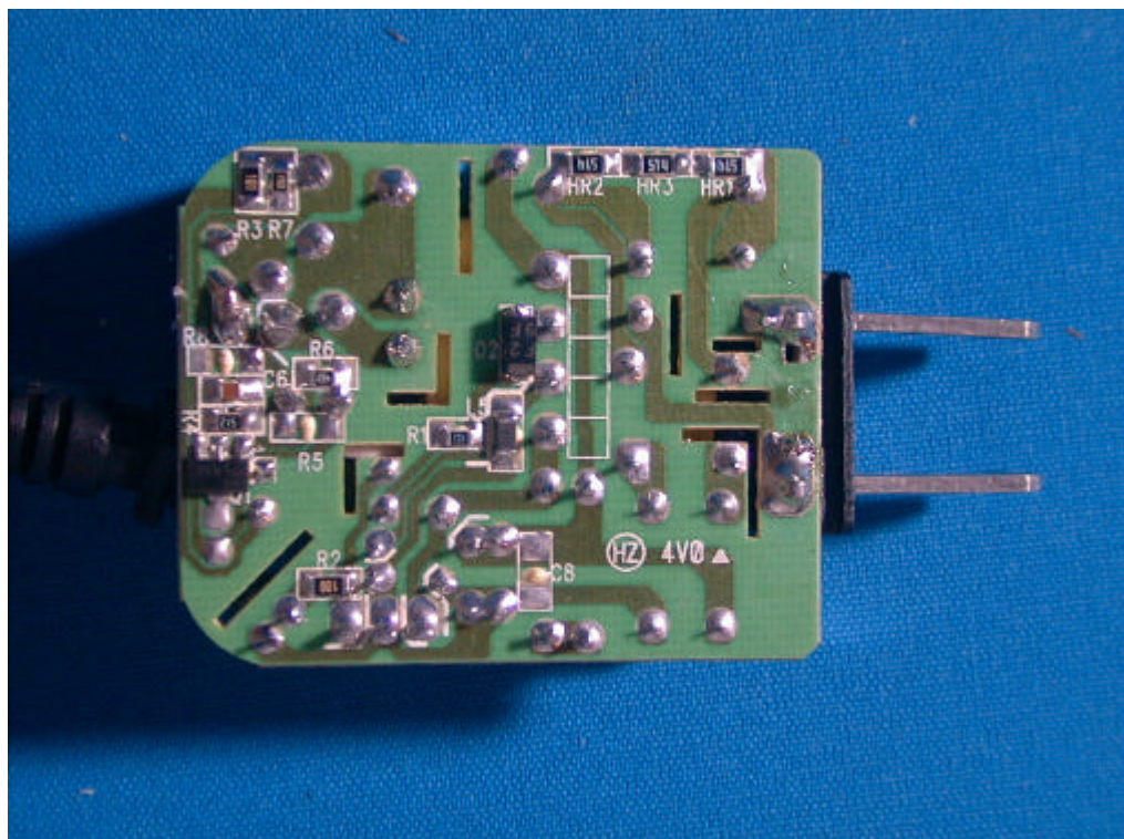
(32) Adapter Photo
