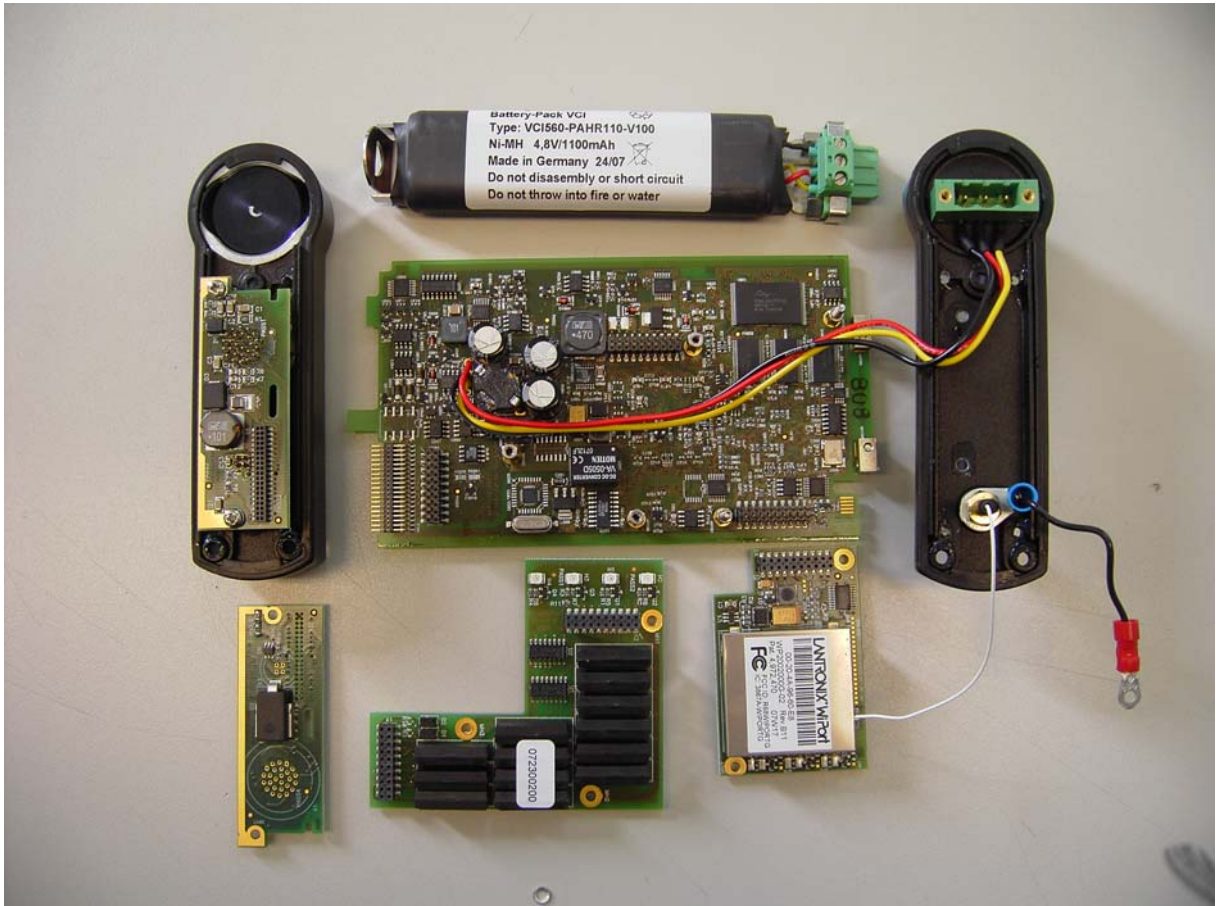
Picture: Internal view (with unmounted PCBs II)
