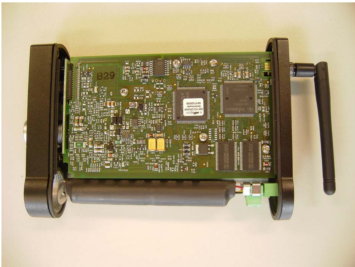
Picture: Internal view bottom
