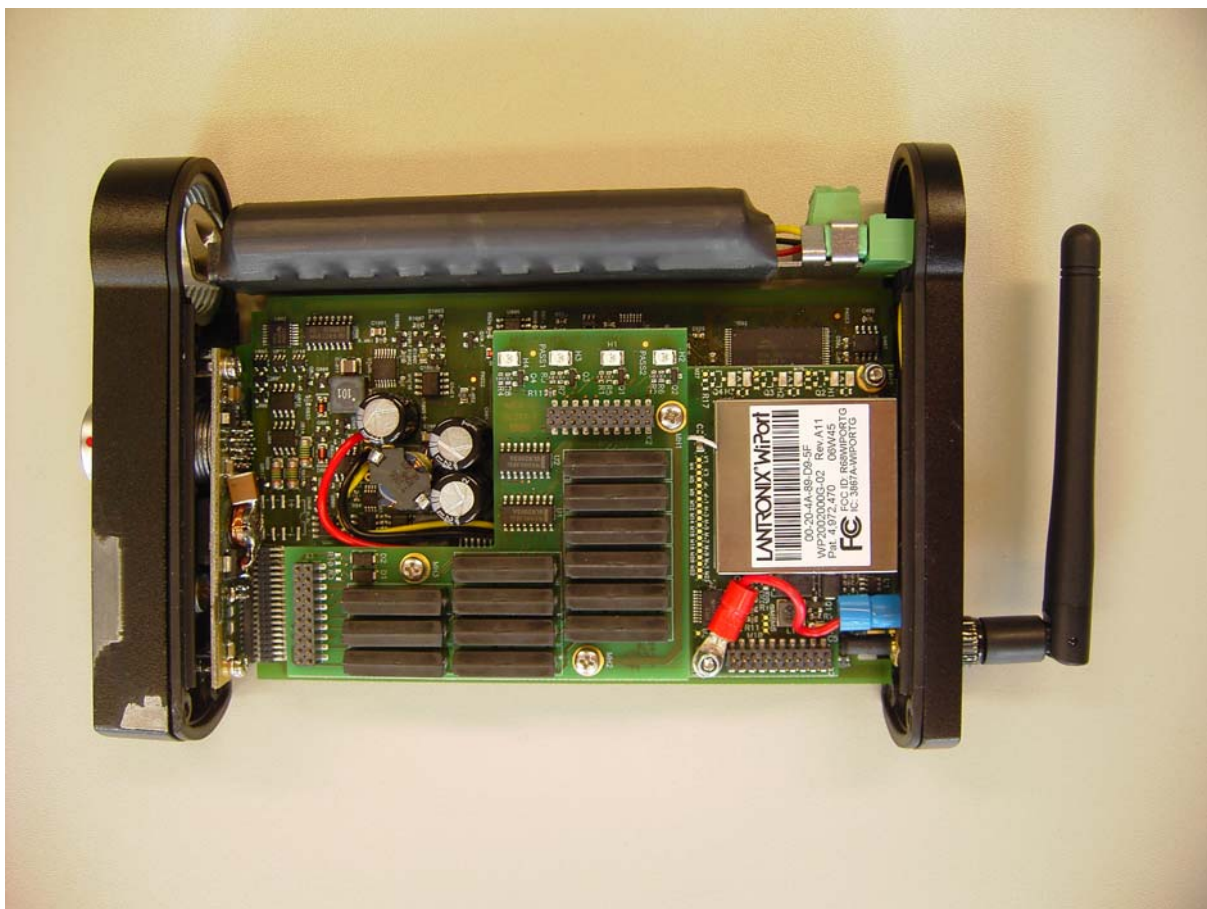
Picture: Internal view top
