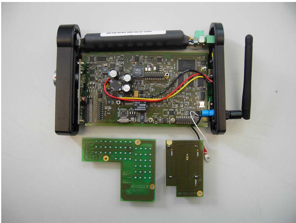
Picture: Internal view (with unmounted PCBs)
