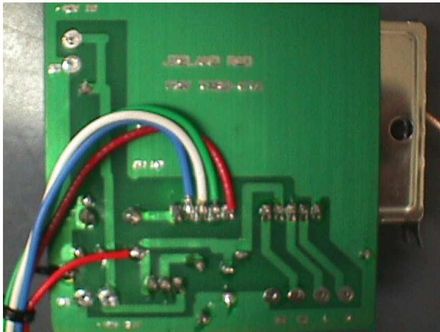
FIGURE 38: 10 TO 15 GHZ
