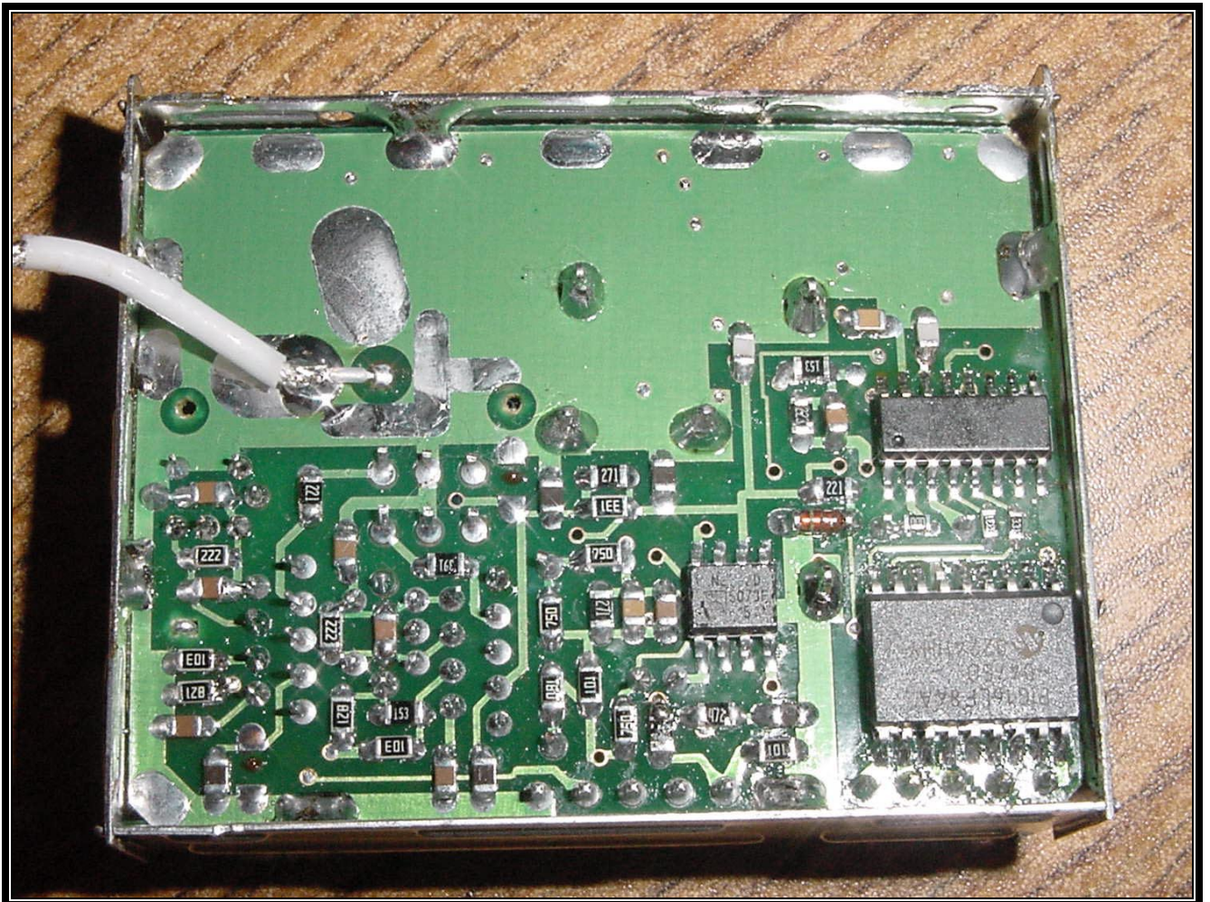
PHOTOGRAPH 11: PCB2 REAR VIEW
