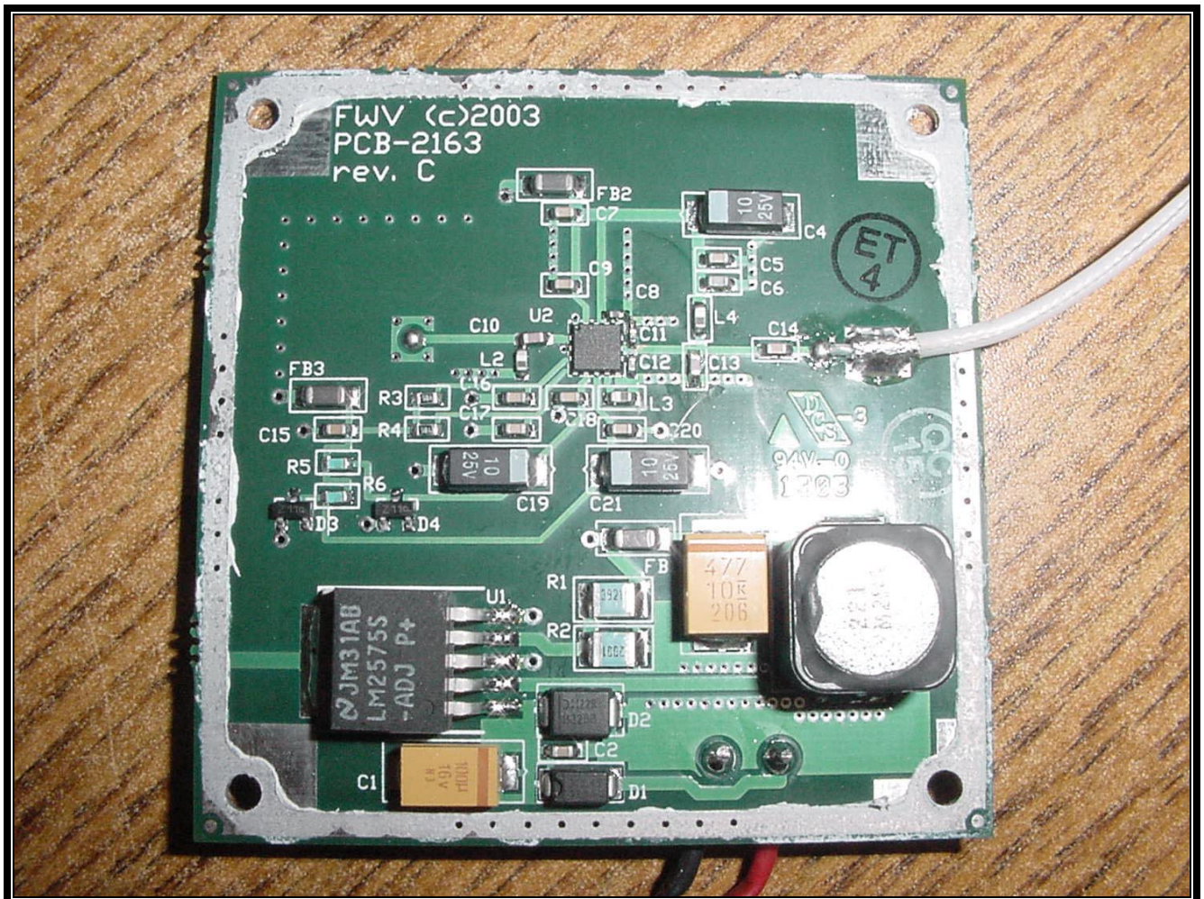
PHOTOGRAPH 8: PCB FRONT VIEW
