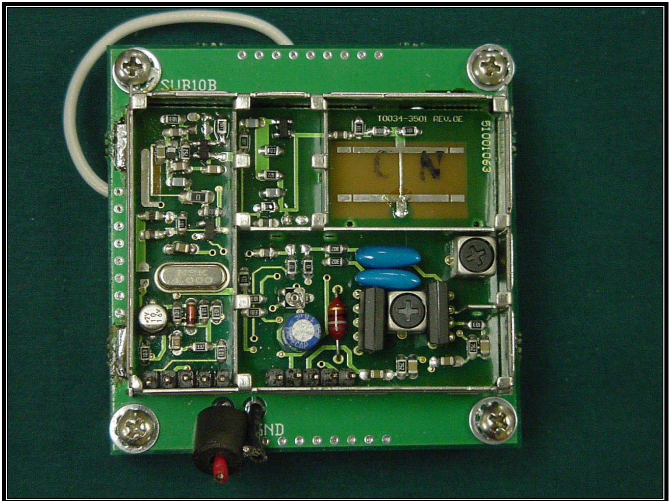
PHOTOGRAPH 10: PCB2 FRONT VIEW
