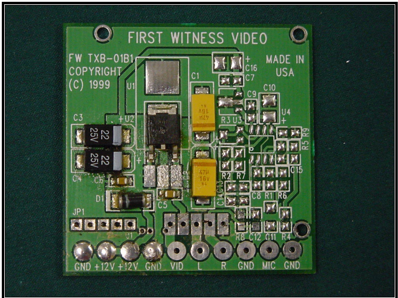
PHOTOGRAPH 12: PCB3 FRONT VIEW
