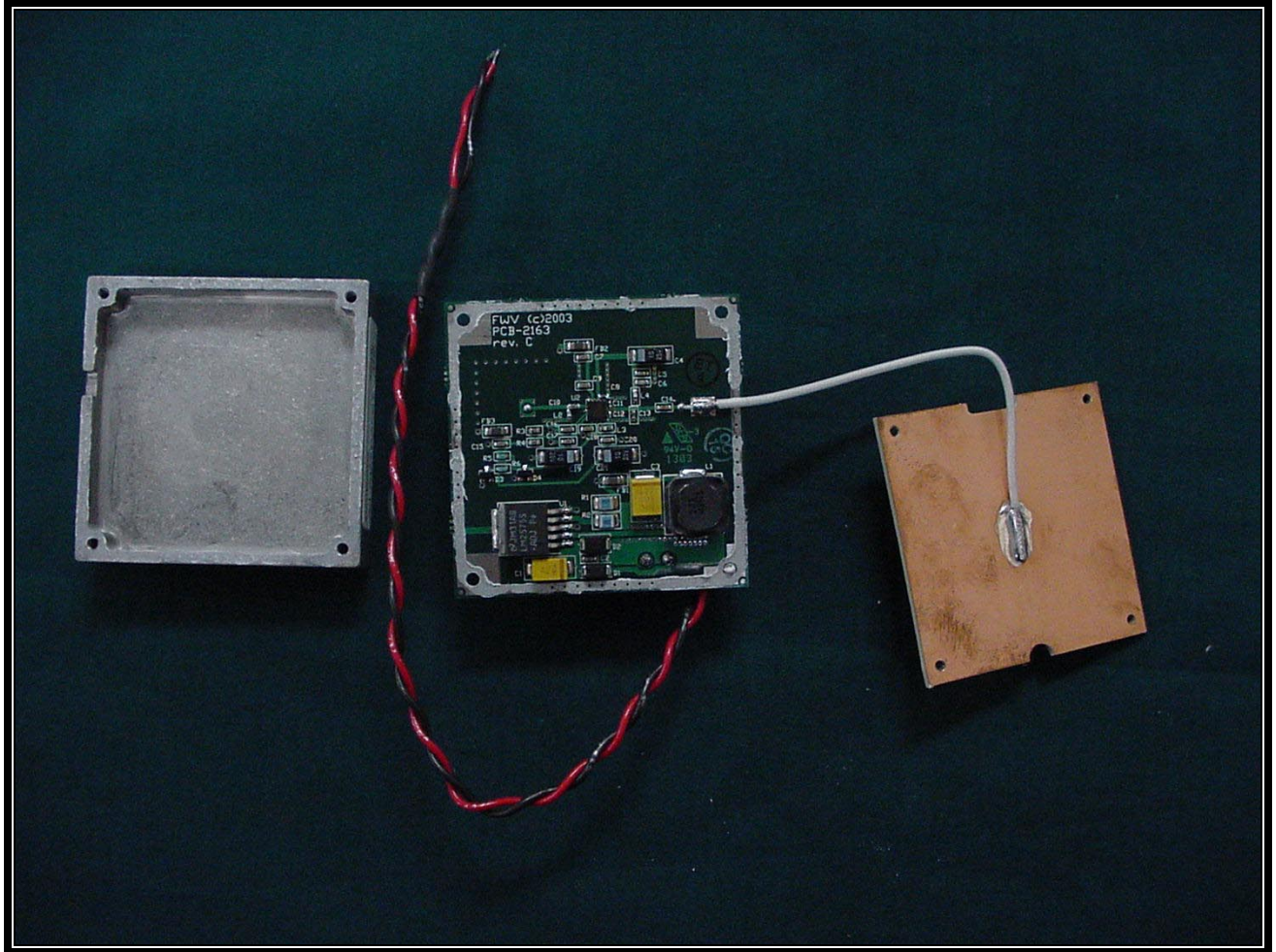
PHOTOGRAPH 7: OVERALL INTERNAL VIEW
