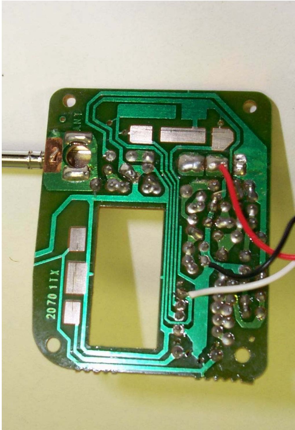
Foil Side
