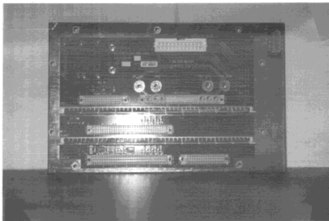
Figure 26, Backplane Board Top Side View CCA
