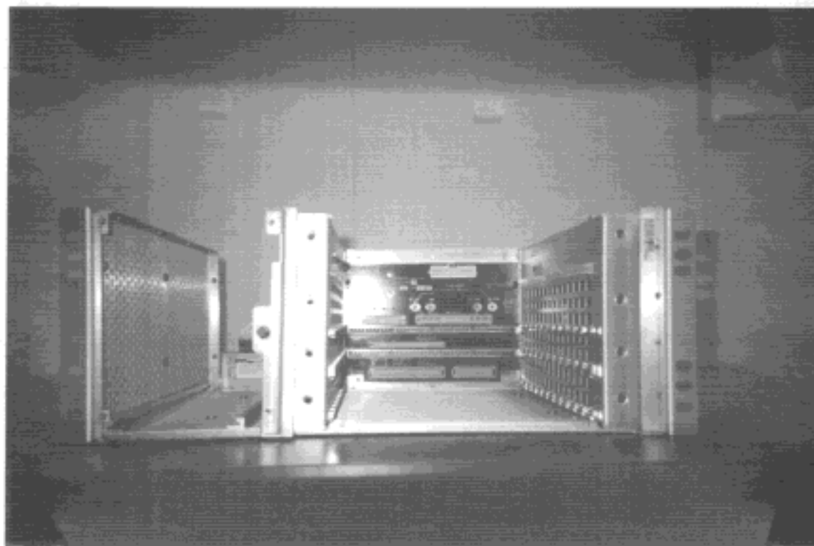
Figure 28, Backplane Board Installed Top Side View
