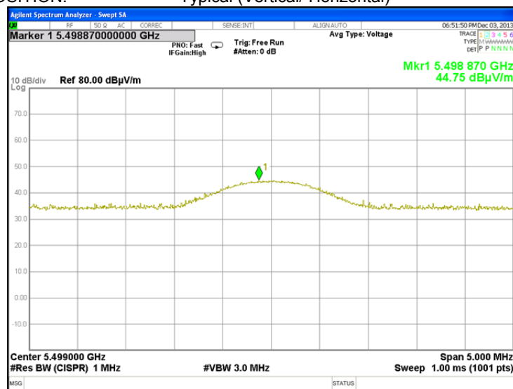
Plot 7.2.18 Radiated emission measurements at the sixth harmonic frequency
