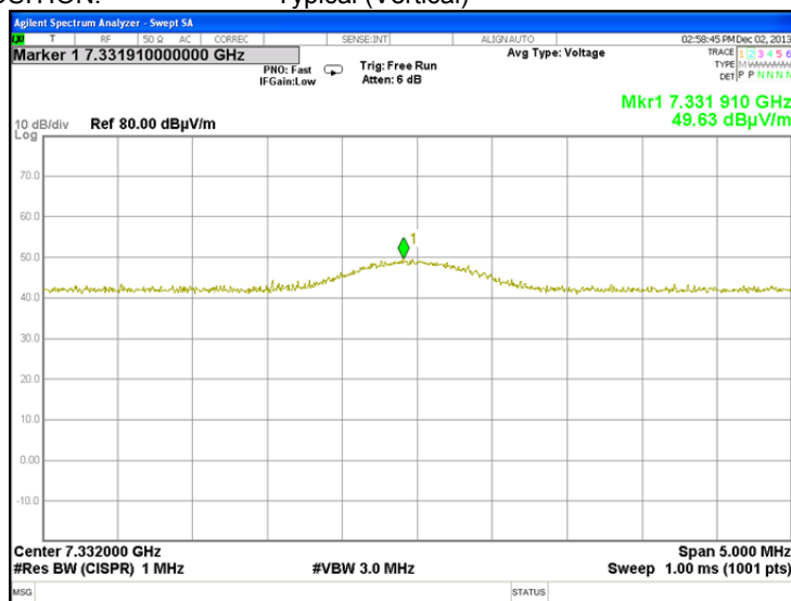
Plot 7.2.20 Radiated emission measurements at the eighth harmonic frequency
