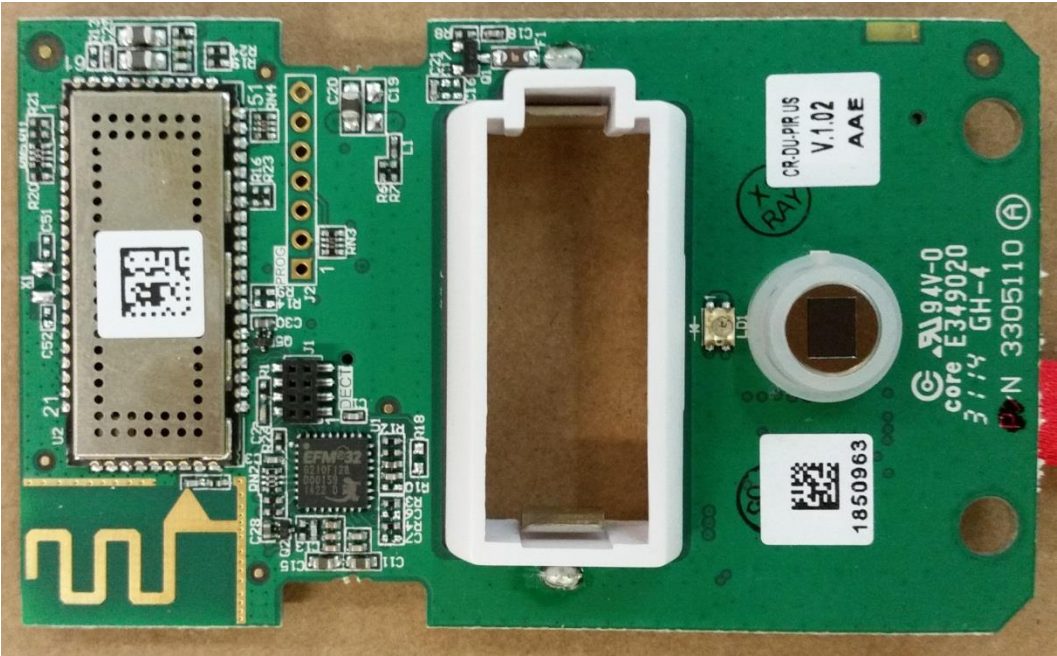
PCB Back Side:
