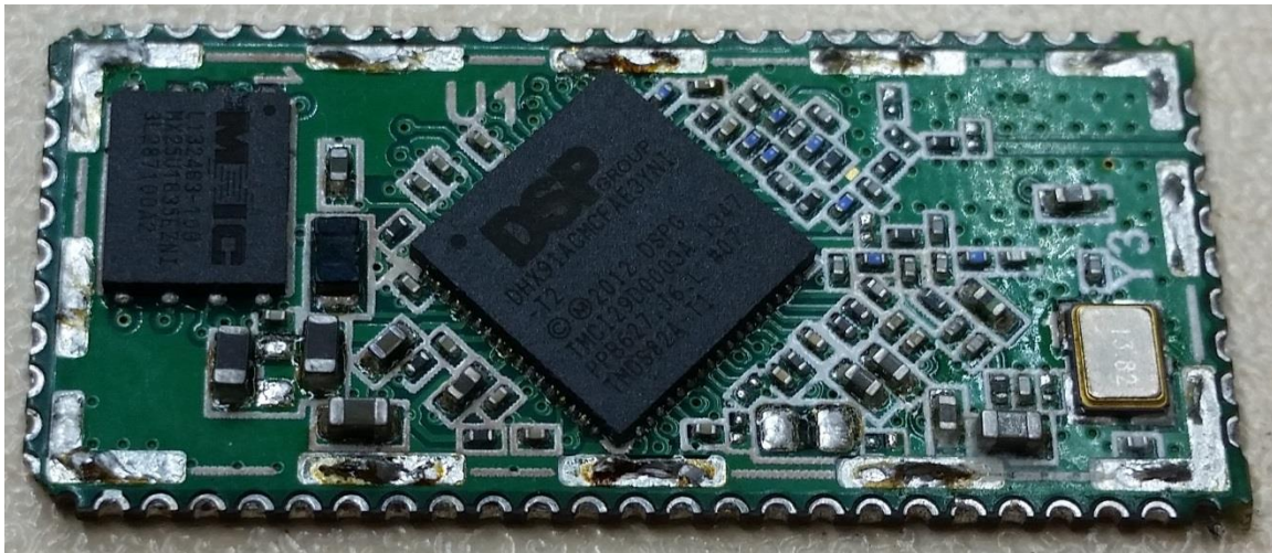
Top View, Radio Module, Front Side without Shield:
