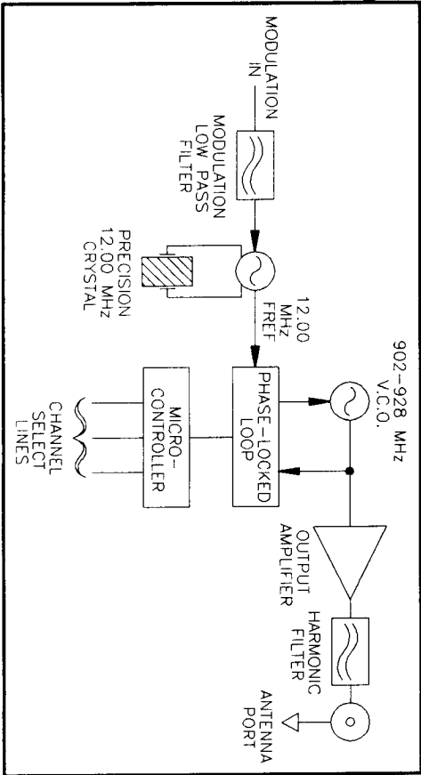
TXM-900-HP-II BLOCK DIAGRAM MODULE PURCHASED COMPLETE FROM LINX TECHNOLOGIES, GRANTS PASS, OR
