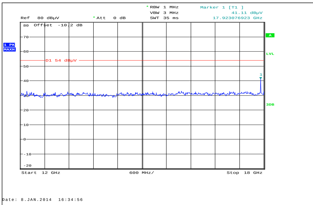
Plot 35: 12 GHz – 18 GHz, antenna horizontal / vertical, TX-Mode, low / mid / high frequency
