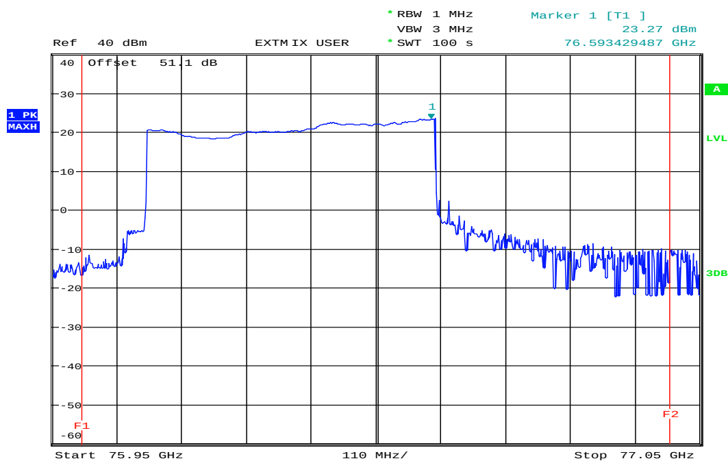
Plot 17: EIRP (Peak detector), T_{\max} / V_{\min} - V_{\max} , normal operation mode
