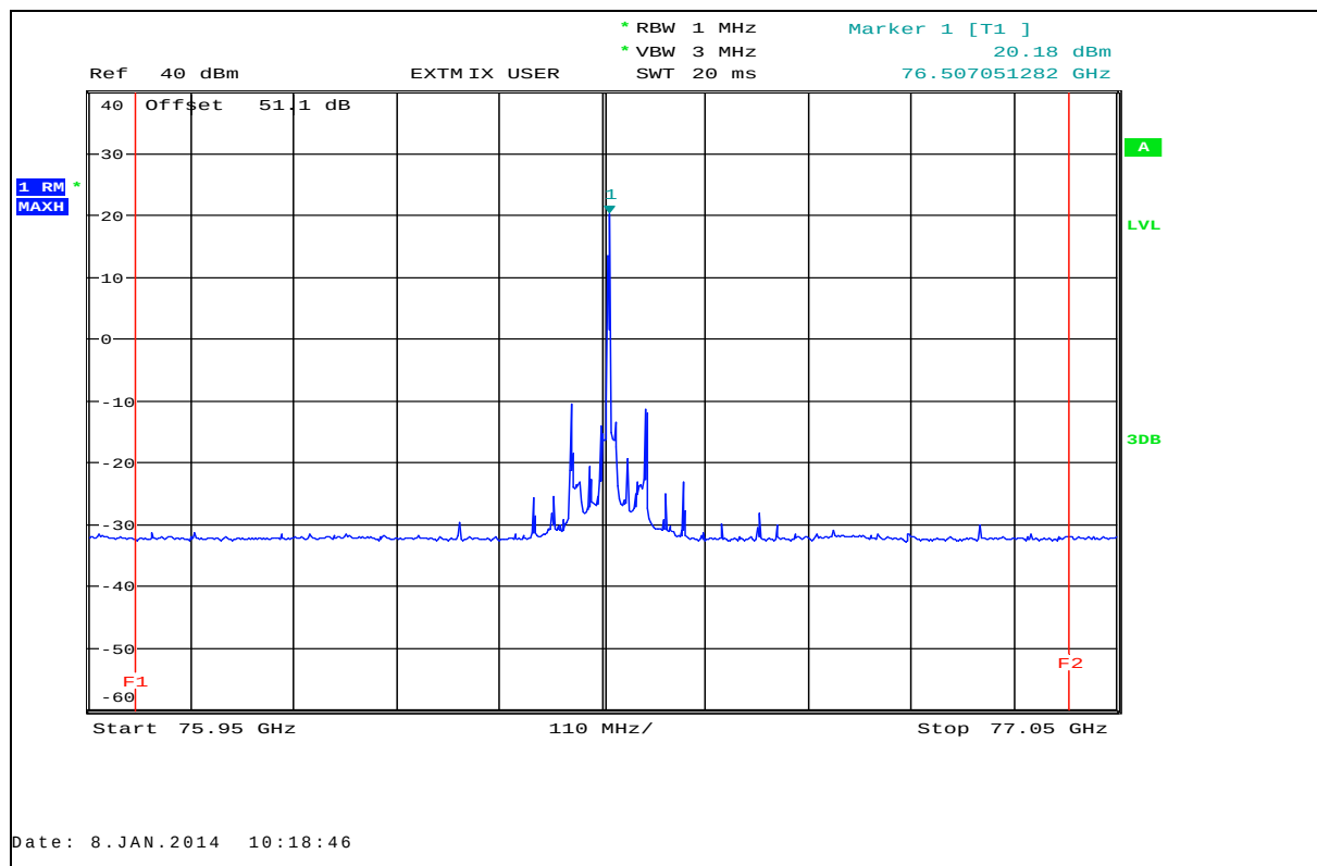
Plot 14: EIRP (RMS detector), T_{\min} / V_{\min} - V_{\max} , CW-Test mode, mid frequency
