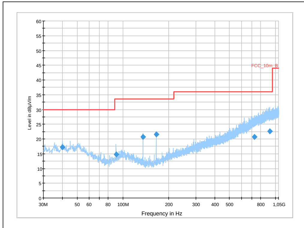
Plot 30: 30 MHz – 1 GHz, antenna horizontal / vertical, TX-Mode, middle frequency
