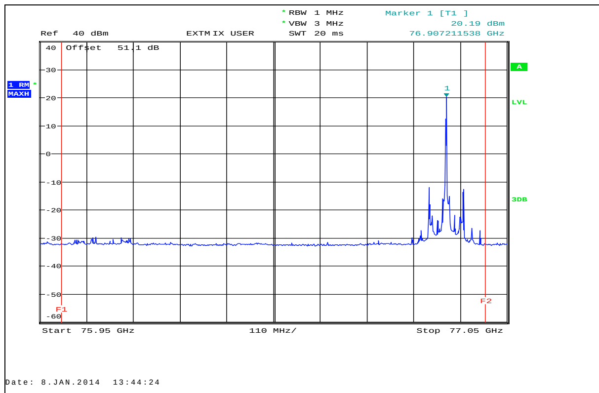
Plot 24: EIRP (RMS detector), T_{\max} / V_{\min} - V_{\max} , CW-Test mode, high frequency
