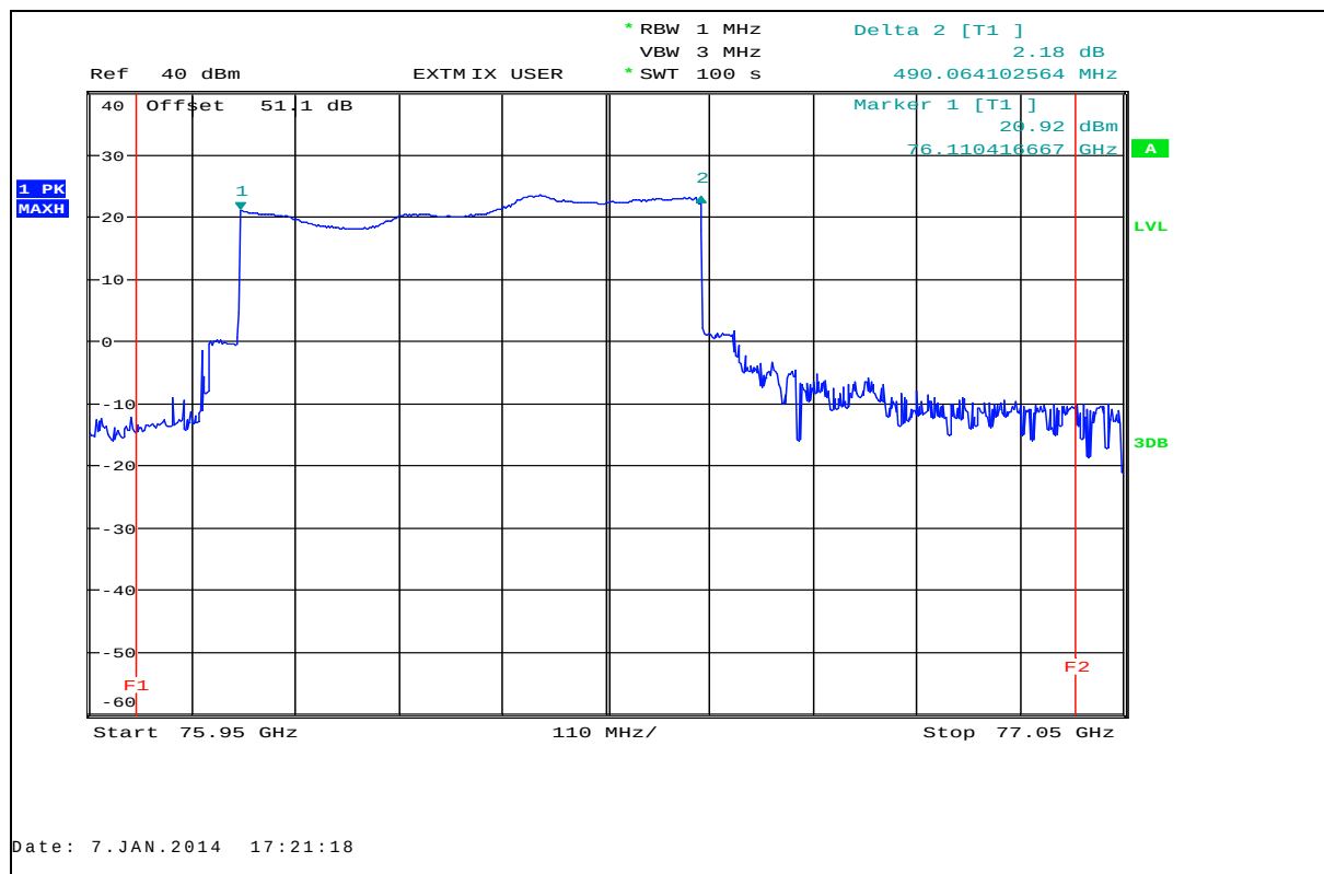
Plot 25: Occupied bandwidth (99%), T_{nom} / V_{nom} , normal operation mode
