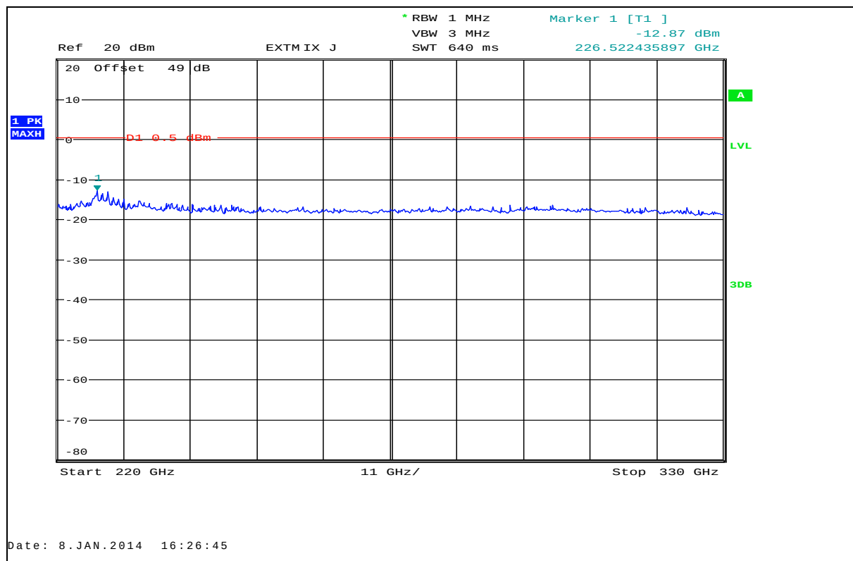
Plot 43: 220 GHz – 330 GHz, antenna horizontal / vertical, TX-Mode, low / mid / high frequency
