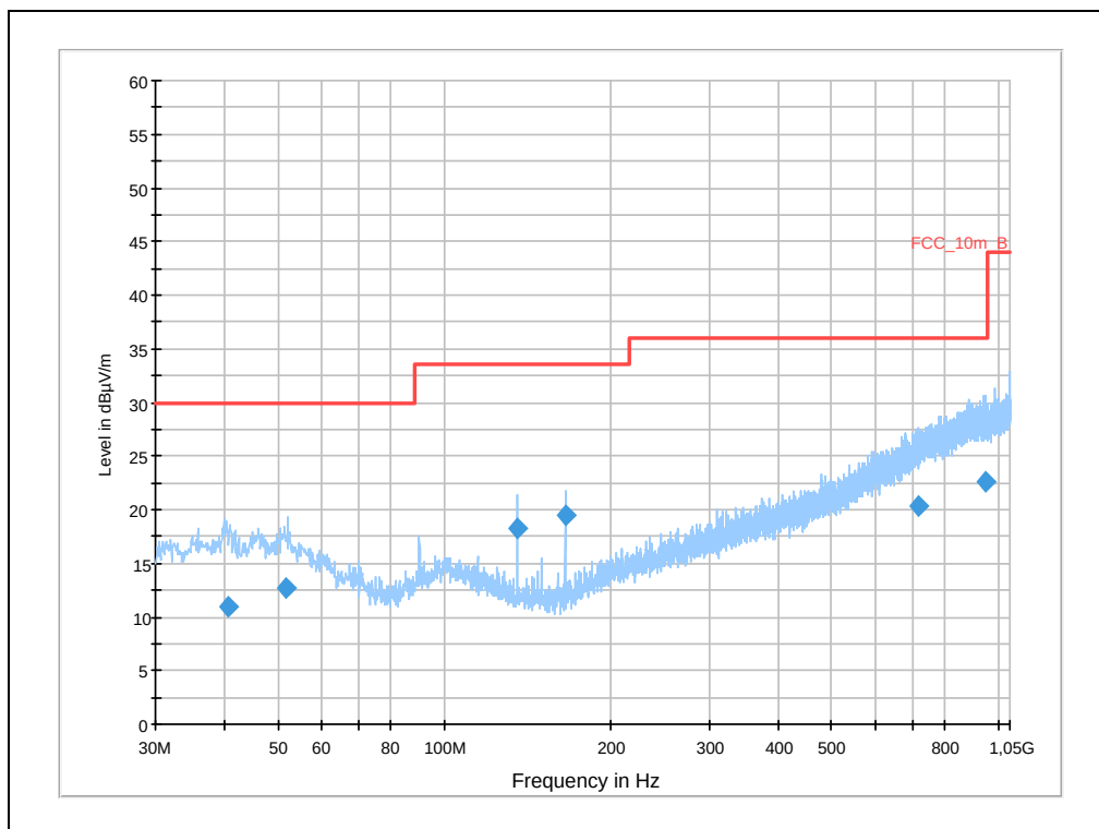
Plot 31: 30 MHz – 1 GHz, antenna horizontal / vertical, TX-Mode, high frequency
