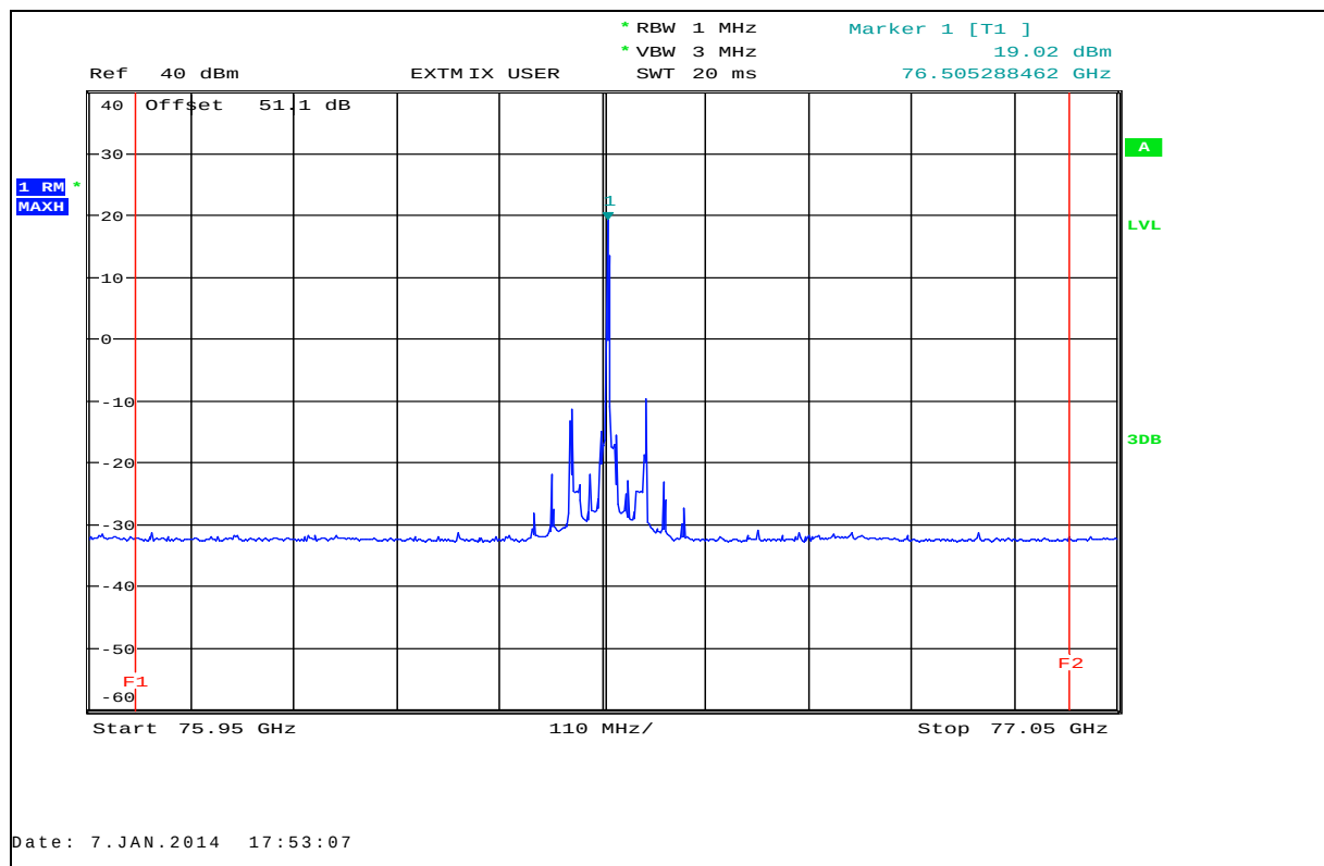
Plot 6: EIRP (RMS detector), T_{nom} / V_{nom} , CW-Test mode, mid frequency
