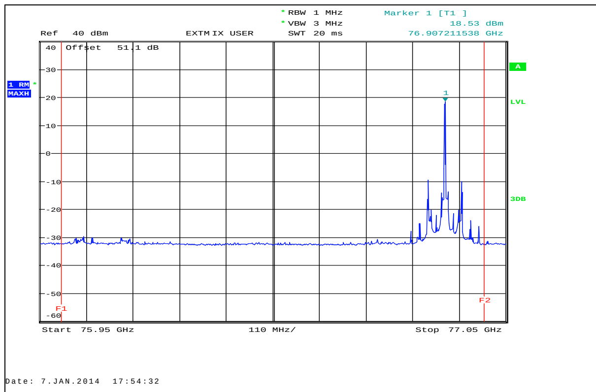
Plot 8: EIRP (RMS detector), T_{nom} / V_{nom} , CW-Test mode, high frequency
