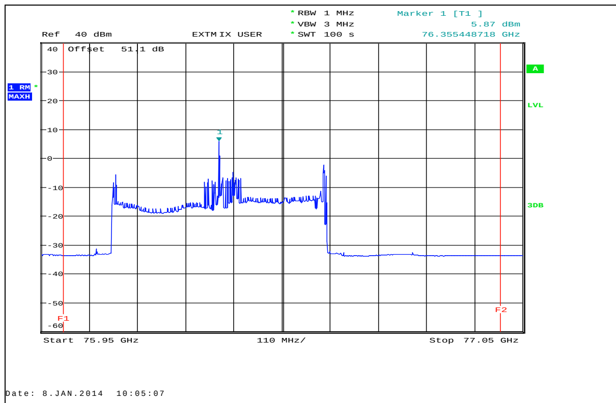
Plot 10: EIRP (RMS detector), T_{\min} / V_{\min} - V_{\max} , normal operation mode
