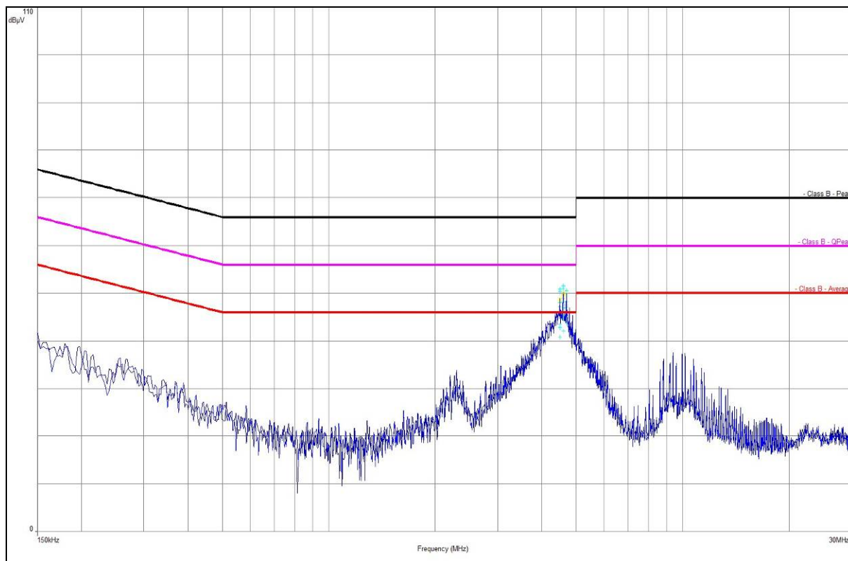
Plot 44: TX-Mode (valid for all frequencies)
