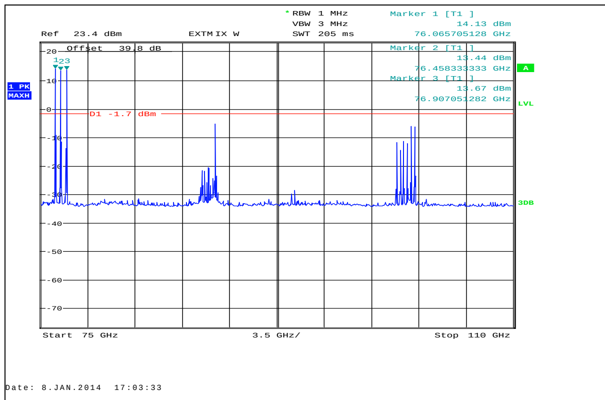
Plot 40: 75 GHz – 110 GHz, antenna horizontal / vertical, TX-Mode, low / mid / high frequency
