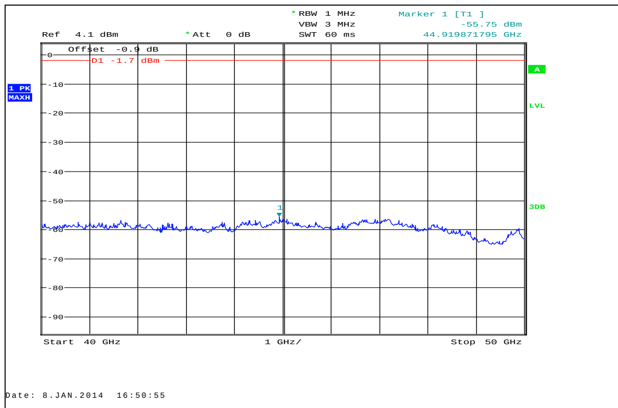
Plot 38: 40 GHz – 50 GHz, antenna horizontal / vertical, TX-Mode, low / mid / high frequency
