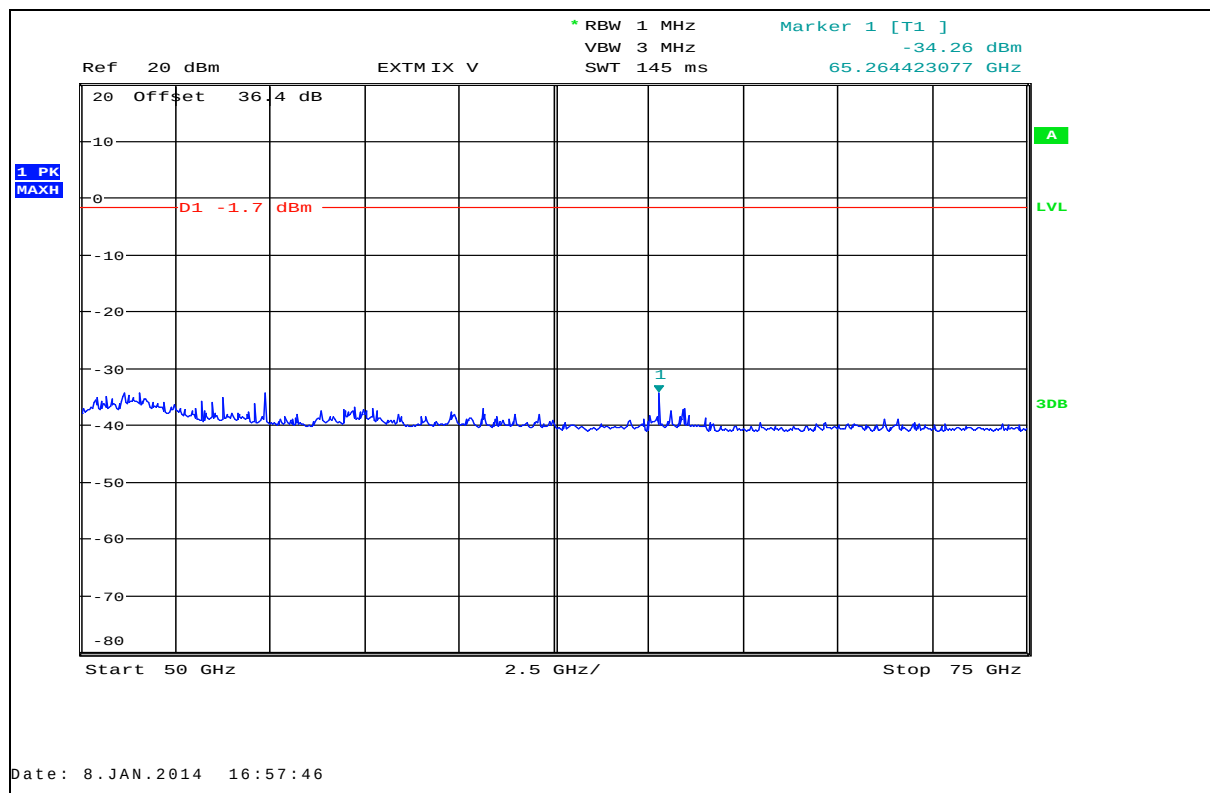
Plot 39: 50 GHz – 75 GHz, antenna horizontal / vertical, TX-Mode, low / mid / high frequency
