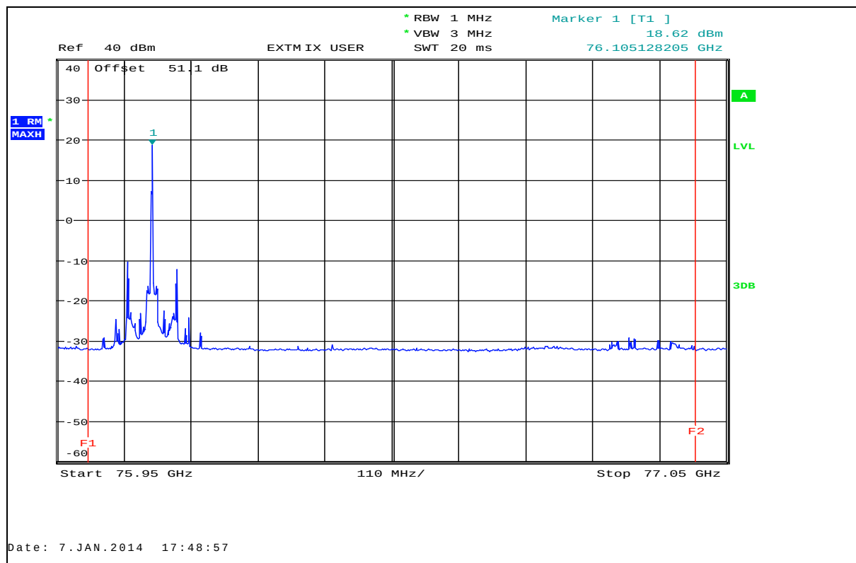
Plot 4: EIRP (RMS detector), T_{\text{nom}} / V_{\text{nom}} , CW-Test mode, low frequency
