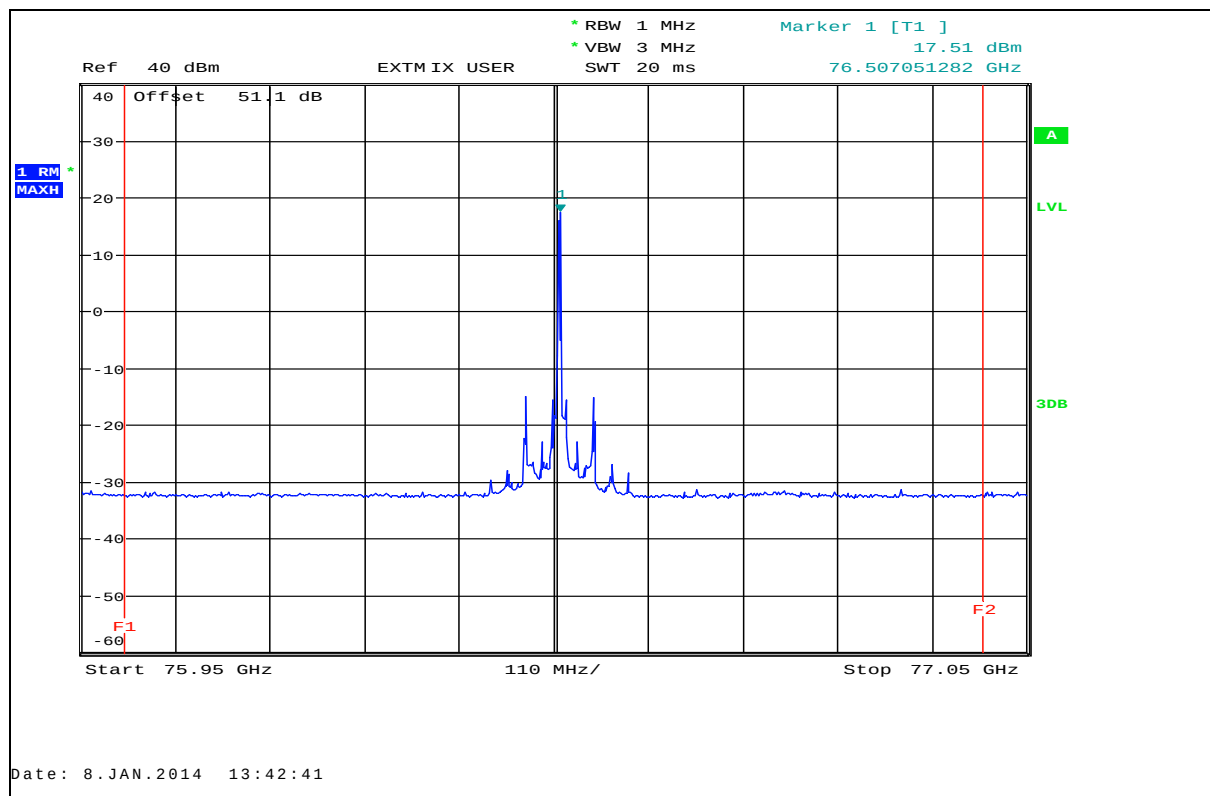
Plot 22: EIRP (RMS detector), T_{\max} / V_{\min} - V_{\max} , CW-Test mode, mid frequency
