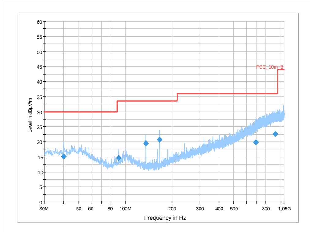
Plot 29: 30 MHz – 1 GHz, antenna horizontal / vertical, TX-Mode, low frequency
