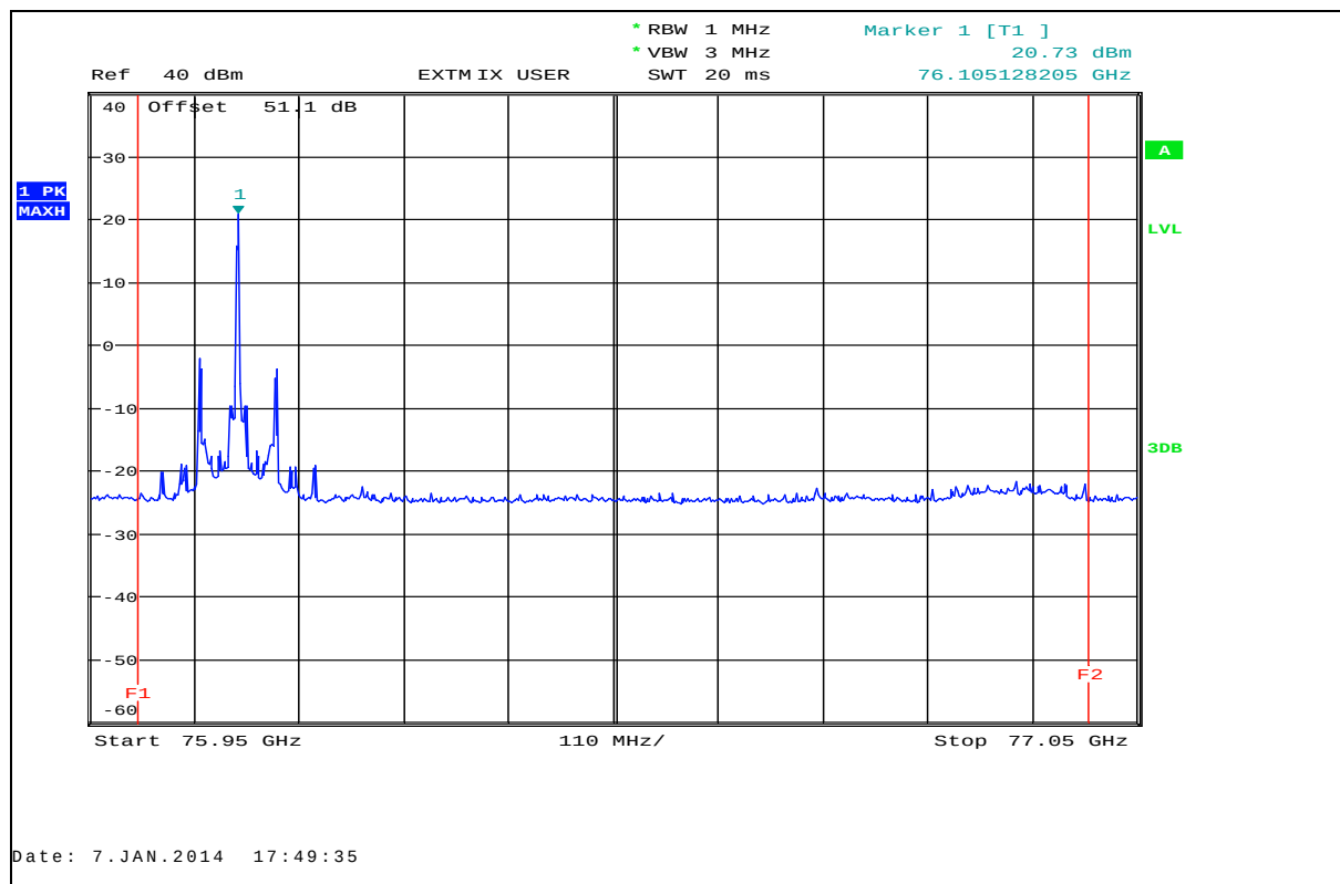
Plot 3: EIRP (Peak detector), T_{\text{nom}} / V_{\text{nom}} , CW-Test mode, low frequency
