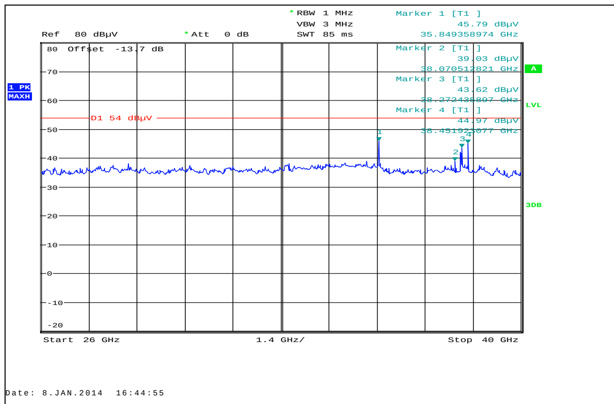
Plot 37: 26 GHz – 40 GHz, Pos-Peak, antenna horizontal / vertical, TX-Mode, low / mid / high frequency
