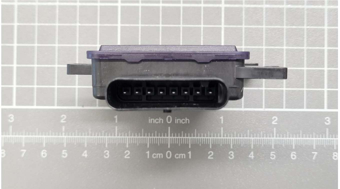
Photo No. 9: EUT with AK2-connector
