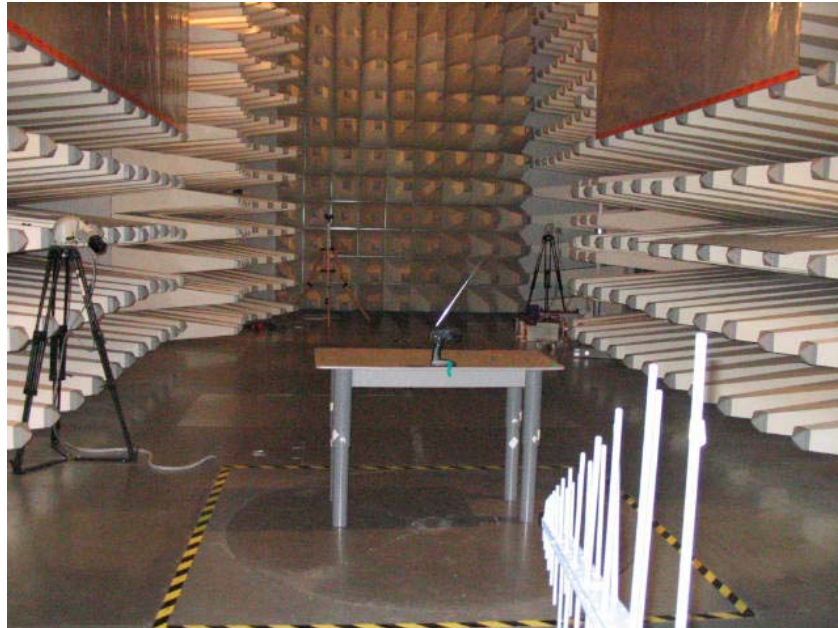
Set-up for Radiation Emission ( Receiver)
