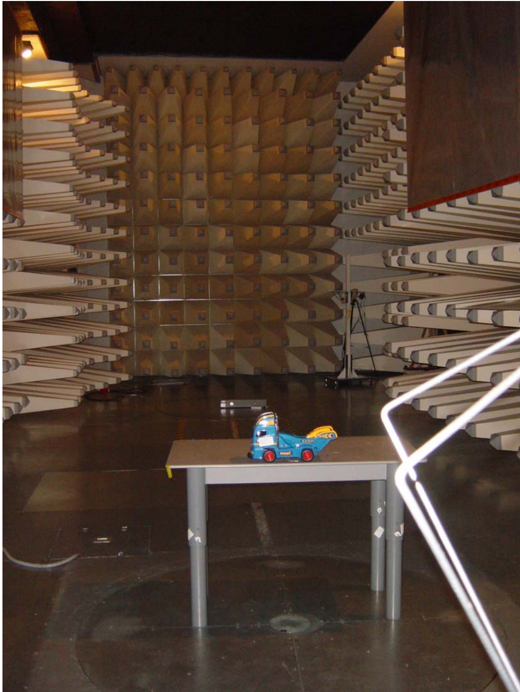
Set-up for Radiation Emission ( Receiver)
