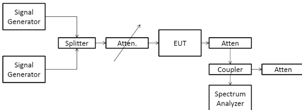
Figure 7.8.1 Spurious emission test setup
