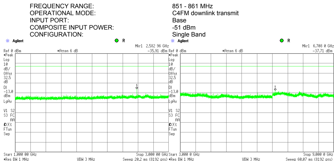
Plot 7.6.84 Spurious emission measurements in 1000 - 9000 MHz at high carrier frequency
