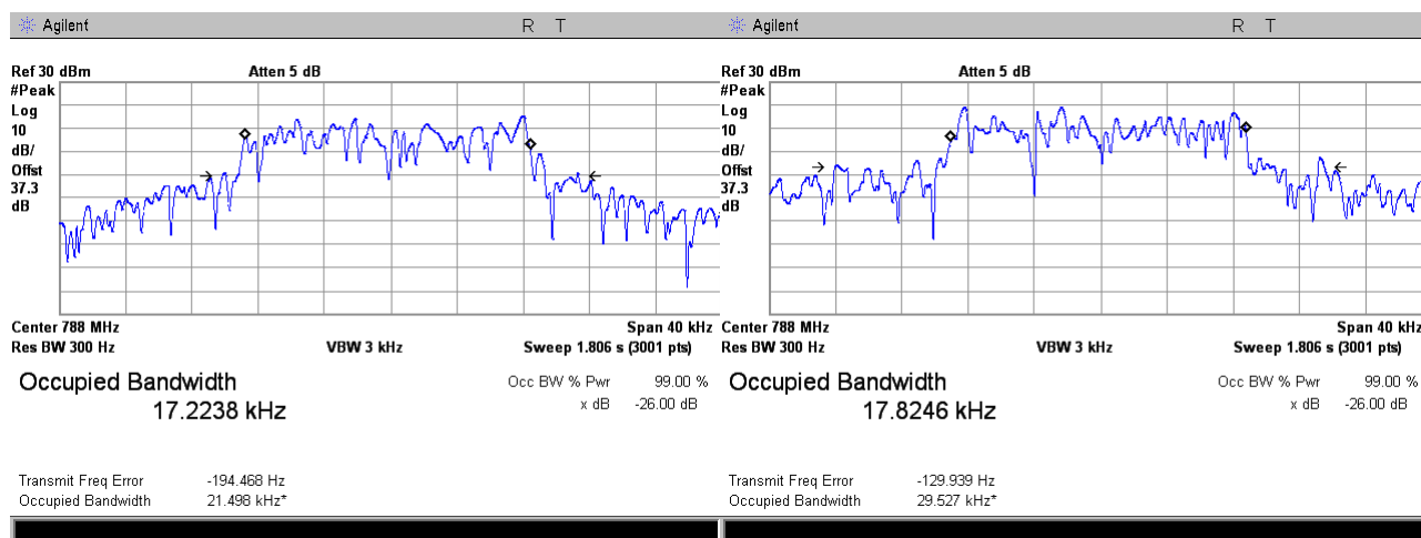
Plot 7.2.17 Occupied bandwidth test result at low frequency carrier, Port 2
