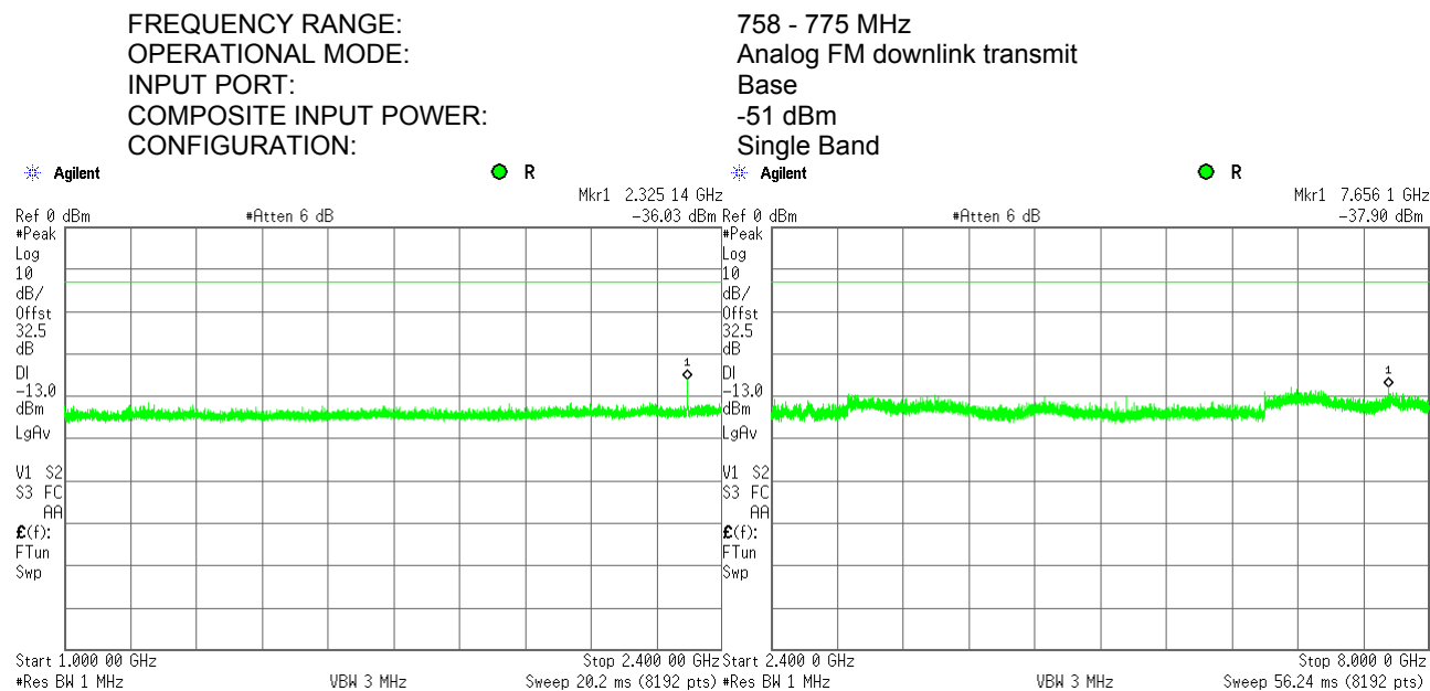
Plot 7.6.36 Spurious emission measurements in 1000 – 8000 MHz at high carrier frequency
