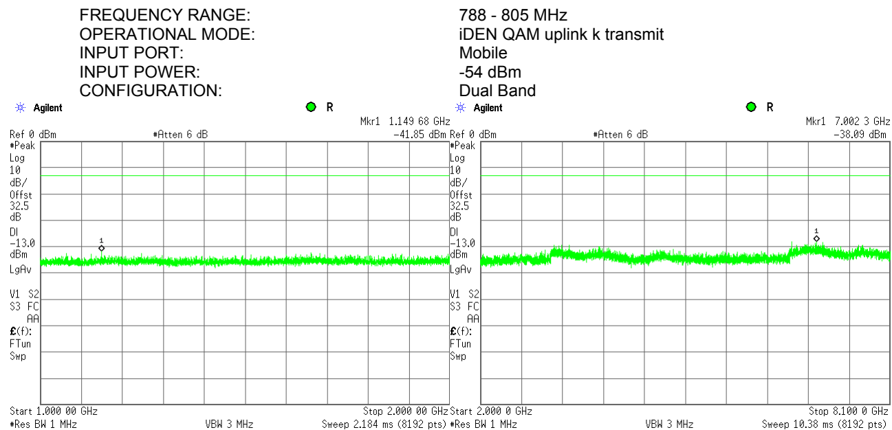
Plot 7.6.59 Spurious emission measurements in 1000 - 8100 MHz at mid carrier frequency
