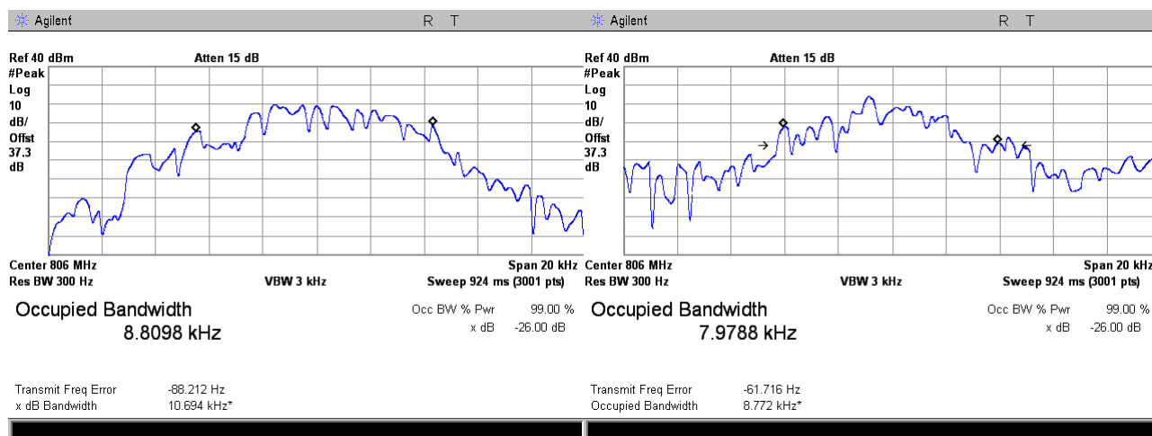
Plot 7.2.11 Occupied bandwidth test result at mid frequency carrier, Port 2
