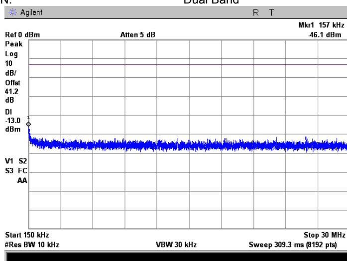
Plot 7.6.156 Spurious emission measurements in 0.15 - 30.0 MHz range at high carrier frequency
