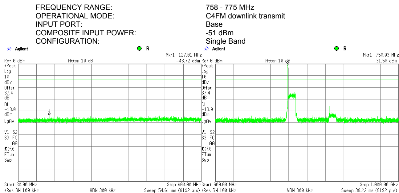
Plot 7.6.7 Spurious emission measurements in 30.0 - 1000 MHz range at low carrier frequency
