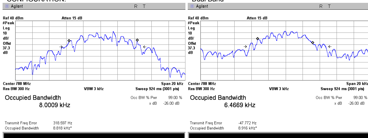
Plot 7.2.5 Occupied bandwidth test result at mid frequency carrier, Port 2
