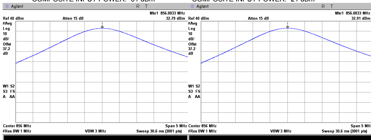
Plot 7.1.18 RF output power measurements at high frequency carrier, Port 1
