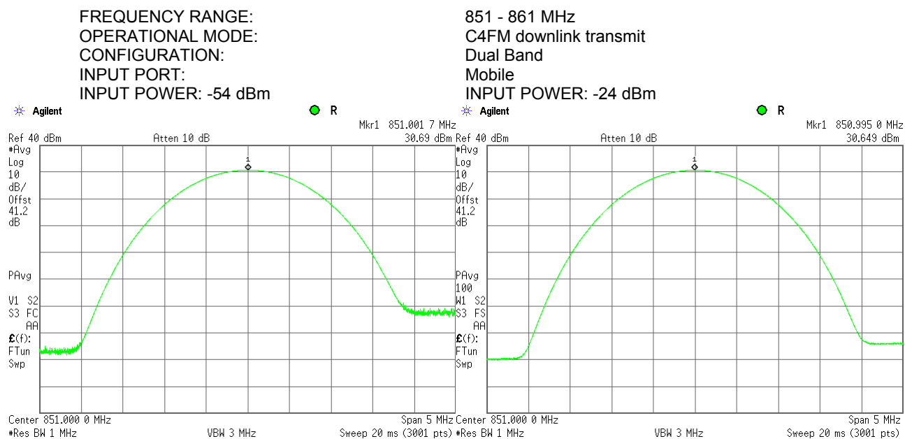
Plot 7.1.7 RF output power measurements at low frequency carrier, Port 1
