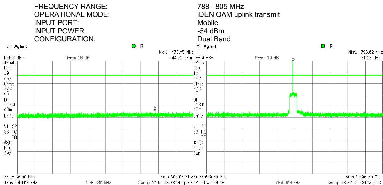
Plot 7.6.56 Spurious emission measurements in 30.0 - 1000 MHz range at mid carrier frequency
