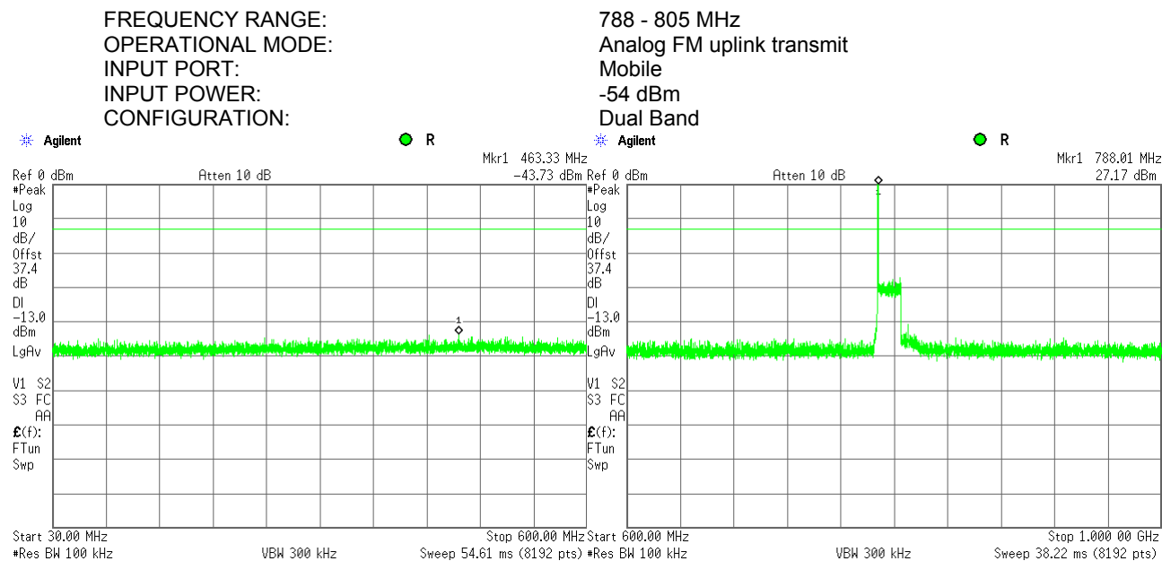
Plot 7.6.68 Spurious emission measurements in 30.0 - 1000 MHz range at mid carrier frequency
