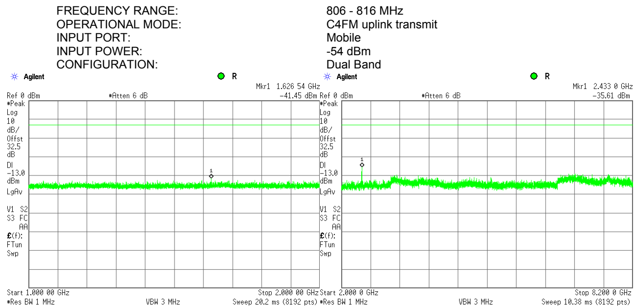
Plot 7.6.120 Spurious emission measurements in 1000 - 8200 MHz at high carrier frequency
