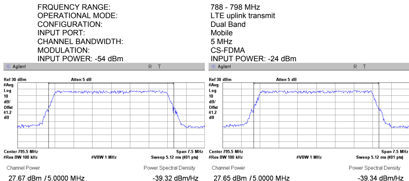
Plot 7.1.60 RF output power measurements at high frequency carrier, Port 2
