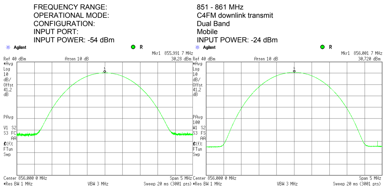
Plot 7.1.8 RF output power measurements at mid frequency carrier, Port 1
