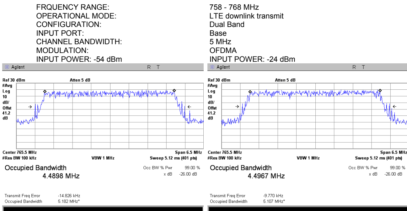
Plot 7.2.38 Occupied bandwidth test result at high frequency carrier, Port 1
