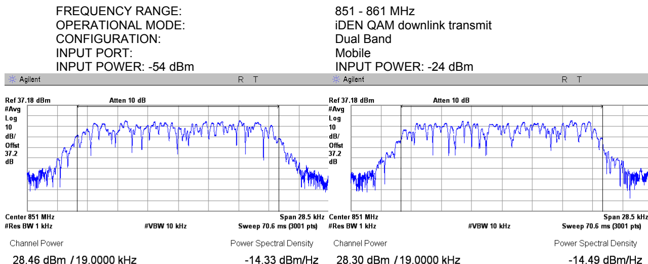
Plot 7.1.25 RF output power measurements at low frequency carrier, Port 1
