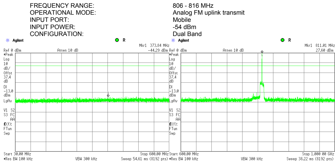
Plot 7.6.140 Spurious emission measurements in 30.0 - 1000 MHz range at mid carrier frequency
