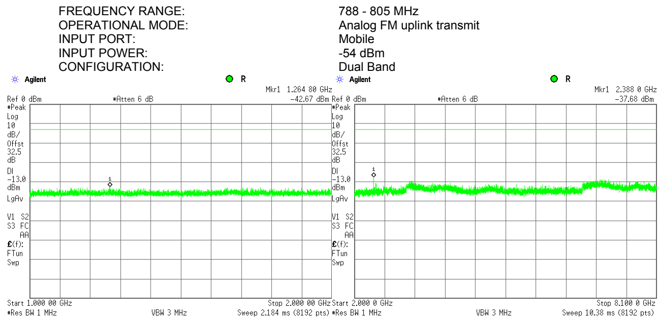
Plot 7.6.72 Spurious emission measurements in 1000 - 8100 MHz at high carrier frequency
