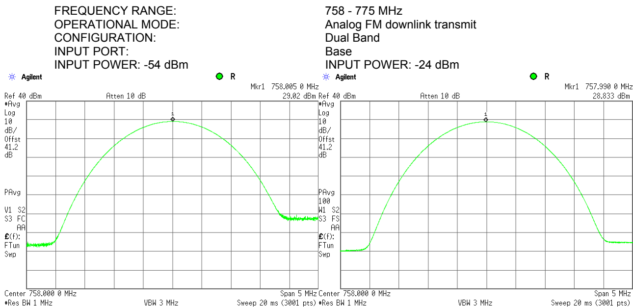
Plot 7.1.37 RF output power measurements at low frequency carrier, Port 1
