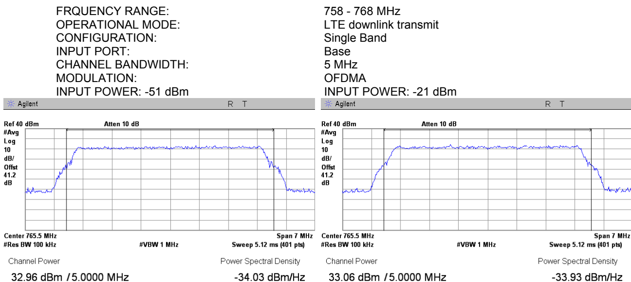
Plot 7.1.58 RF output power measurements at high frequency carrier, Port 1
