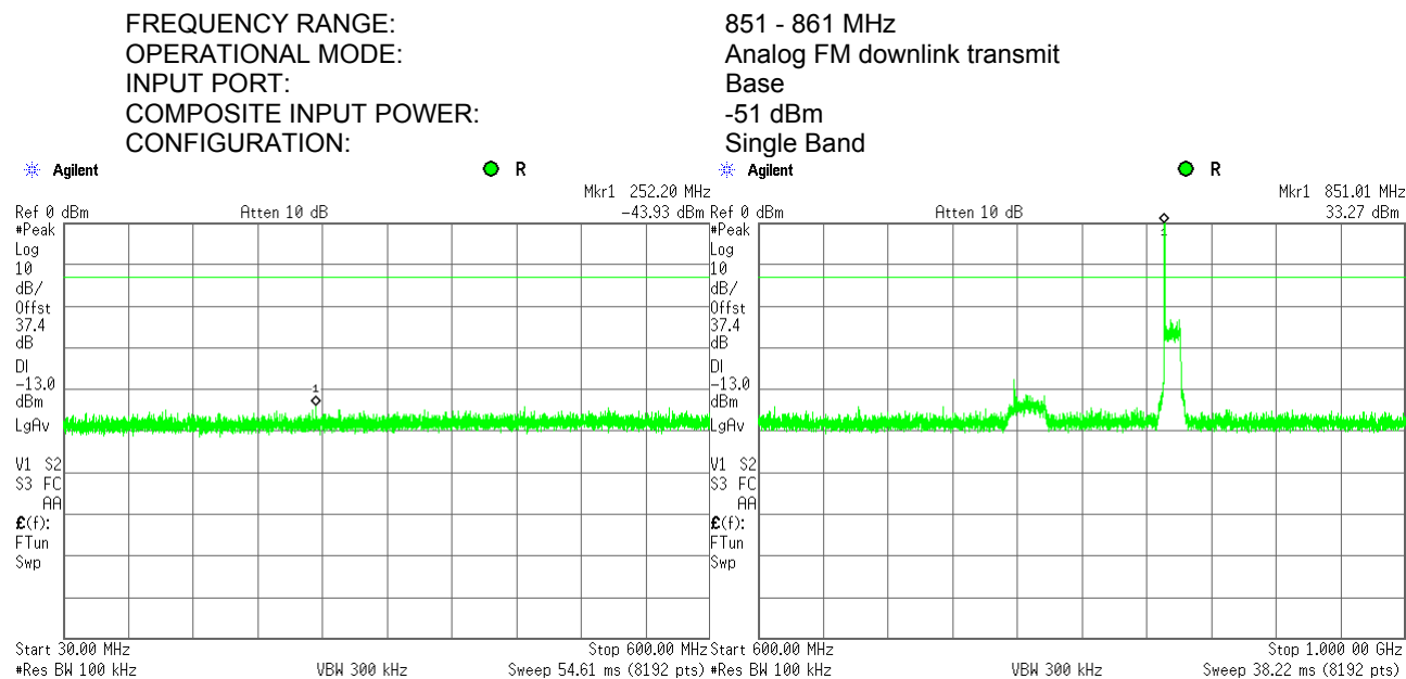
Plot 7.6.104 Spurious emission measurements in 30.0 - 1000 MHz range at mid carrier frequency
