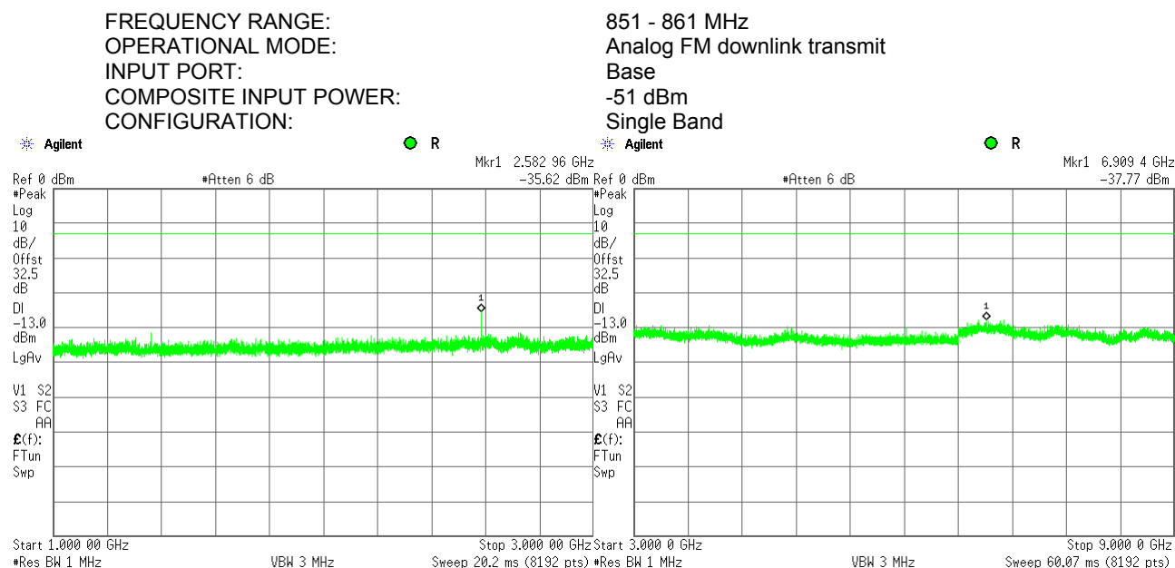
Plot 7.6.108 Spurious emission measurements in 1000 - 9000 MHz at high carrier frequency
