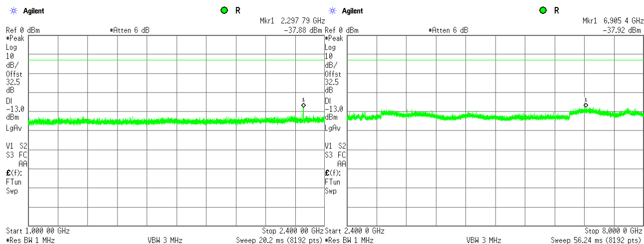
Plot 7.6.12 Spurious emission measurements in 1000 - 8000 MHz at high carrier frequency
