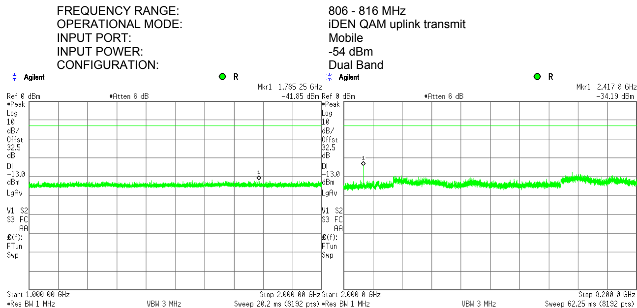
Plot 7.6.130 Spurious emission measurements in 1000 - 8200 MHz range at low carrier frequency
