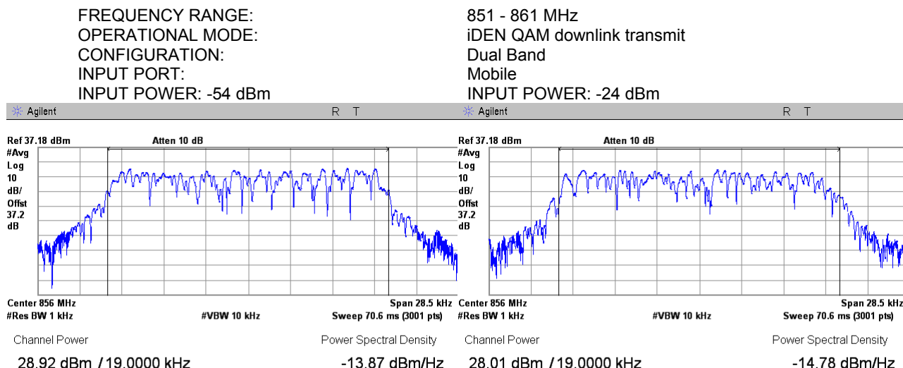
Plot 7.1.26 RF output power measurements at mid frequency carrier, Port 1
