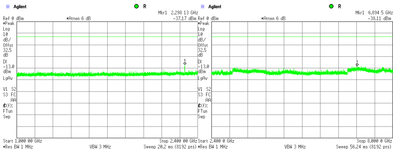
Plot 7.6.24 Spurious emission measurements in 1000 - 8000 MHz at high carrier frequency
