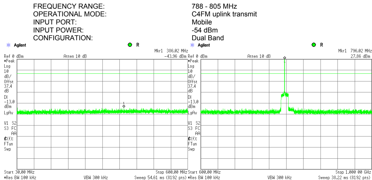
Plot 7.6.44 Spurious emission measurements in 30.0 - 1000 MHz range at mid carrier frequency
