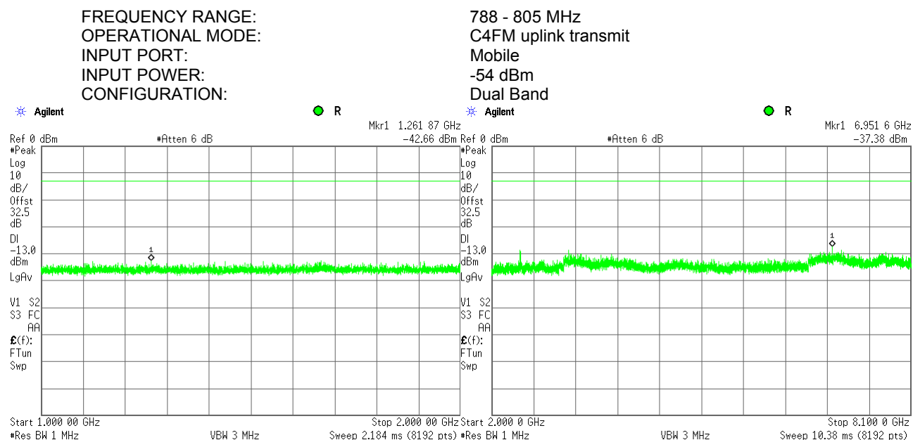
Plot 7.6.48 Spurious emission measurements in 1000 - 8100 MHz at high carrier frequency
