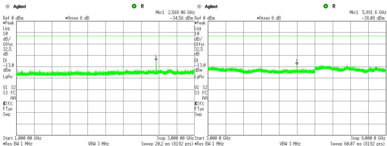
Plot 7.6.96 Spurious emission measurements in 1000 - 9000 MHz at high carrier frequency
