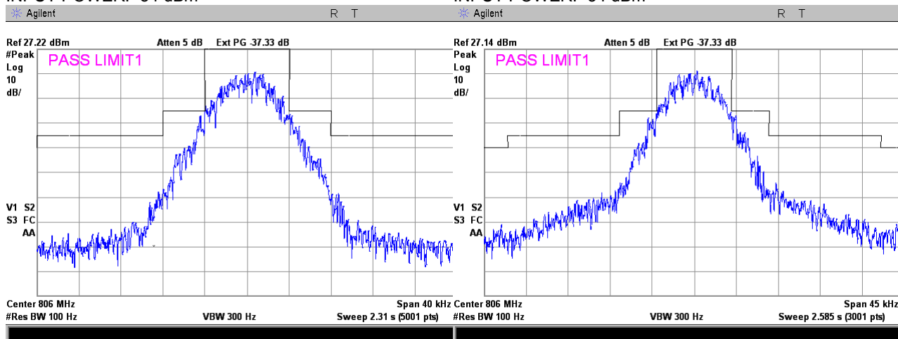
Plot 7.3.23 Occupied bandwidth test result at mid frequency carrier, Port 2
