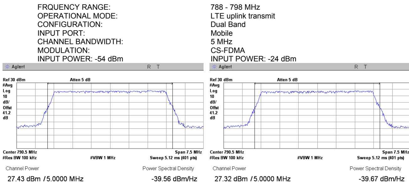
Plot 7.1.59 RF output power measurements at low frequency carrier, Port 2
