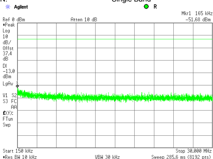
Plot 7.6.102 Spurious emission measurements in 0.15 - 30.0 MHz range at high carrier frequency
