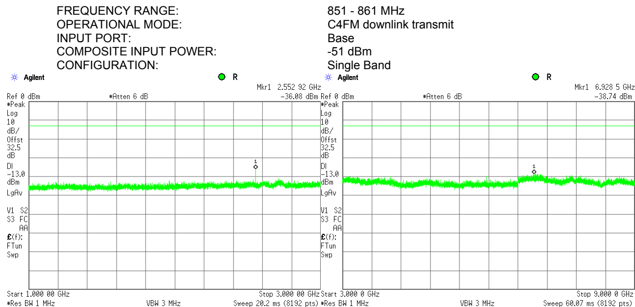
Plot 7.6.82 Spurious emission measurements in 1000 - 9000 MHz range at low carrier frequency
