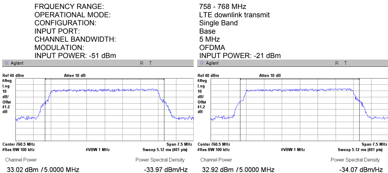
Plot 7.1.57 RF output power measurements at low frequency carrier, Port 1
