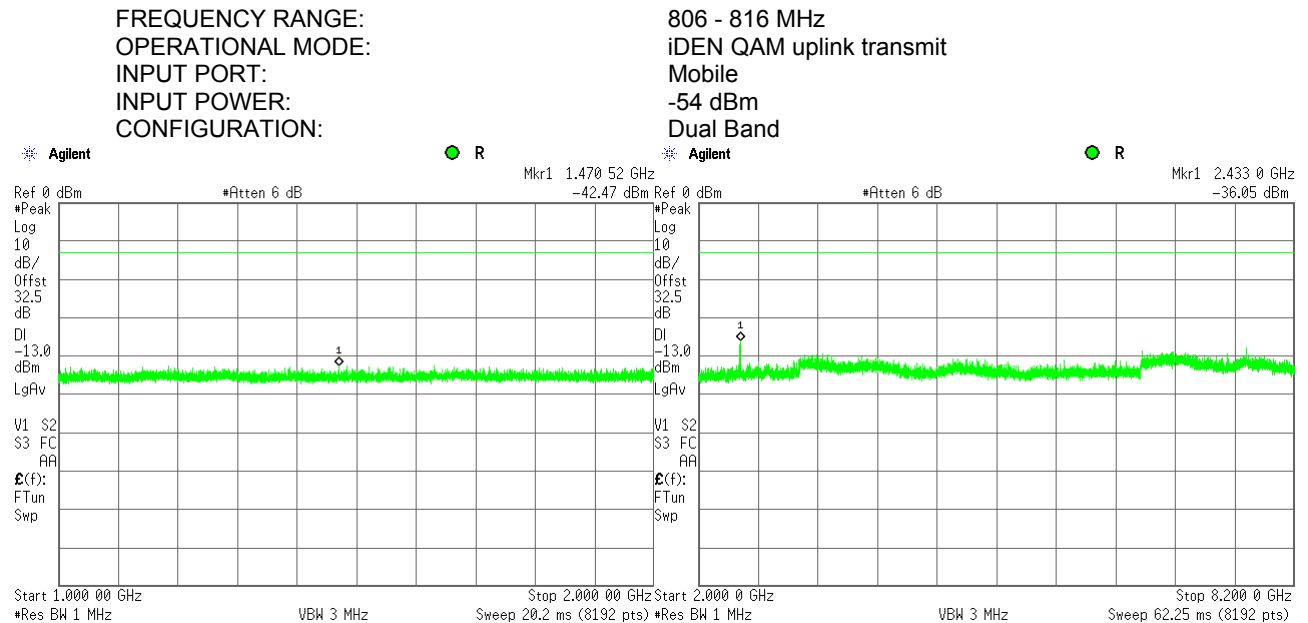
Plot 7.6.132 Spurious emission measurements in 1000 - 8200 MHz at high carrier frequency
