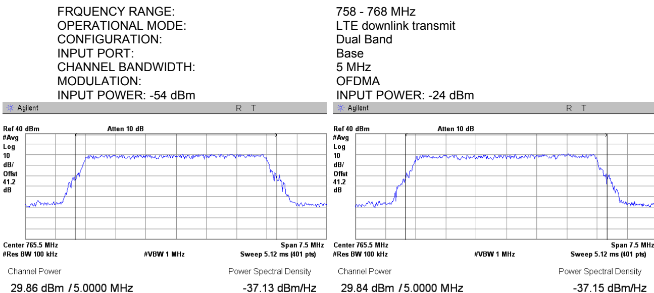
Plot 7.1.56 RF output power measurements at high frequency carrier, Port 1
