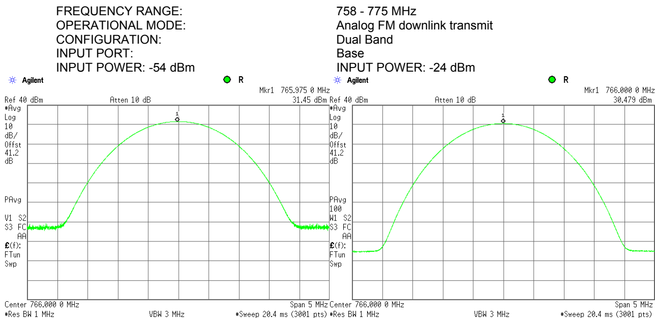
Plot 7.1.38 RF output power measurements at mid frequency carrier, Port 1
