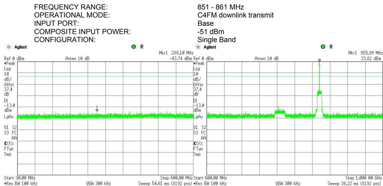
Plot 7.6.80 Spurious emission measurements in 30.0 - 1000 MHz range at mid carrier frequency
