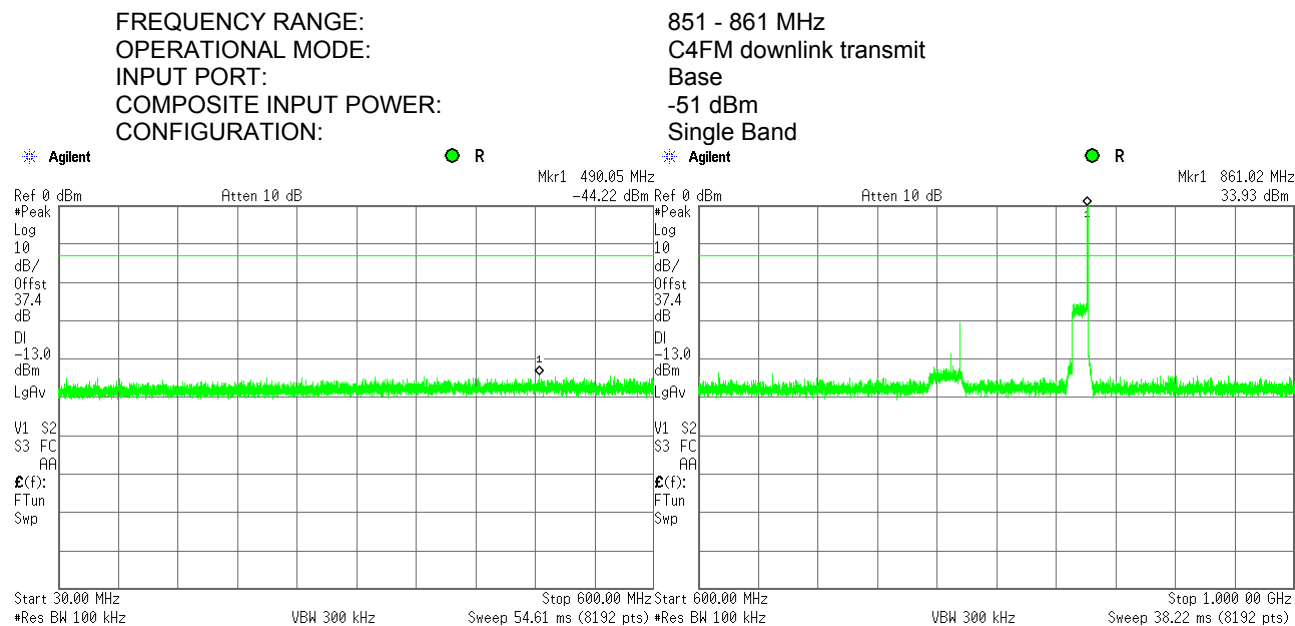
Plot 7.6.81 Spurious emission measurements in 30.0 - 1000 MHz range at high carrier frequency
