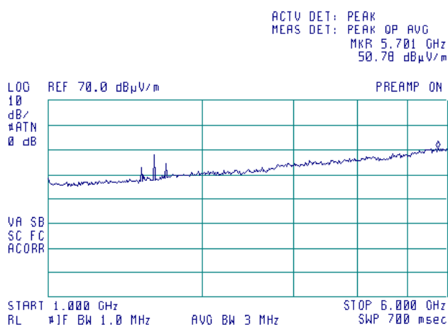
Plot 7.5.5 Radiated emission measurements in 1000 – 6000 MHz range
