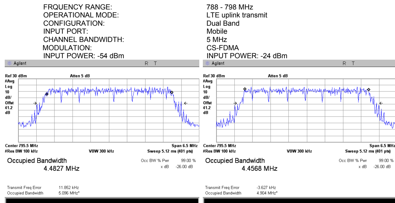
Plot 7.2.42 Occupied bandwidth test result at high frequency carrier, Port 2
