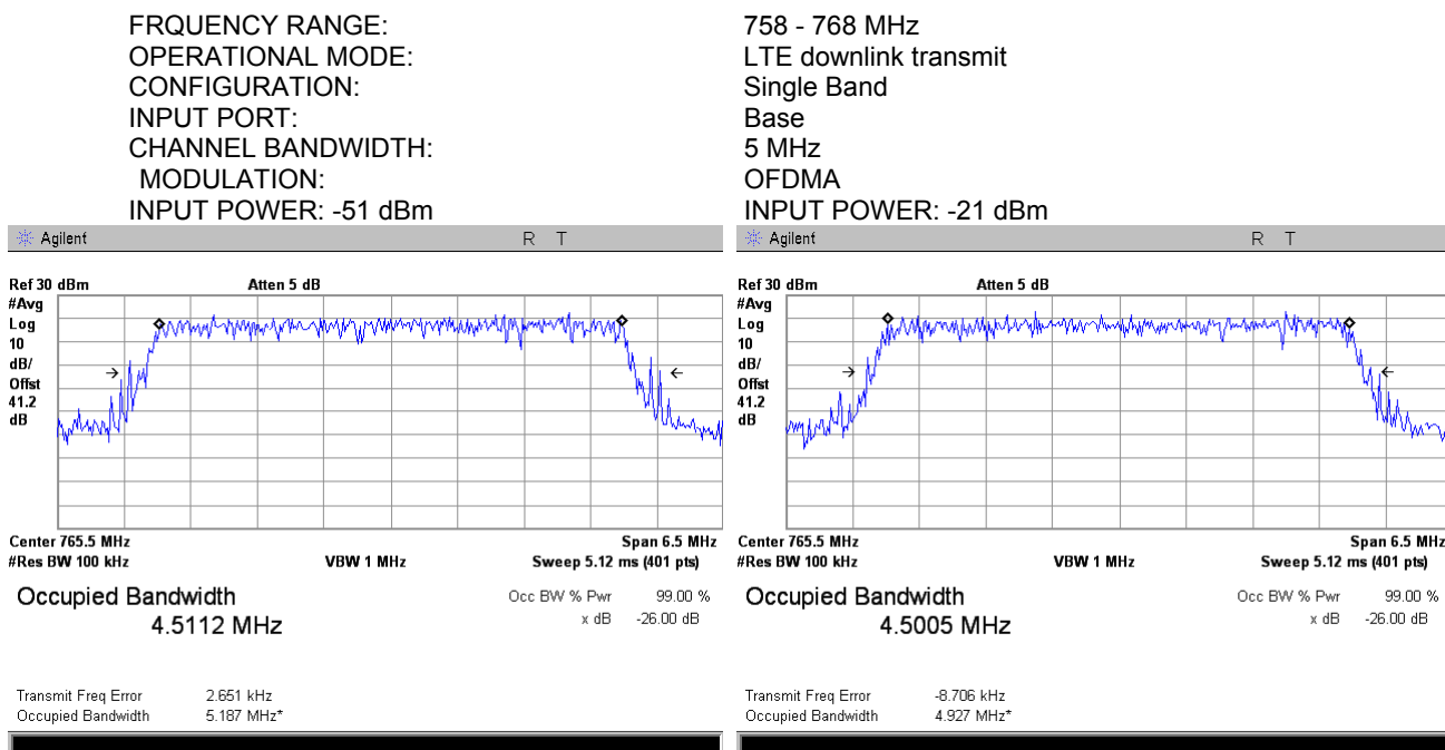
Plot 7.2.40 Occupied bandwidth test result at high frequency carrier, Port 1
