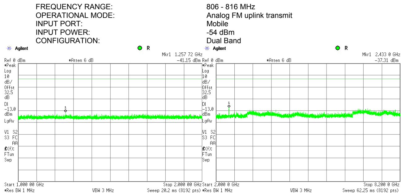
Plot 7.6.144 Spurious emission measurements in 1000 - 8200 MHz at high carrier frequency
