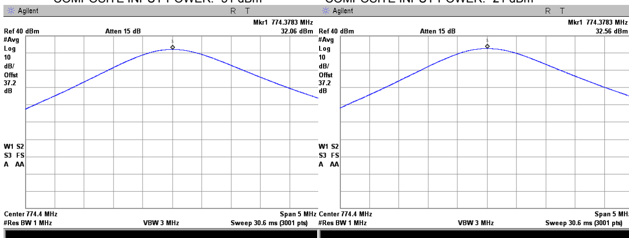
Plot 7.1.16 RF output power measurements at low frequency carrier, Port 1
