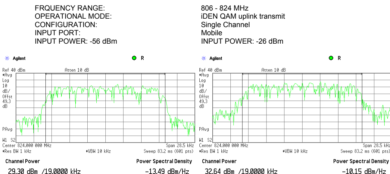
Plot 7.1.24 RF output power measurements at high frequency carrier, Port 2
