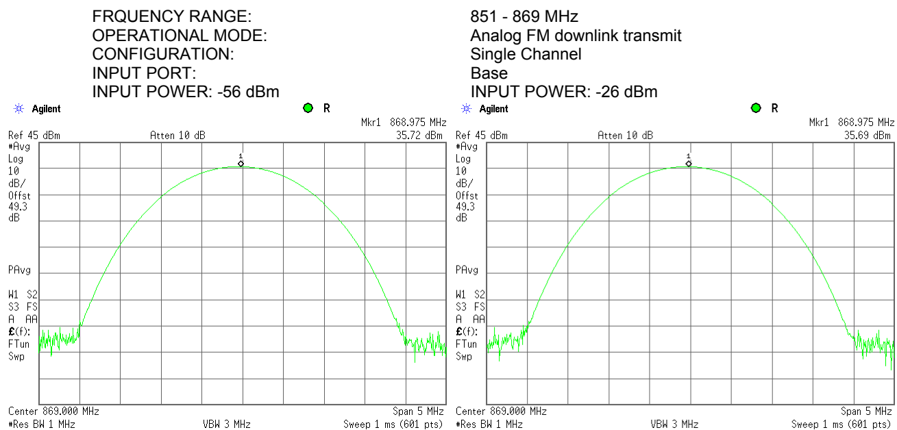
Plot 7.1.33 RF output power measurements at high frequency carrier, Port 1
