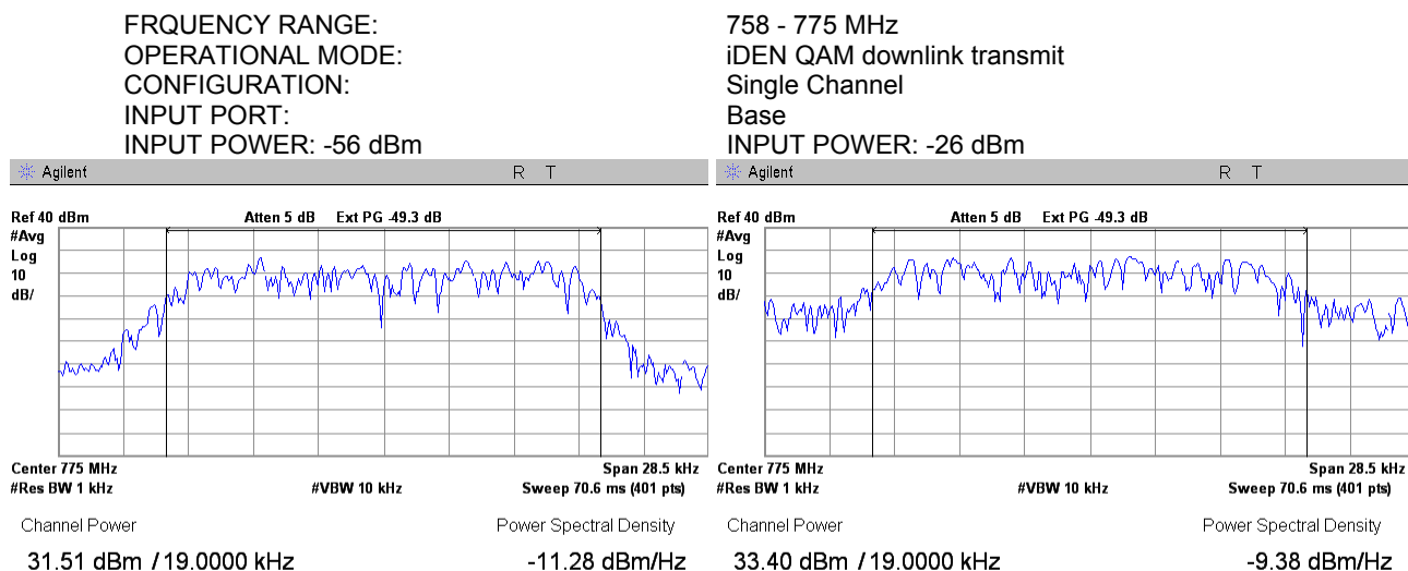
Plot 7.1.15 RF output power measurements at high frequency carrier, Port 1
