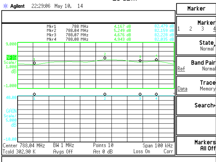
Plot 7.7.8 Noise figure test results at mid frequency
