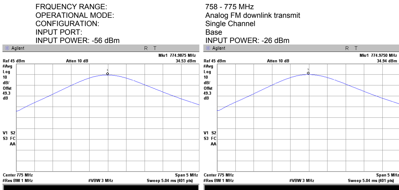
Plot 7.1.27 RF output power measurements at high frequency carrier, Port 1
