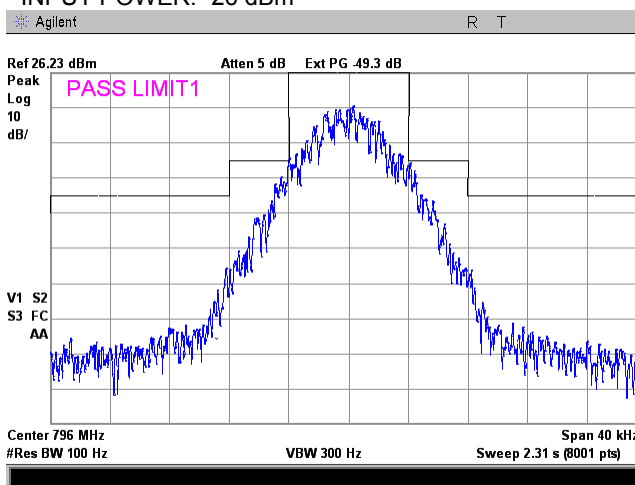
Plot 7.3.18 Emission mask test result at high frequency carrier, Port 2
