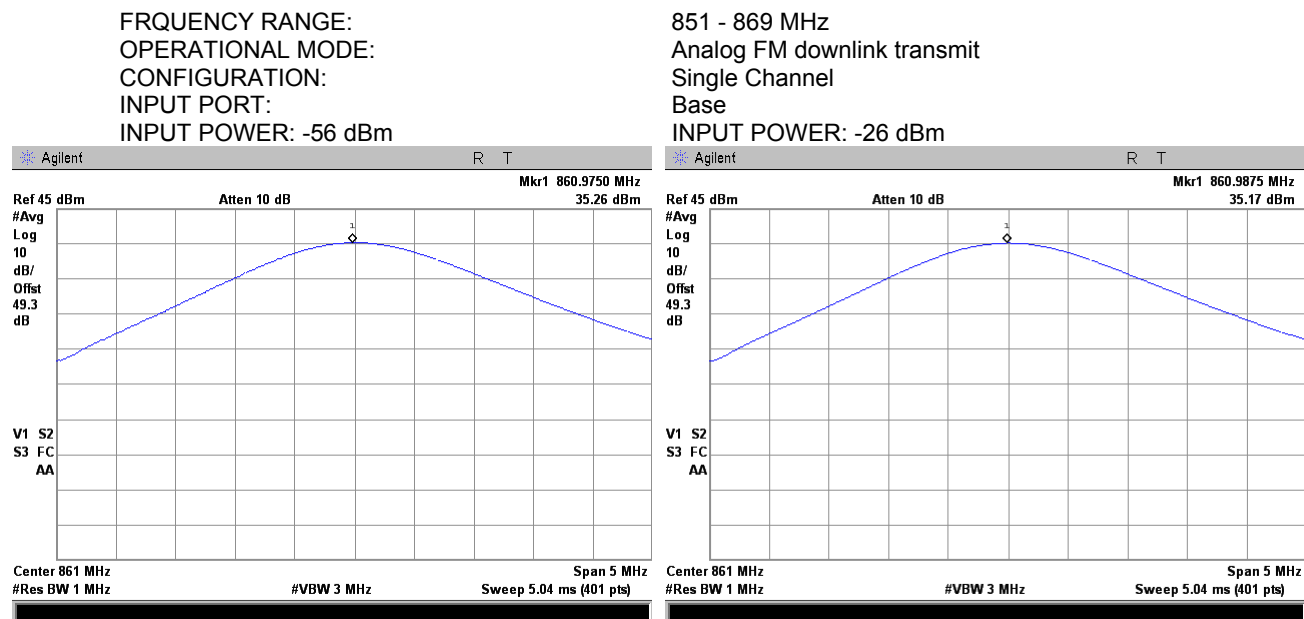
Plot 7.1.32 RF output power measurements at mid frequency carrier, Port 1
