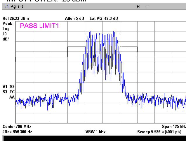
Plot 7.3.42 Emission mask test result at high frequency carrier, Port 2
