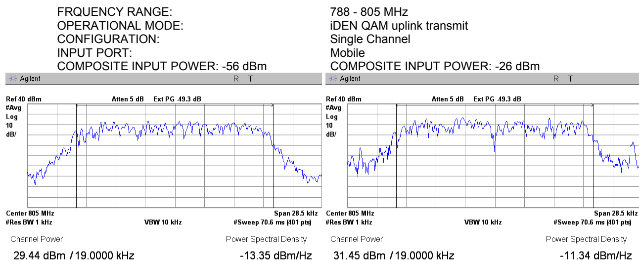
Plot 7.1.18 RF output power measurements at high frequency carrier, Port 2
