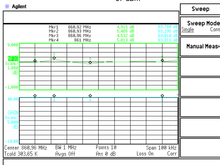
Plot 7.7.6 Noise figure test results at high frequency
