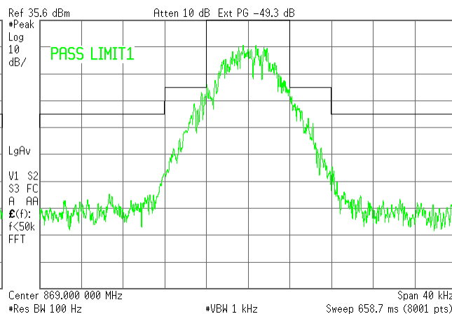
Plot 7.3.22 Emission mask test result at low frequency carrier, Port 2
