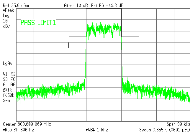
Plot 7.3.34 Emission mask test result at low frequency carrier, Port 2
