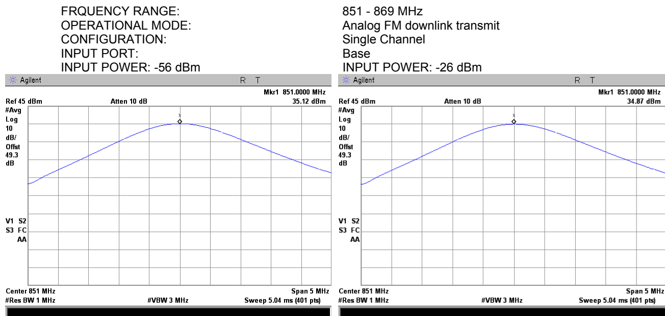
Plot 7.1.31 RF output power measurements at low frequency carrier, Port 1
