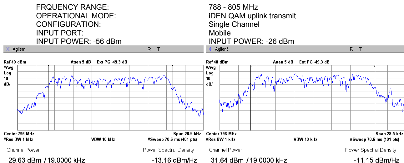
Plot 7.1.17 RF output power measurements at mid frequency carrier, Port 2
