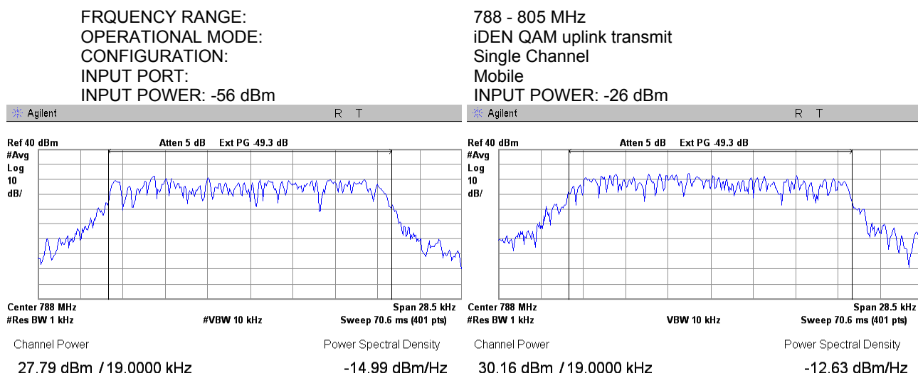
Plot 7.1.16 RF output power measurements at low frequency carrier, Port 2
