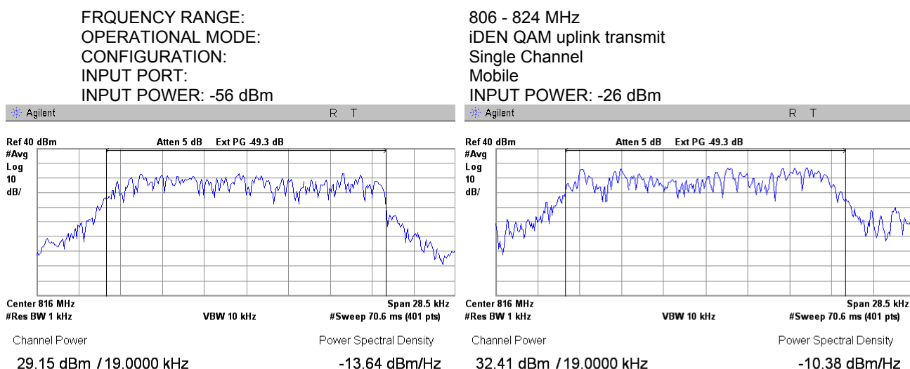
Plot 7.1.23 RF output power measurements at mid frequency carrier, Port 2
