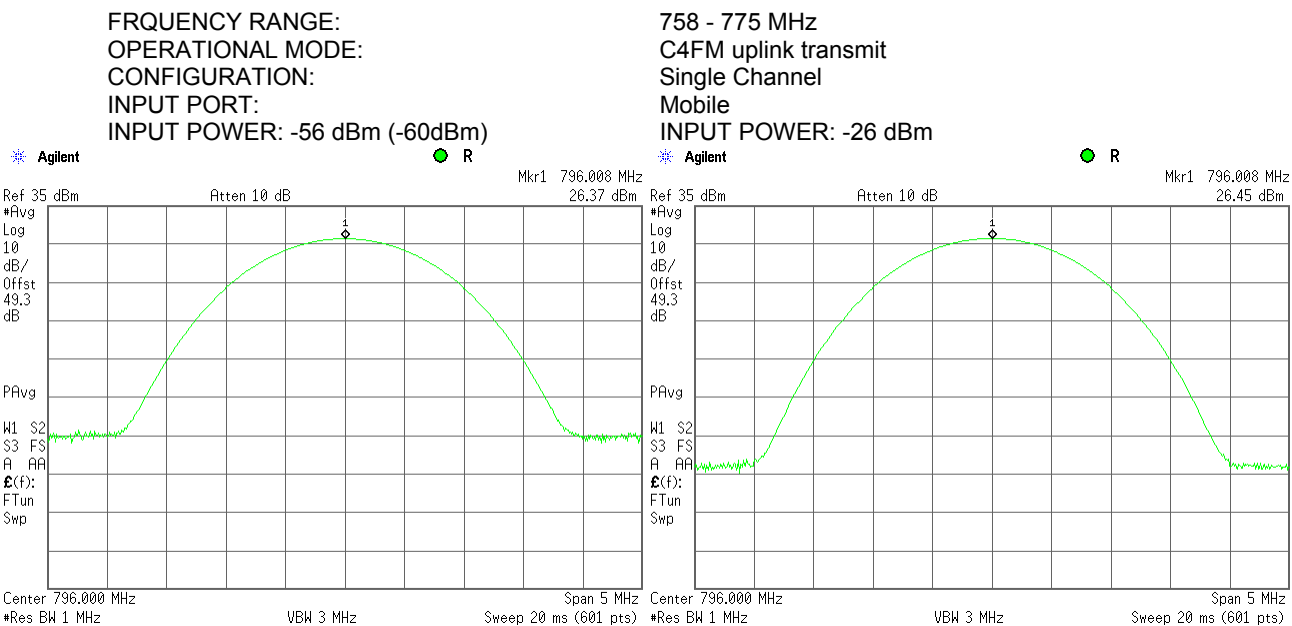
Plot 7.1.6 RF output power measurements at high frequency carrier, Port 2
