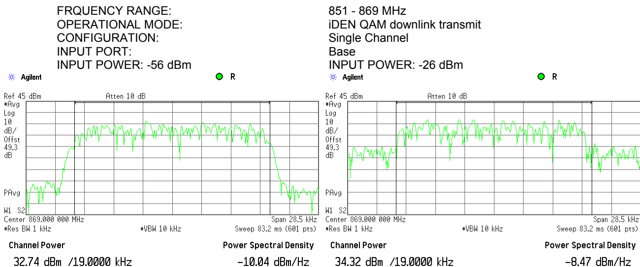
Plot 7.1.21 RF output power measurements at high frequency carrier, Port 1
