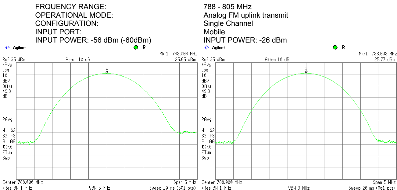
Plot 7.1.28 RF output power measurements at low frequency carrier, Port 2
