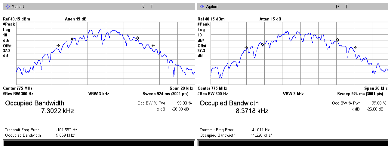
Plot 7.2.4 Occupied bandwidth test result at low frequency carrier, Port 2
