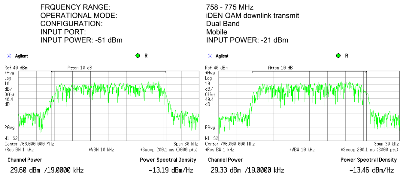
Plot 7.1.14 RF output power measurements at mid frequency carrier, Port 1
