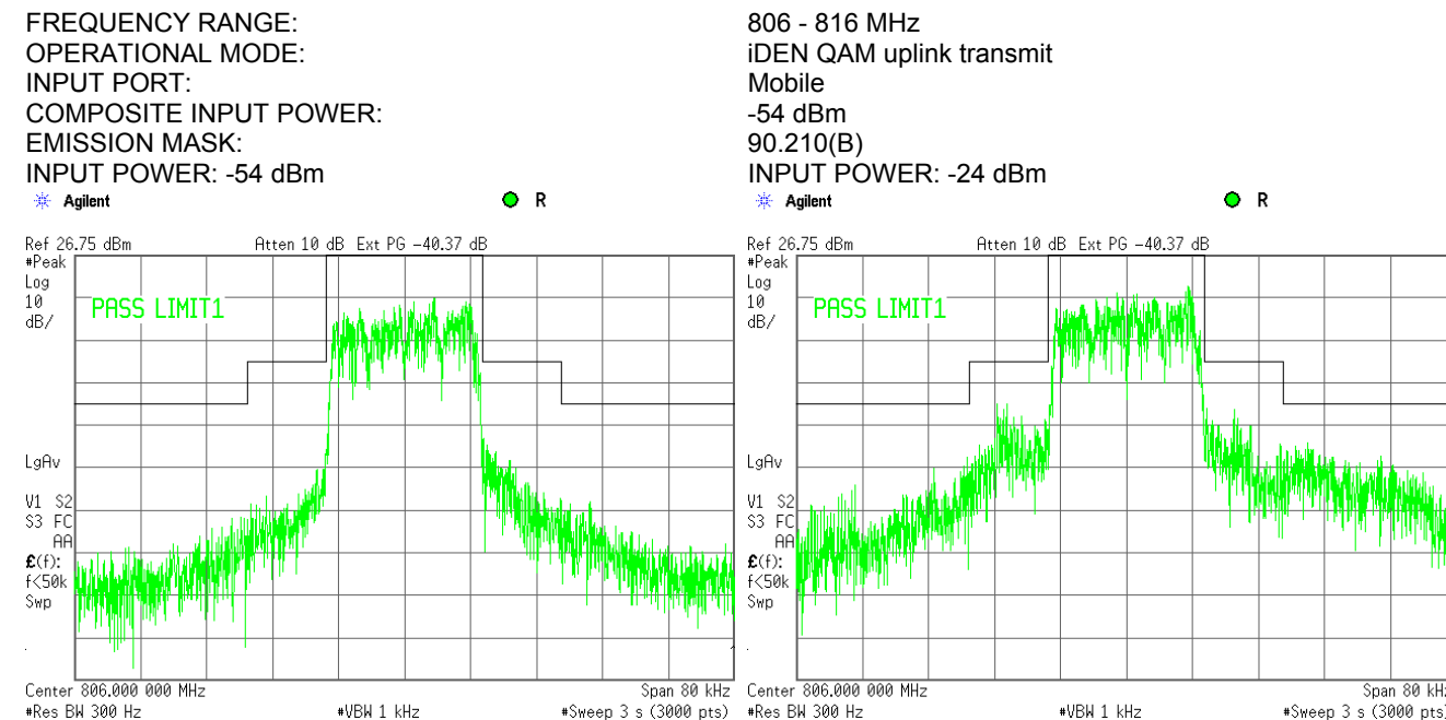
Plot 7.3.34 Emission mask test result at low frequency carrier, Port 2
