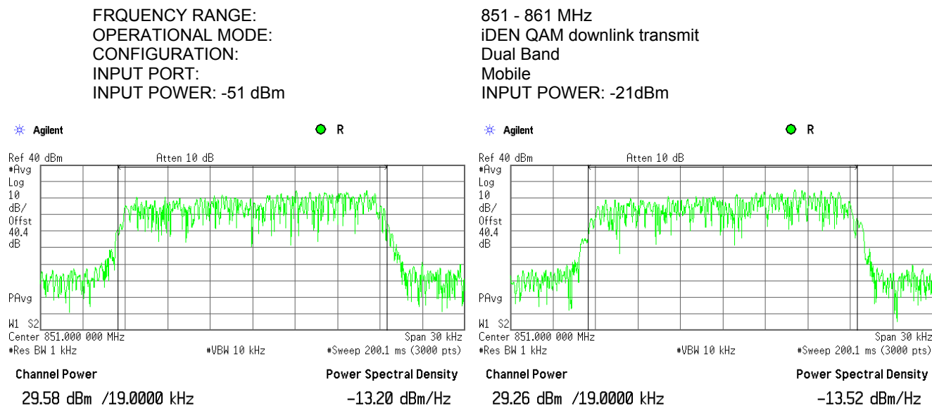
Plot 7.1.19 RF output power measurements at low frequency carrier, Port 1
