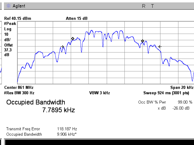
Plot 7.2.10 Occupied bandwidth test result at low frequency carrier, Port 2
