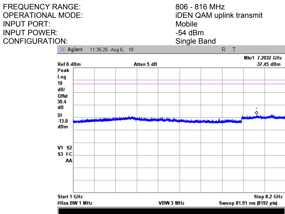
Plot 7.8.130 Spurious emission measurements in 1000 - 8200 MHz range at low carrier frequency
