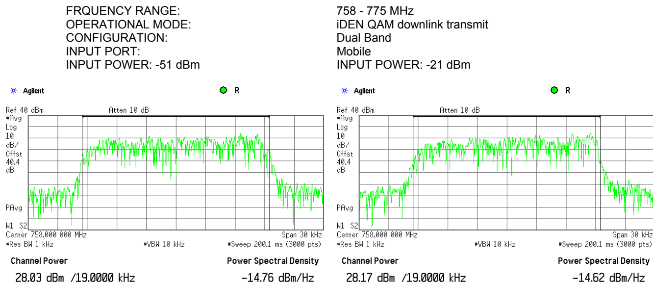
Plot 7.1.13 RF output power measurements at low frequency carrier, Port 1
