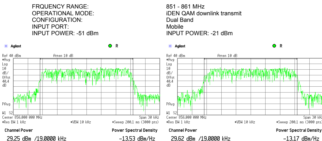
Plot 7.1.20 RF output power measurements at mid frequency carrier, Port 1
