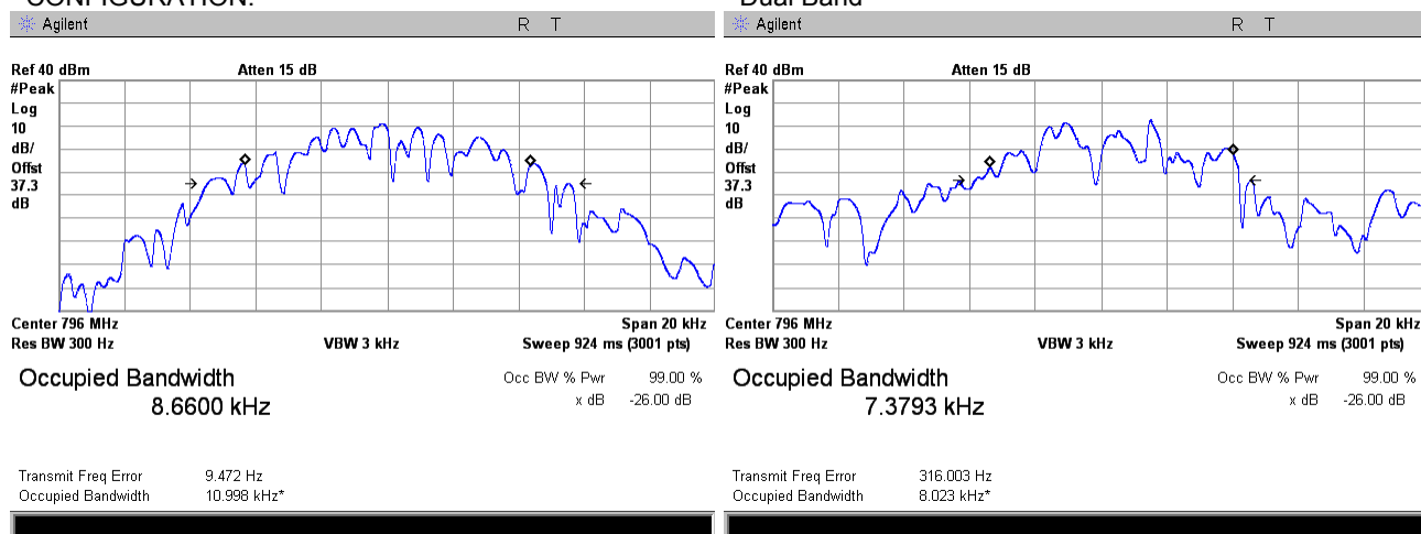
Plot 7.2.6 Occupied bandwidth test result at high frequency carrier, Port 2
