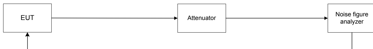
Figure 7.5.1 Emission mask test setup
