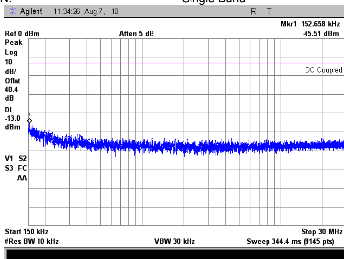
Plot 7.8.78 Spurious emission measurements in 0.15 – 30.0 MHz range at high carrier frequency
