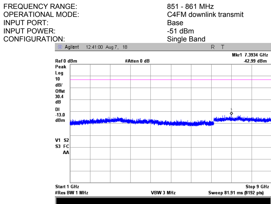
Plot 7.8.82 Spurious emission measurements in 1000 - 9000 MHz range at low carrier frequency
