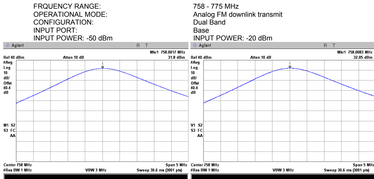
Plot 7.1.25 RF output power measurements at low frequency carrier, Port 1
