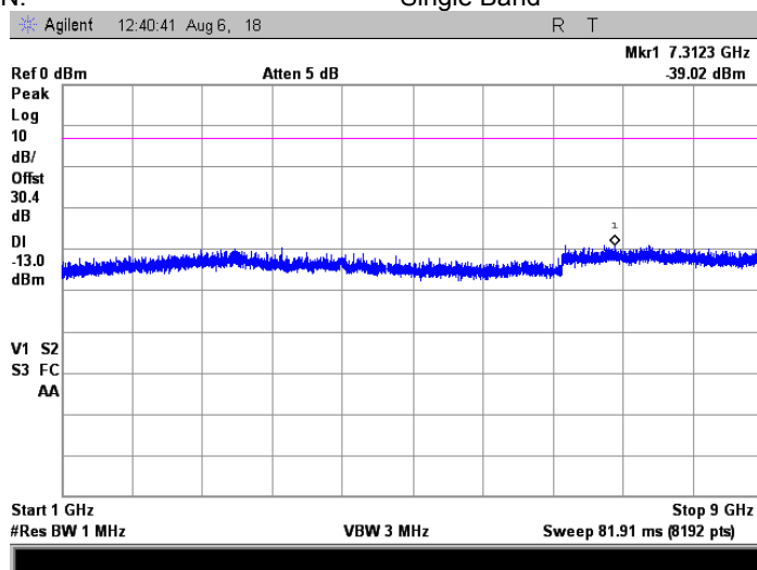
Plot 7.8.96 Spurious emission measurements in 1000 - 9000 MHz at high carrier frequency
