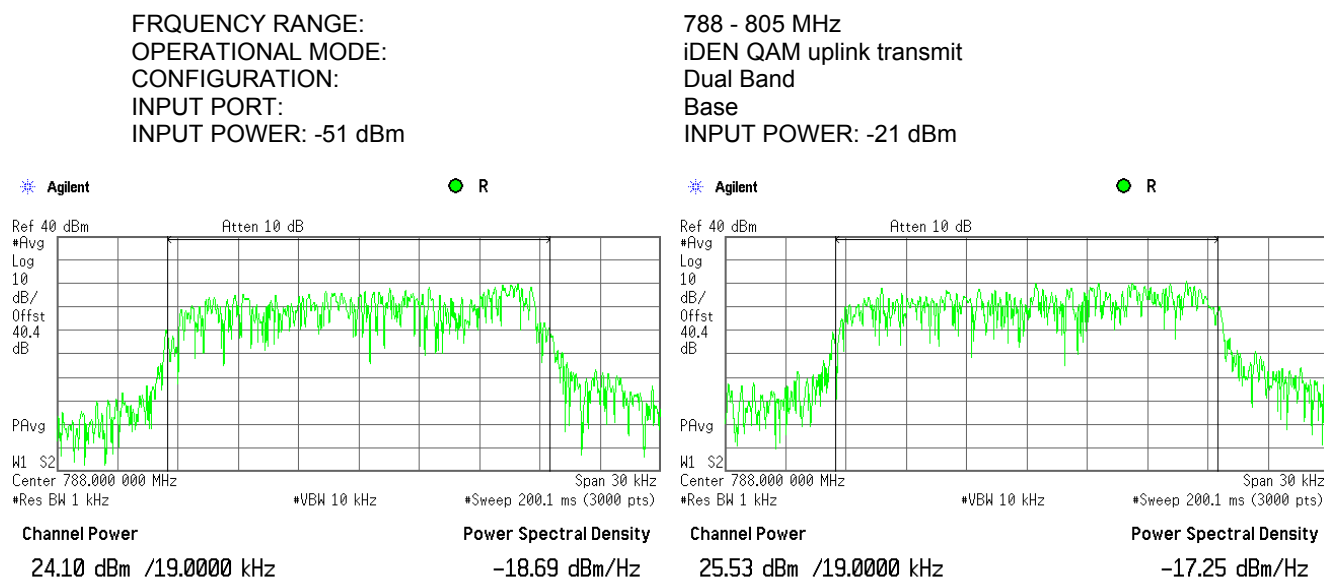
Plot 7.1.16 RF output power measurements at low frequency carrier, Port 2
