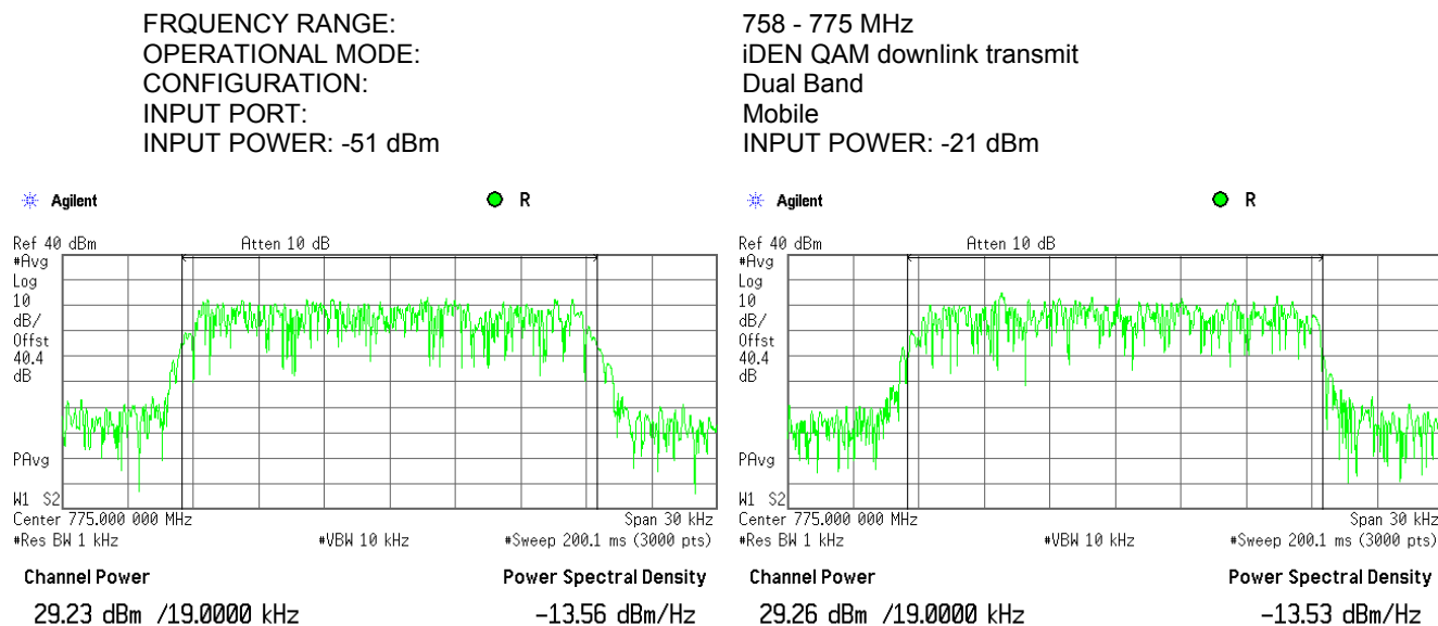
Plot 7.1.15 RF output power measurements at high frequency carrier, Port 1
