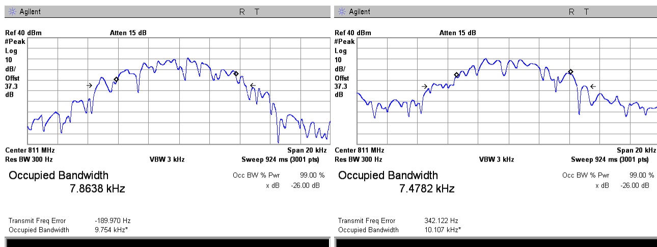
Plot 7.2.12 Occupied bandwidth test result at low frequency carrier, Port 2
