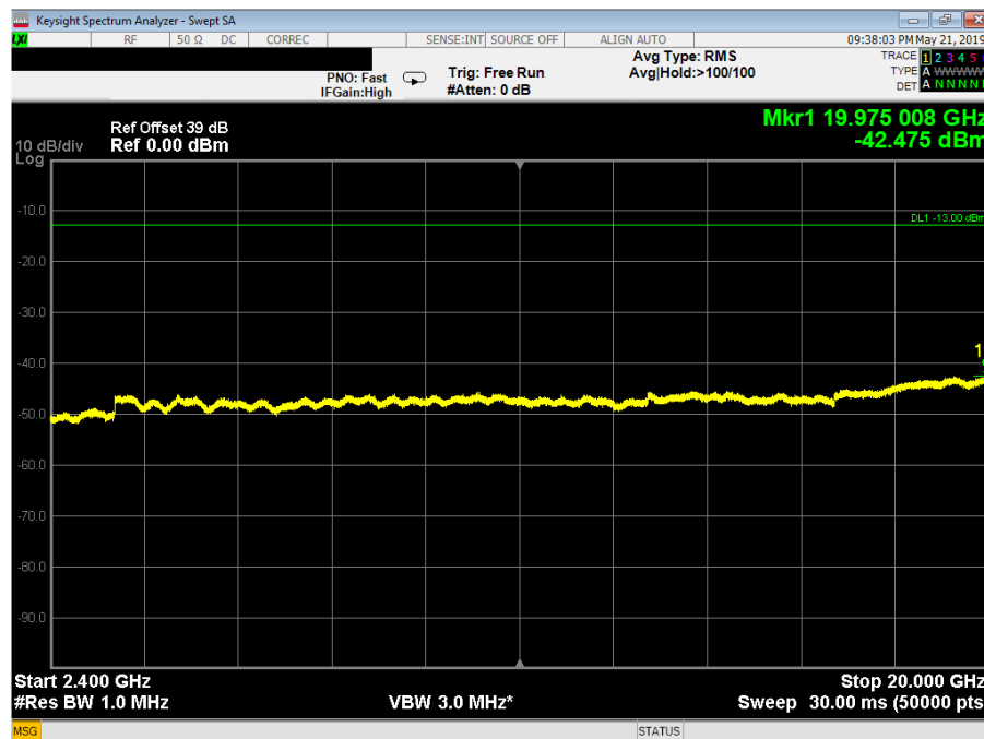
Plot 3.5.4: Spurious Emission Conducted Measurement, MSK Gaussian filter 0.3 data rate 270kbps, F_c = 1962.500, 2.4 \text{ GHz} - 20.0 \text{ GHz}
