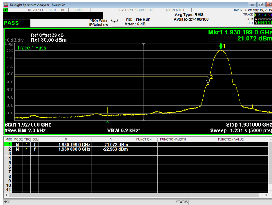
Plot 3.4.1: Band Edge test results, MSK Gaussian filter 0.3 data rate 270kbps, Fc = 1930.200 MHz, single test signal
