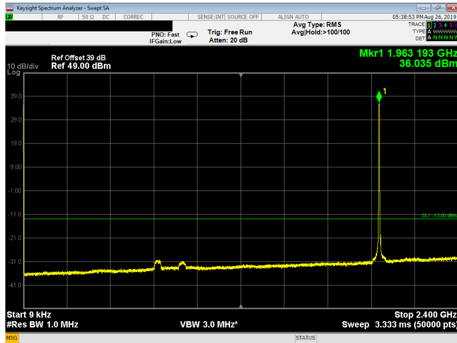
Plot 3.5.9: Spurious Emission Conducted Measurement, AWGN 4.1MHz, Fc = 1962.50 MHz, 9 kHz – 2.4 GHz
