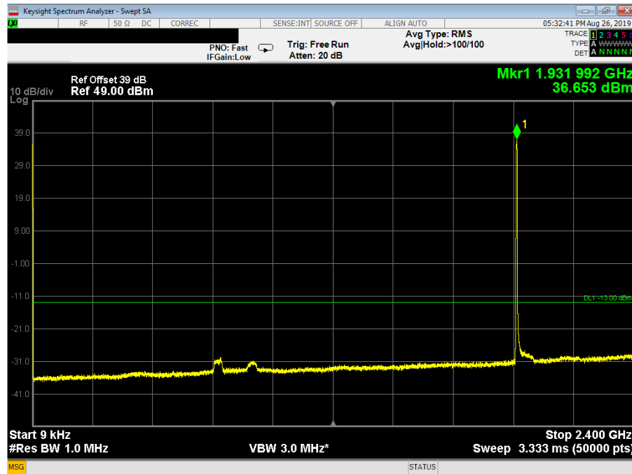
Plot 3.5.7: Spurious Emission Conducted Measurement, AWGN 4.1MHz, Fc = 1932.50 MHz, 9 kHz – 2.4 GHz
