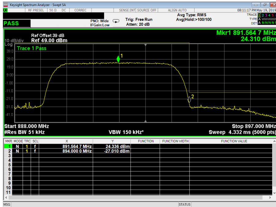
Plot 3.4.7: Band Edge test results, AWGN 4.1MHz, Fc = 891.500 MHz, single test signal
