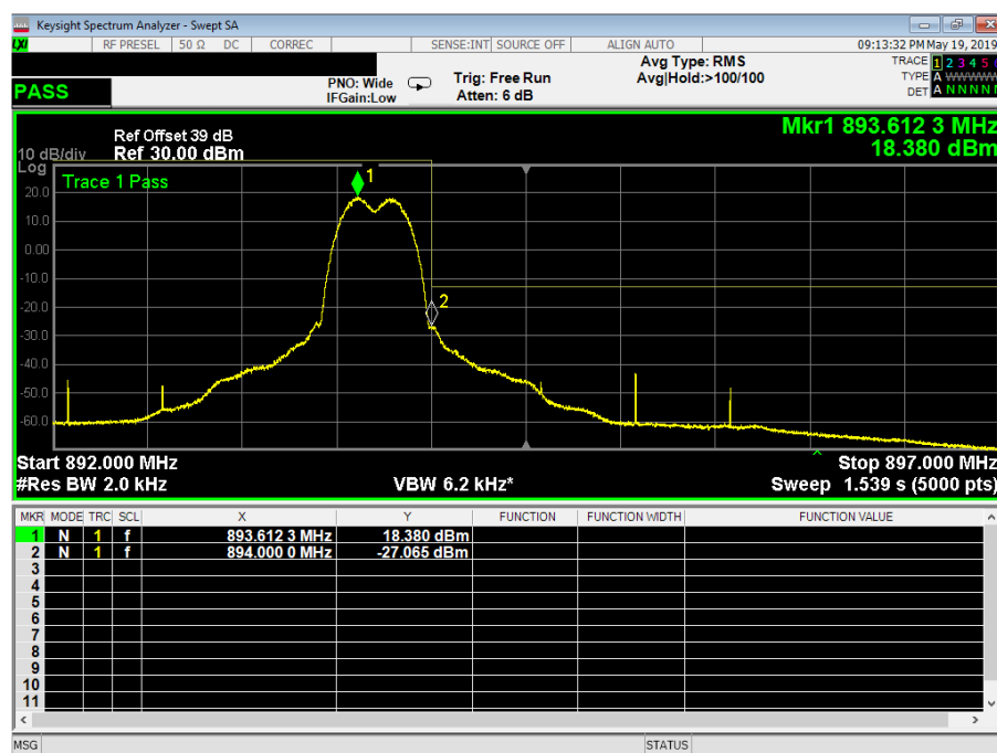
Plot 3.4.4: Band Edge test results, MSK Gaussian filter 0.3 data rate 270kbps, Fc = 893.600 + 893.800 MHz, two test signals
