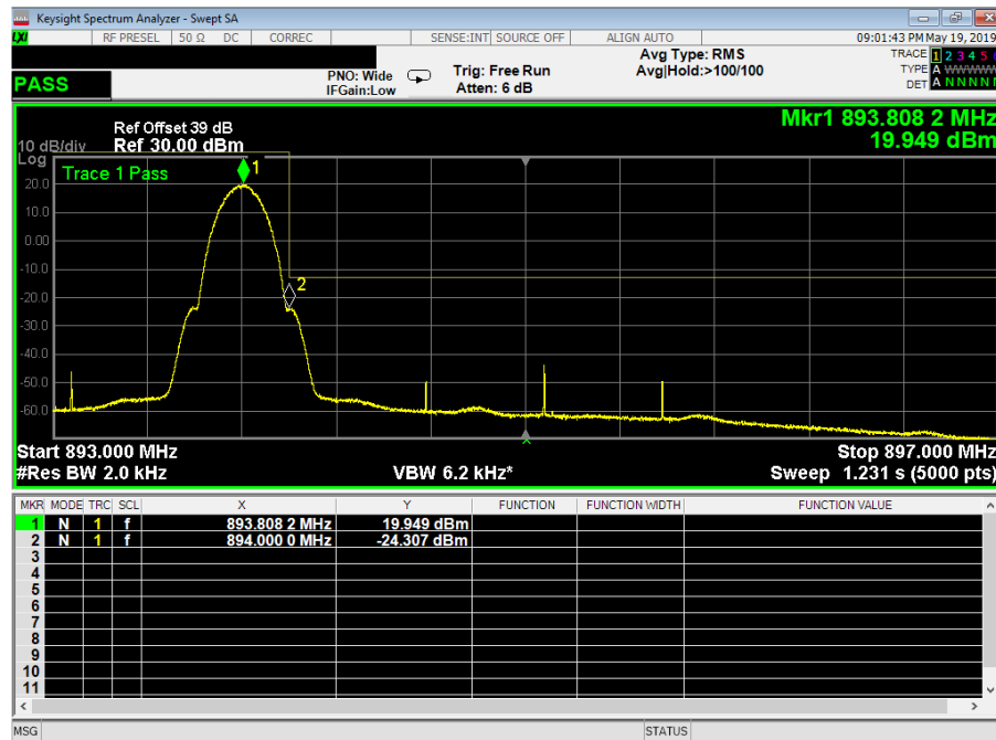
Plot 3.4.3: Band Edge test results, MSK Gaussian filter 0.3 data rate 270kbps, Fc = 893.800 MHz, single test signal
