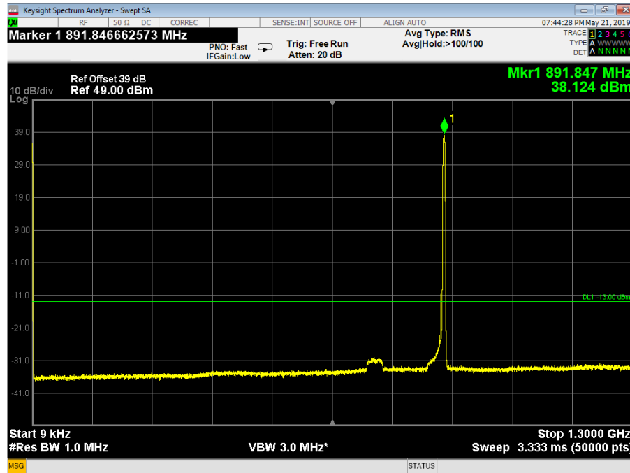
Plot 3.5.11: Spurious Emission Conducted Measurement, AWGN 4.1MHz, Fc = 891.500 MHz, 9 kHz – 1.3 GHz
