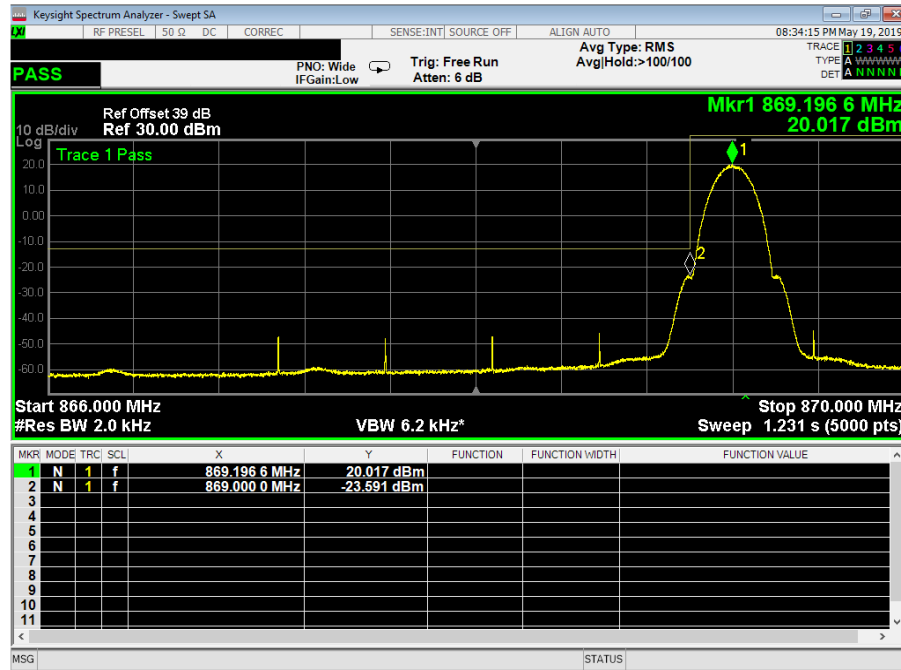
Plot 3.4.1: Band Edge test results, MSK Gaussian filter 0.3 data rate 270kbps, Fc = 869.200 MHz, single test signal
