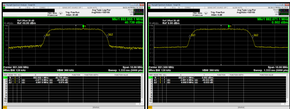
Plot 3.2.4: Input-versus-output signal comparison, AWGN 4.1MHz, 3 dB above AGC threshold level
