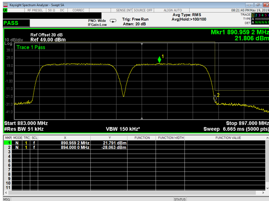
Plot 3.4.8: Band Edge test results, AWGN 4.1MHz, Fc = 886.500 + 891.500 MHz, two test signals
