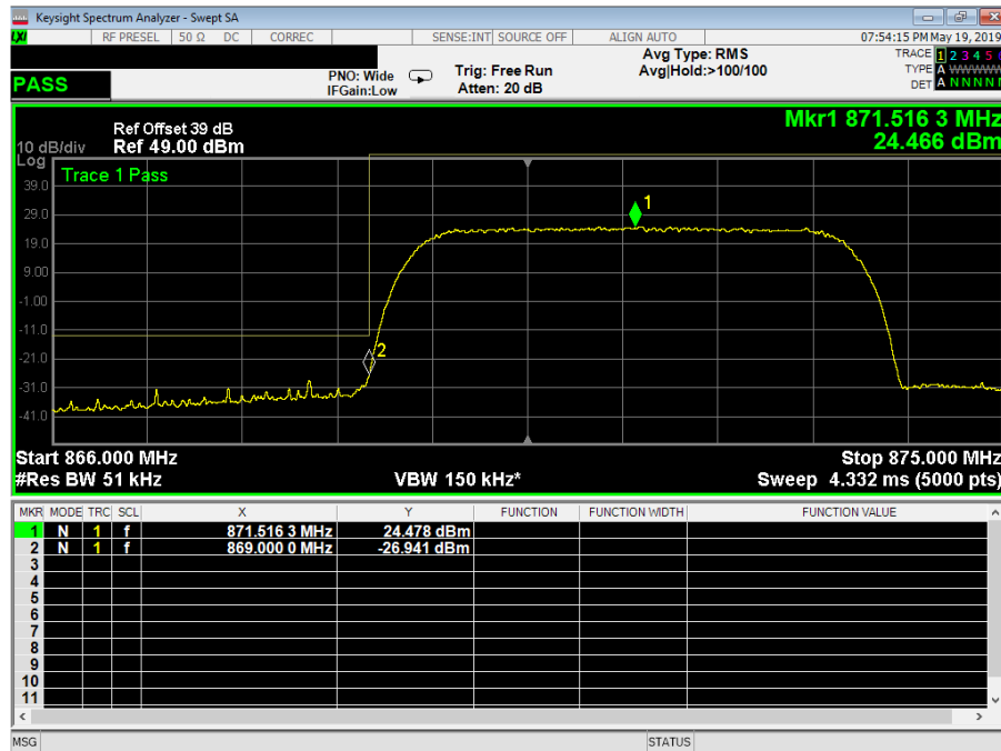
Plot 3.4.5: Band Edge test results, AWGN 4.1MHz, Fc = 871.500 MHz, single test signal
