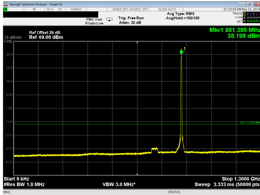
Plot 3.5.9: Spurious Emission Conducted Measurement, AWGN 4.1MHz, Fc = 881.500 MHz, 9 kHz – 1.3 GHz
